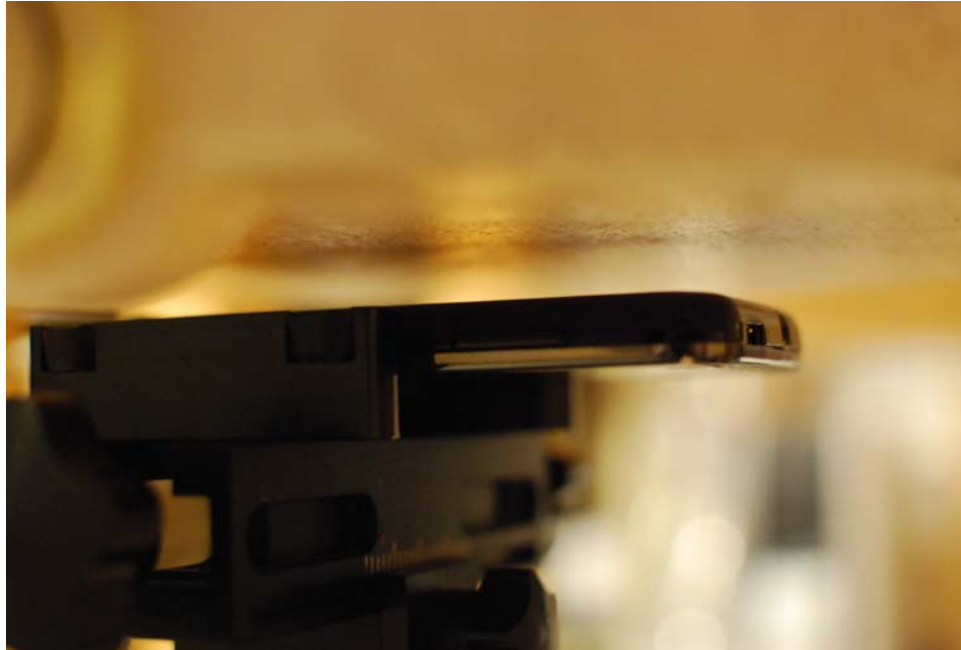
Figure 21-5 SAR Test Setup Photo 5: Back and 1.0 cm
