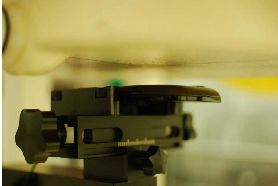
Figure 20-5 SAR Test Setup Photo 4
