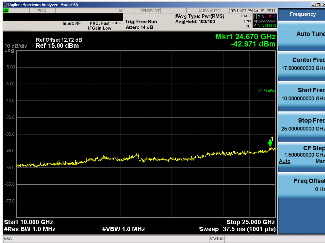
Plot 6-21. Conducted Spurious Plot (Bluetooth, 2Mbps – Ch. 39)
