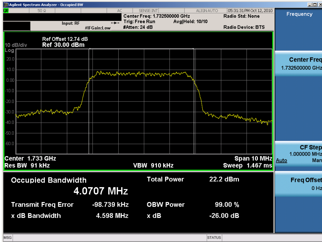
Plot 7-31. Occupied Bandwidth Plot (AWS WCDMA Mode – Ch. 1412)
