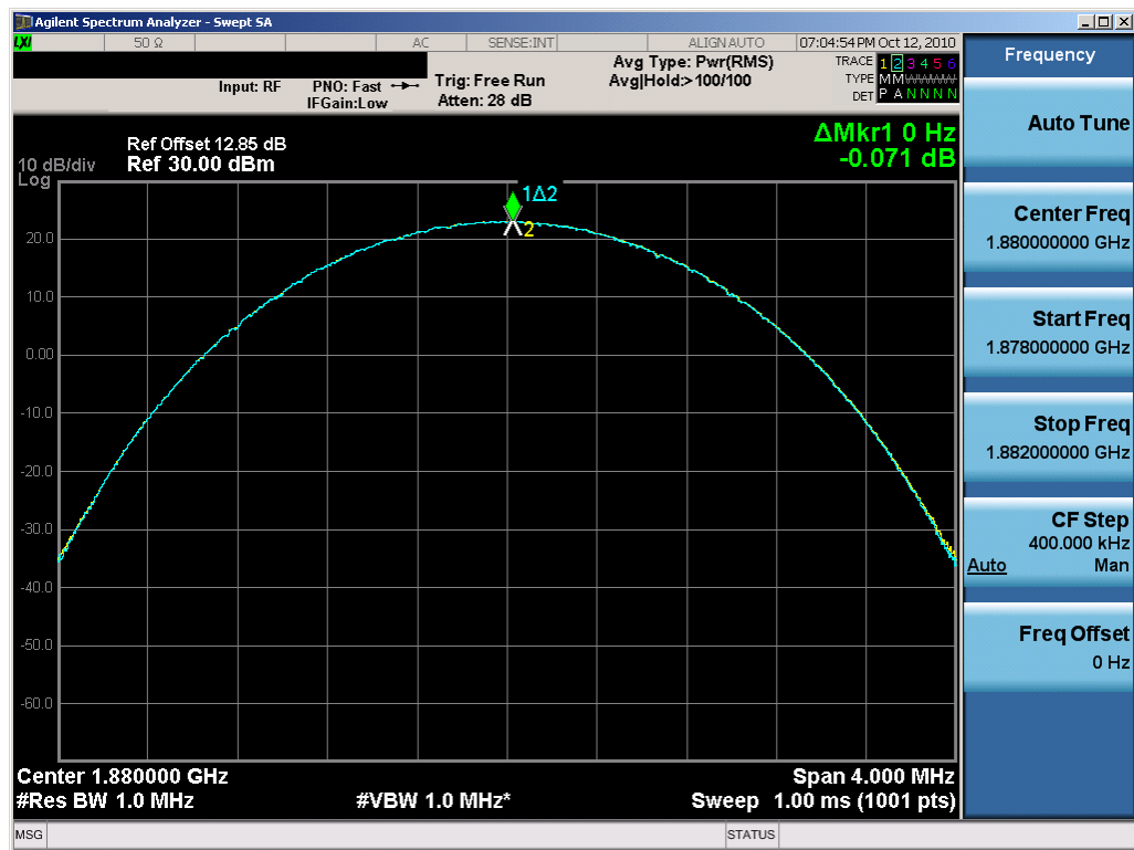
Plot 7-24. Peak-Average Ratio Plot (EDGE1900 Mode – Ch. 661)
