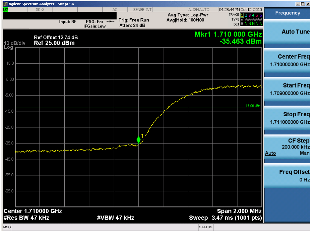
Plot 7-27. Band Edge Plot (AWS WCDMA Mode – Ch. 1312)
