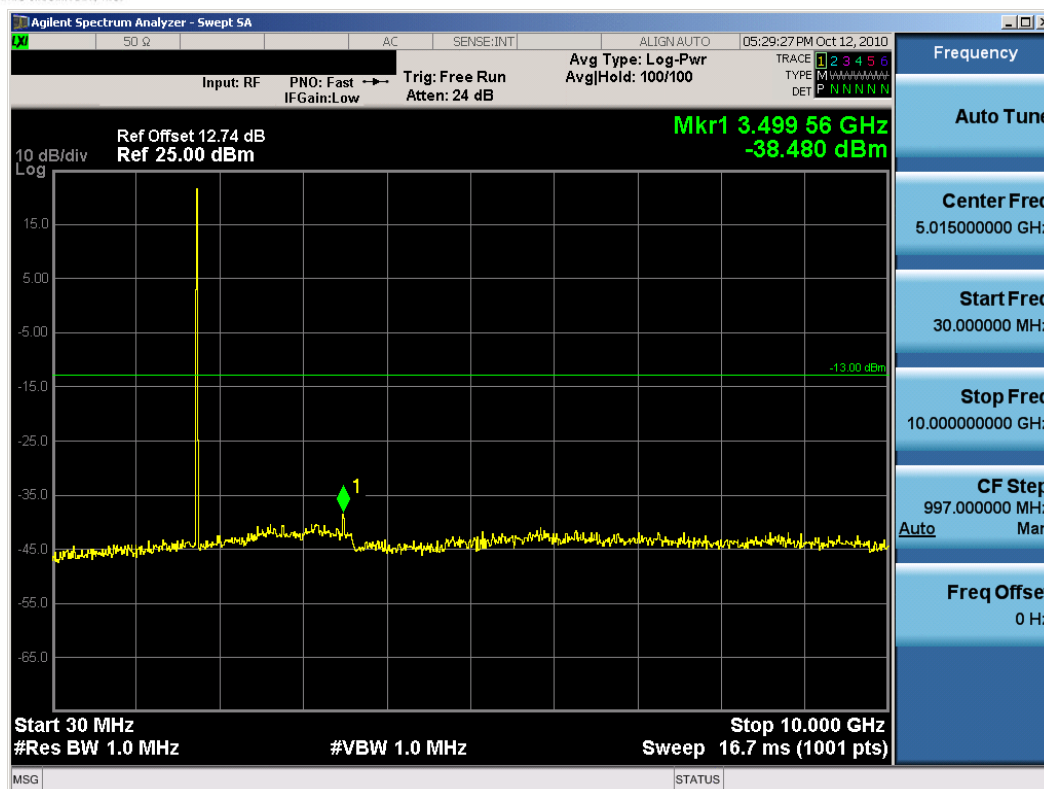
Plot 7-33. Conducted Spurious Plot (AWS WCDMA Mode – Ch. 1862)
