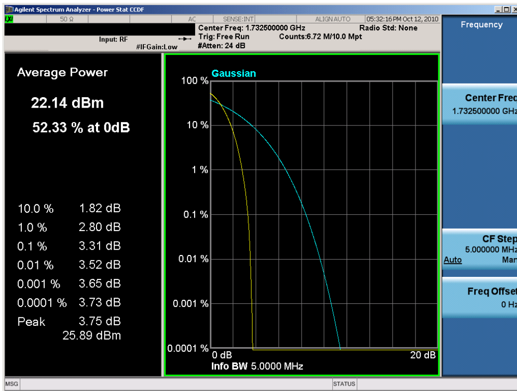
Plot 7-32. Peak-Average Ratio Plot (AWS WCDMA Mode – Ch. 1412)
