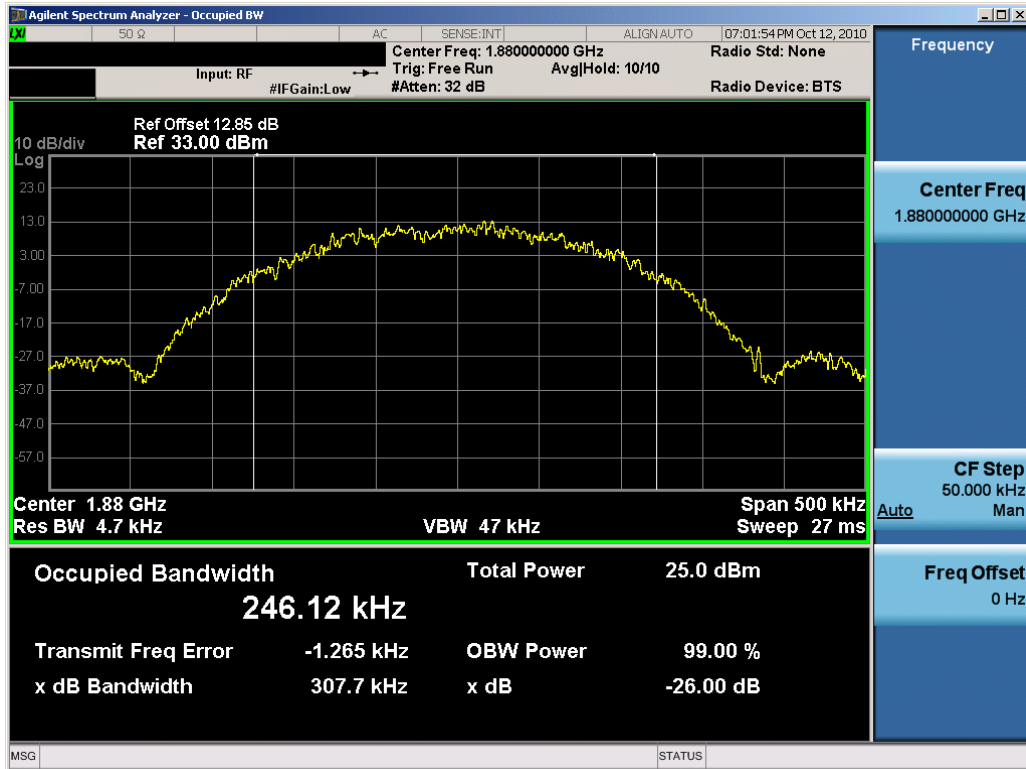
Plot 7-23. Occupied Bandwidth Plot (EDGE1900 Mode – Ch. 661)
