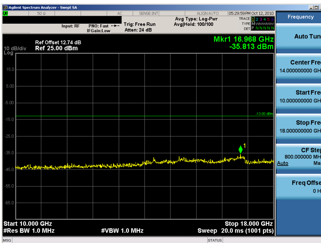
Plot 7-34. Conducted Spurious Plot (AWS WCDMA Mode – Ch. 1862)
