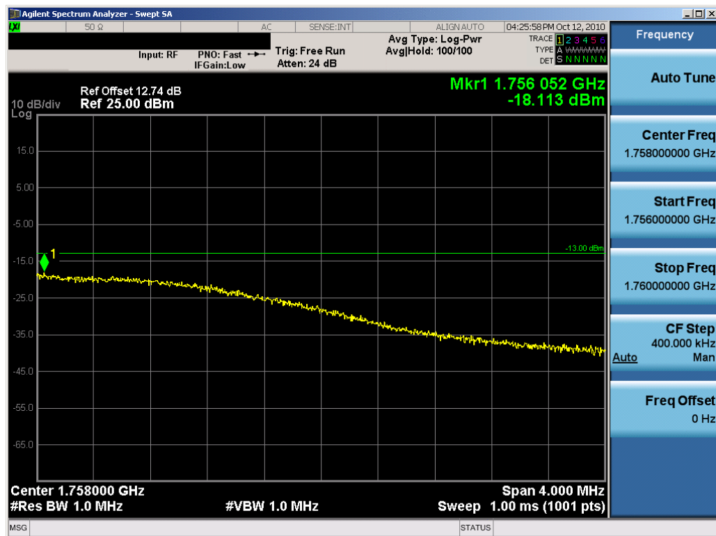
Plot 7-36. 4MHz Span Plot (AWS WCDMA Mode – Ch. 1862)
