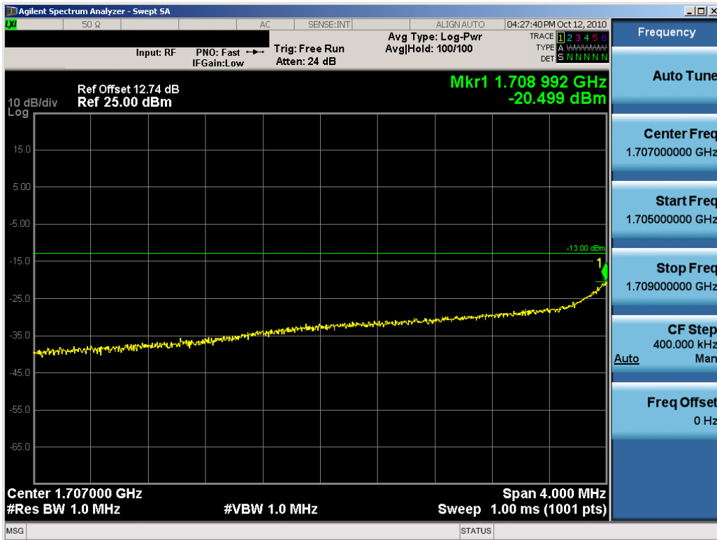
Plot 7-28. 4MHz Span Plot (AWS WCDMA Mode – Ch. 1312)
