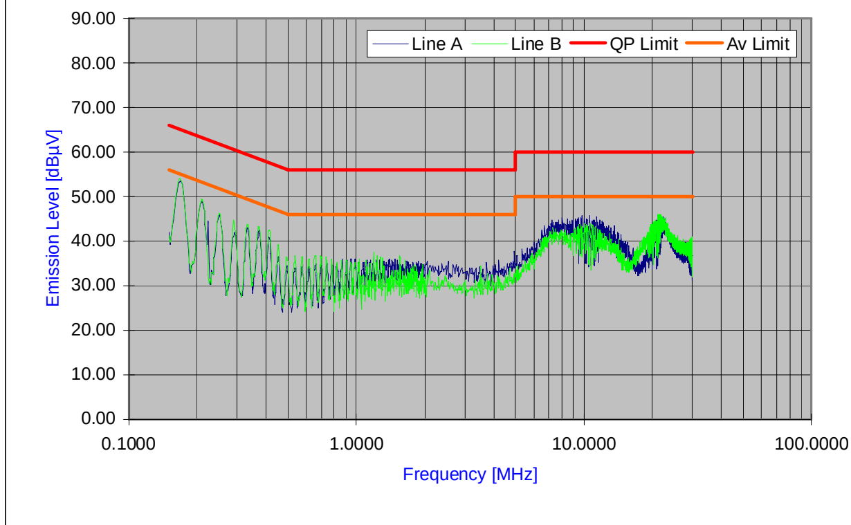
Plot 6-32. Line Conducted Plot with 802.11g
