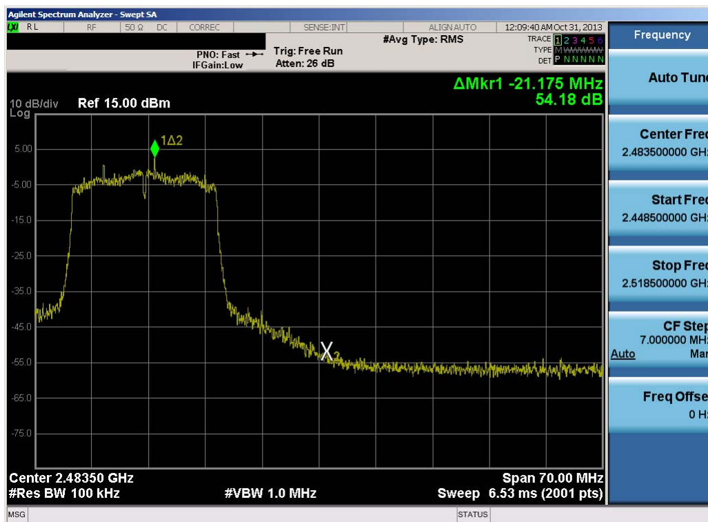
Plot 6-24. Band Edge Plot (802.11n (2.4GHz) – Ch. 11)
