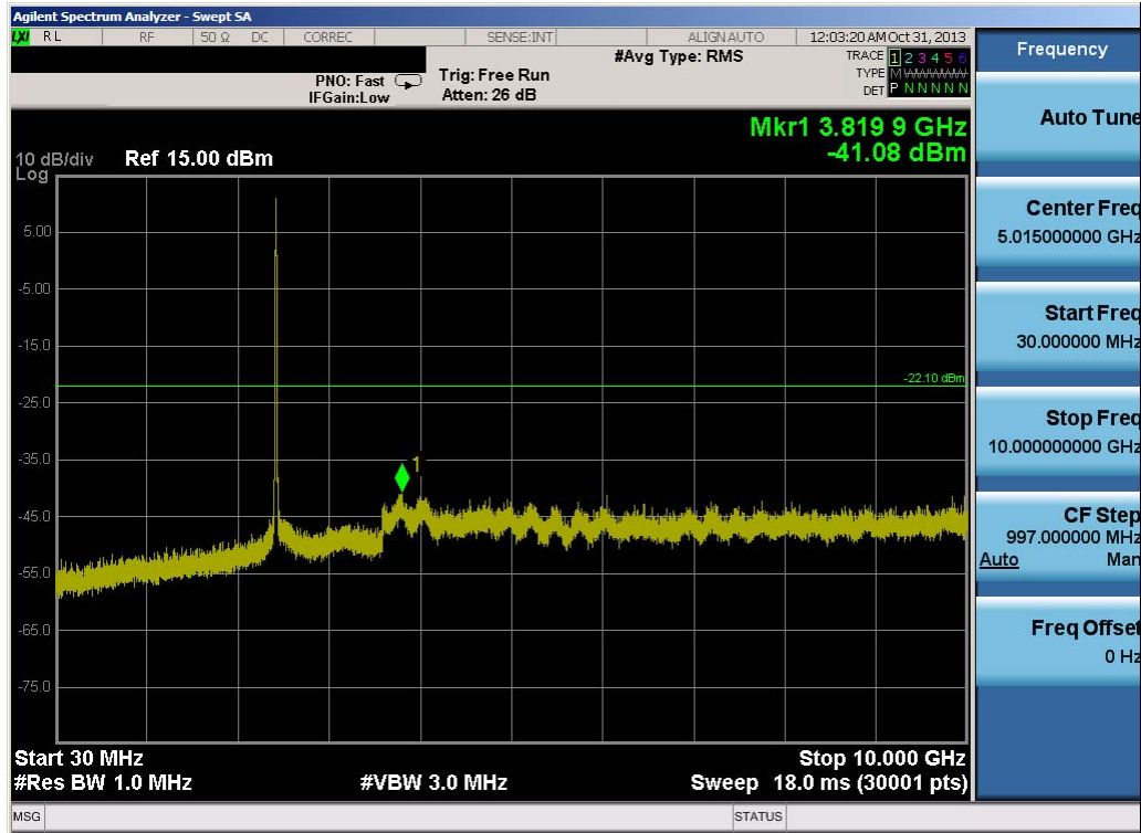
Plot 6-27. Conducted Spurious Plot (802.11b – Ch. 6)
