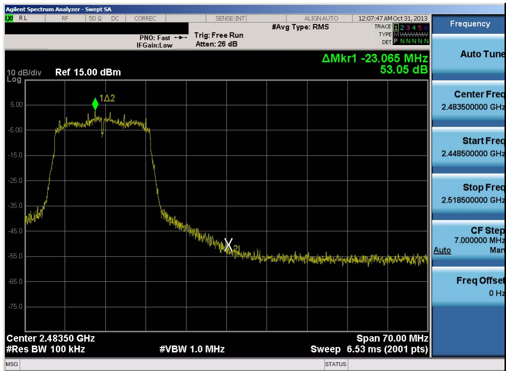
Plot 6-22. Band Edge Plot (802.11g – Ch. 11)
