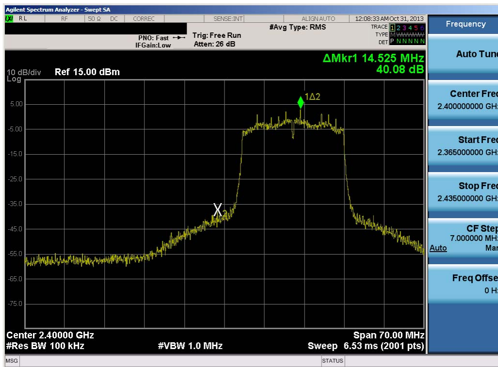
Plot 6-23. Band Edge Plot (802.11n (2.4GHz) – Ch. 1)
