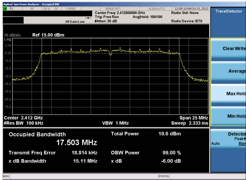
Plot 6-7. 6dB Bandwidth Plot (802.11n (2.4GHz) – Ch. 1)
