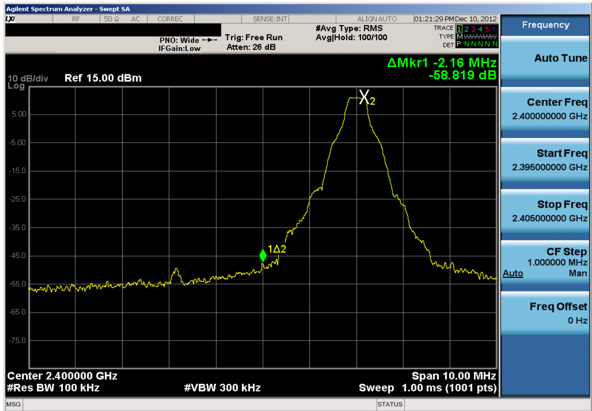
Plot 6-28. Band Edge Plot (Bluetooth with Hopping Disabled, 1Mbps – Ch. 0)
