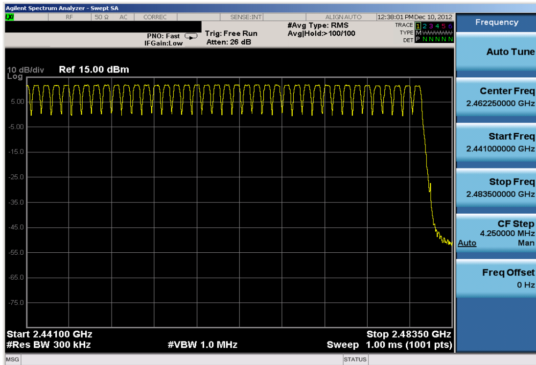
Plot 6-35. High End Spectrum Channel Hopping Plot (Bluetooth)
