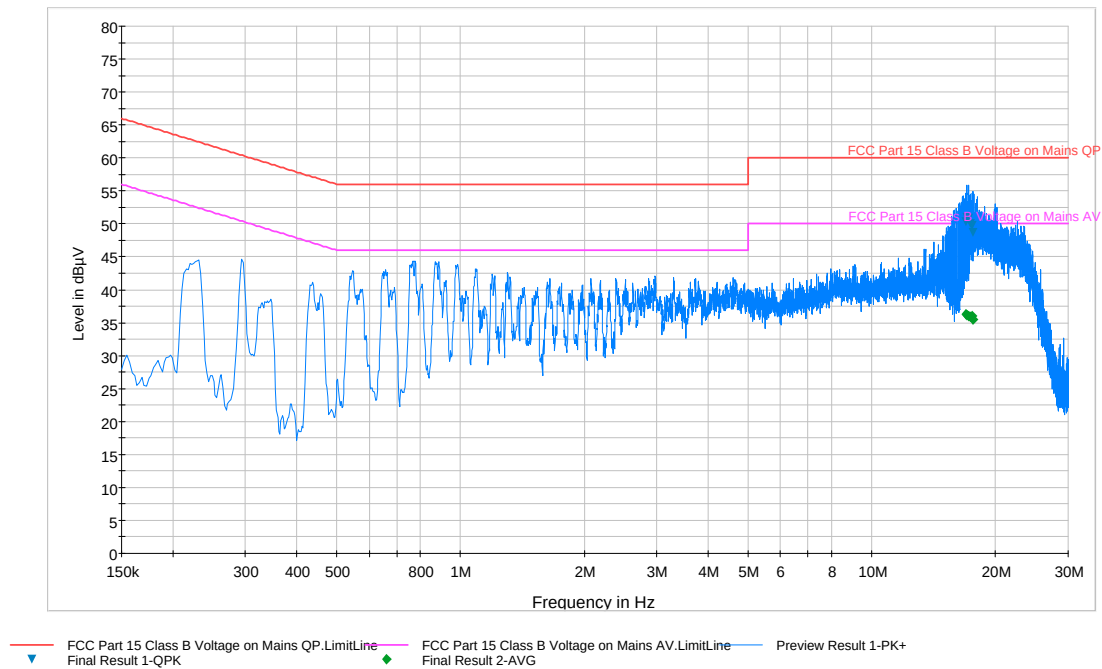
Plot 6-43. Line-Conducted Test Plot (N)
