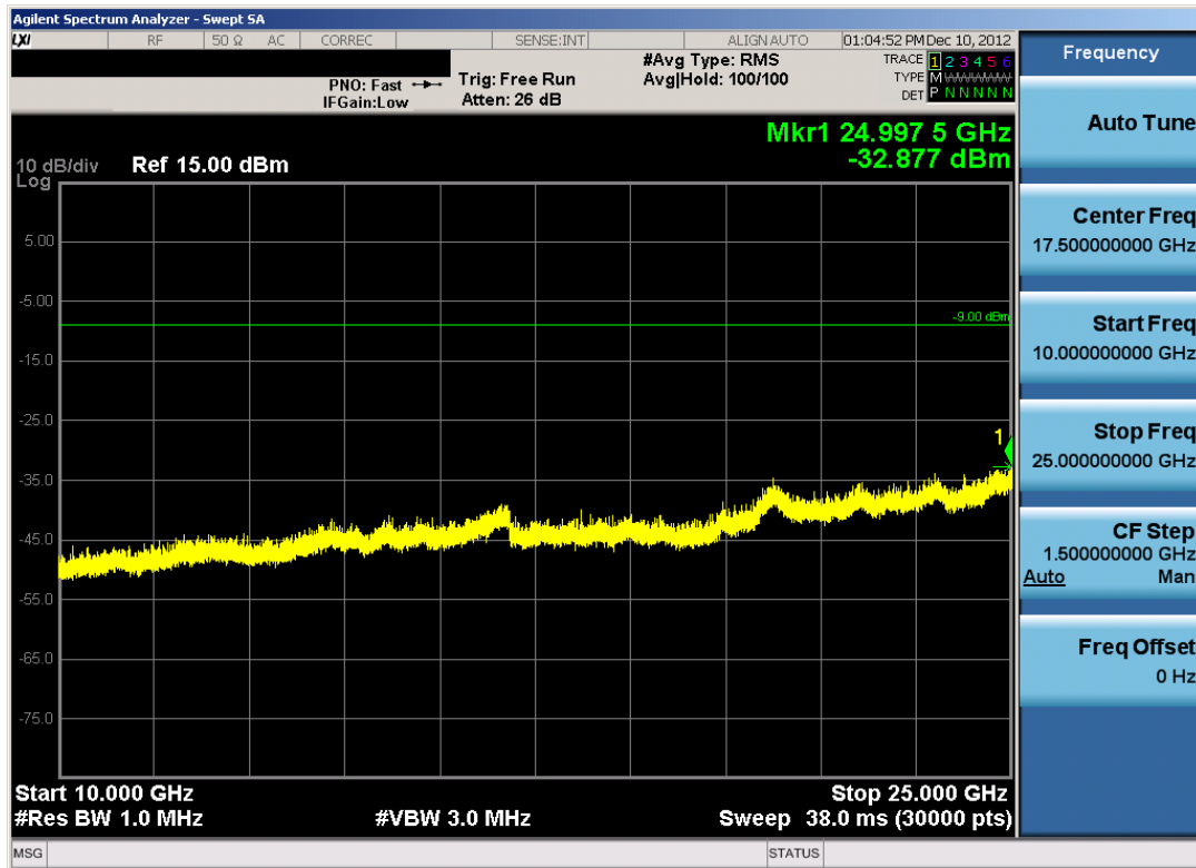
Plot 6-41. Conducted Spurious Plot (Bluetooth, 1Mbps – Ch. 78)
