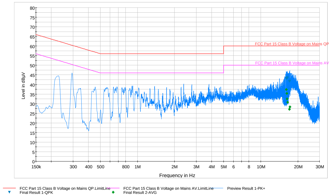
Plot 6-42. Line-Conducted Test Plot (L1)
