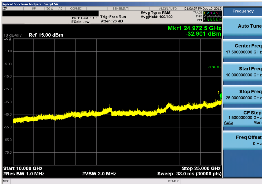
Plot 6-37. Conducted Spurious Plot (Bluetooth, 1Mbps – Ch. 0)
