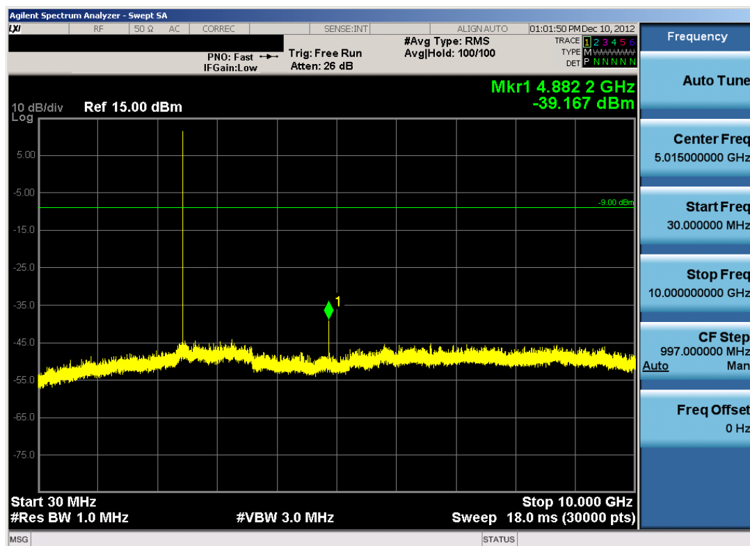
Plot 6-38. Conducted Spurious Plot (Bluetooth, 1Mbps – Ch. 39)
