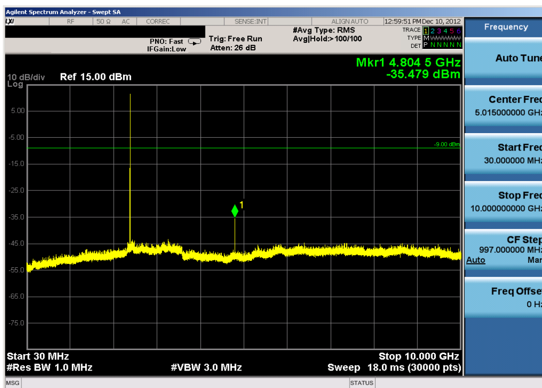
Plot 6-36. Conducted Spurious Plot (Bluetooth, 1Mbps – Ch. 0)
