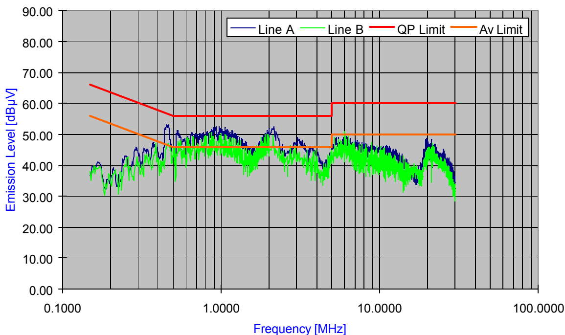
Plot 6-56. Line Conducted Plot with 802.11n
