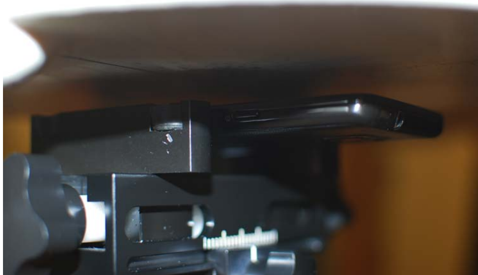
SAR Test Setup Photo 6: Front at 1.0 cm
