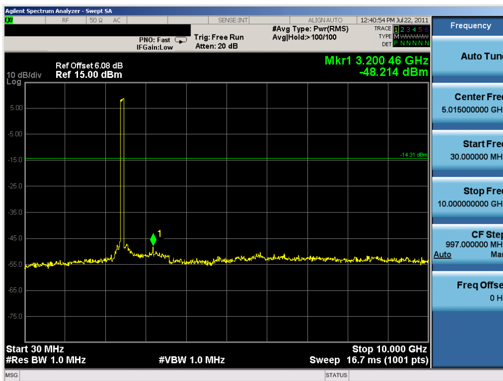
Plot 6-18. Conducted Spurious Plot (Bluetooth, 1Mbps – Ch. 0)
