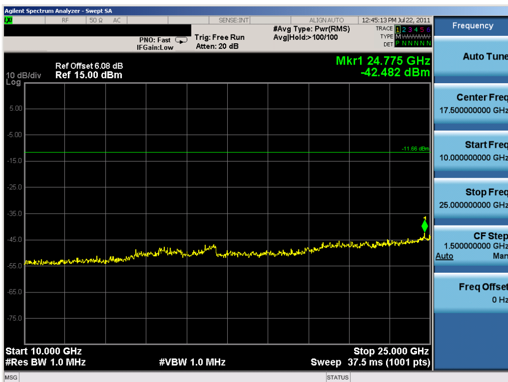
Plot 6-22. Conducted Spurious Plot (Bluetooth, 1Mbps – Ch. 39)
