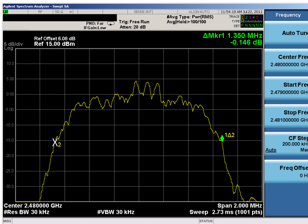
Plot 6-6. 20dB Bandwidth Plot (Bluetooth, 2Mbps – Ch. 78)
