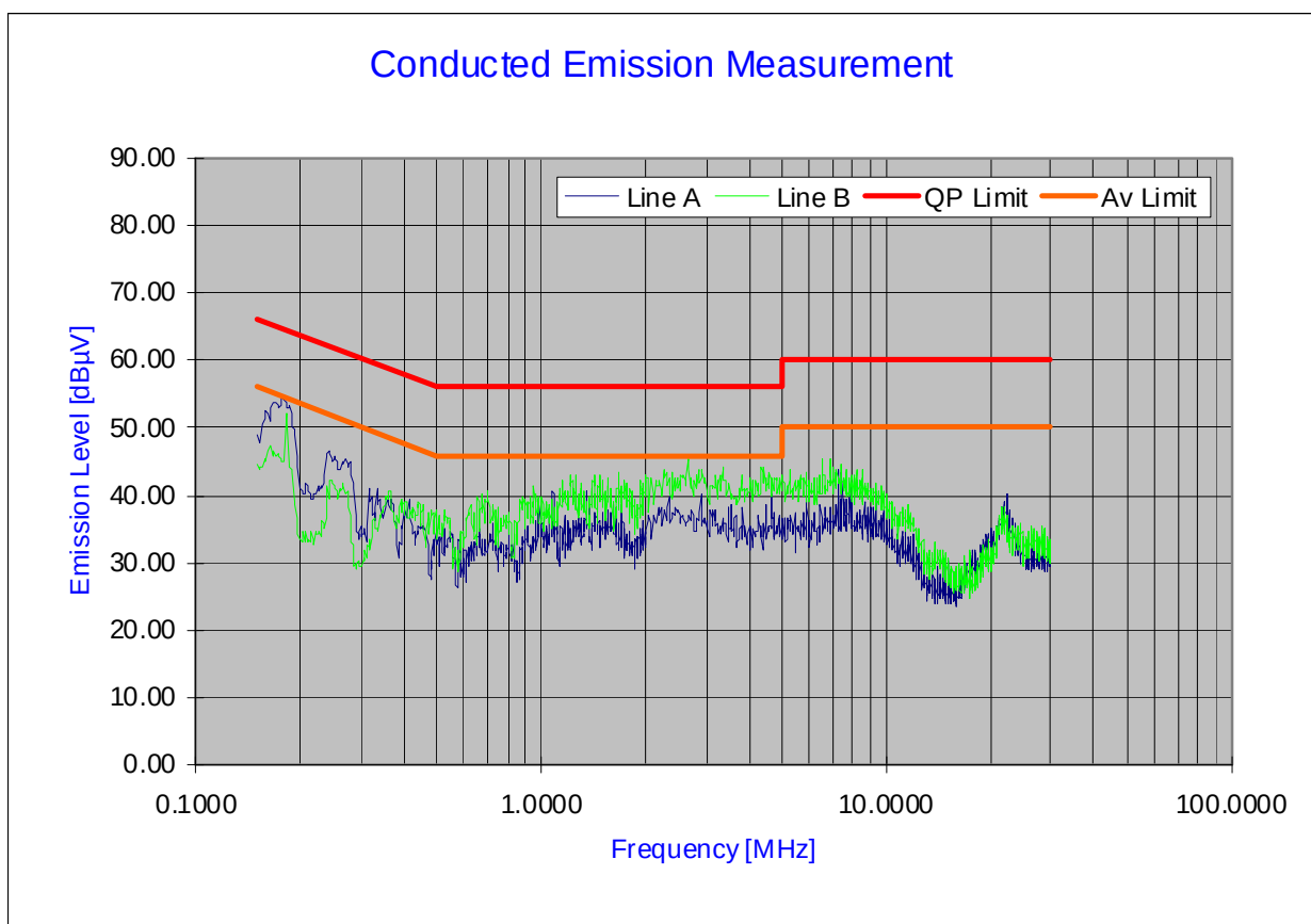
Plot 6-25. Line Conducted Plot with Bluetooth
