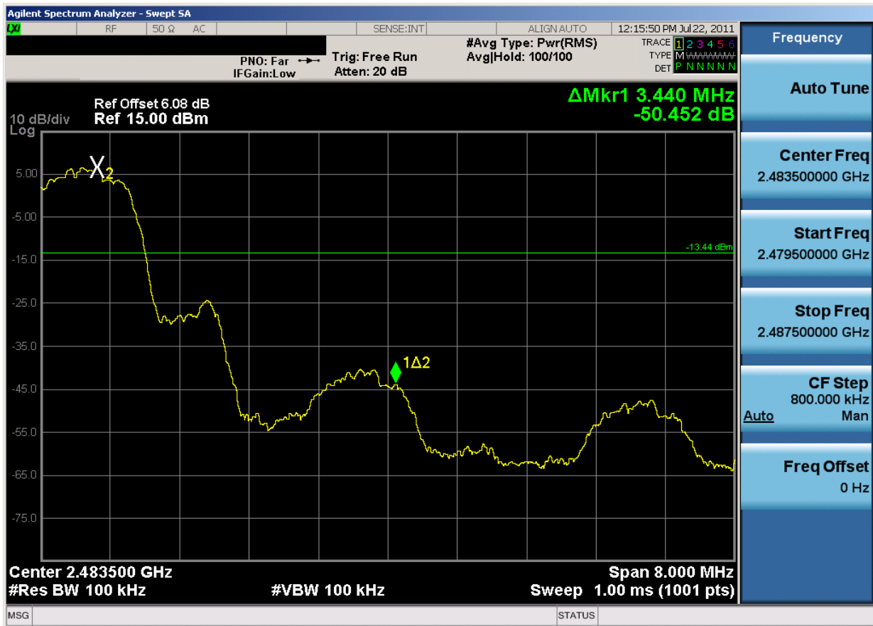
Plot 6-13. Band Edge Plot (Bluetooth, 3Mbps – Ch. 78)
