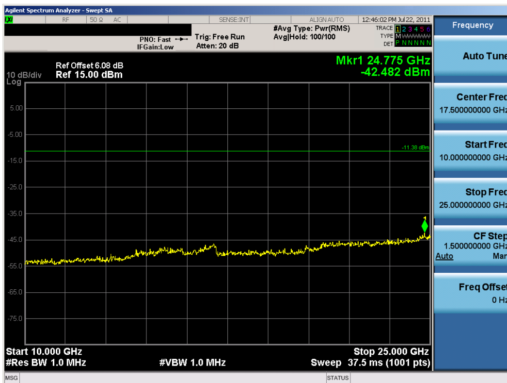
Plot 6-24. Conducted Spurious Plot (Bluetooth, 1Mbps – Ch. 78)
