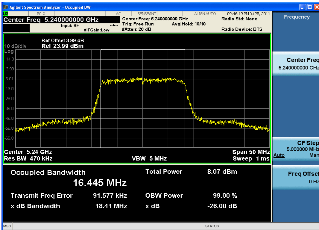
Plot 6-3. 26dB Bandwidth Plot (802.11a (UNII Band 1) – Ch. 48)
