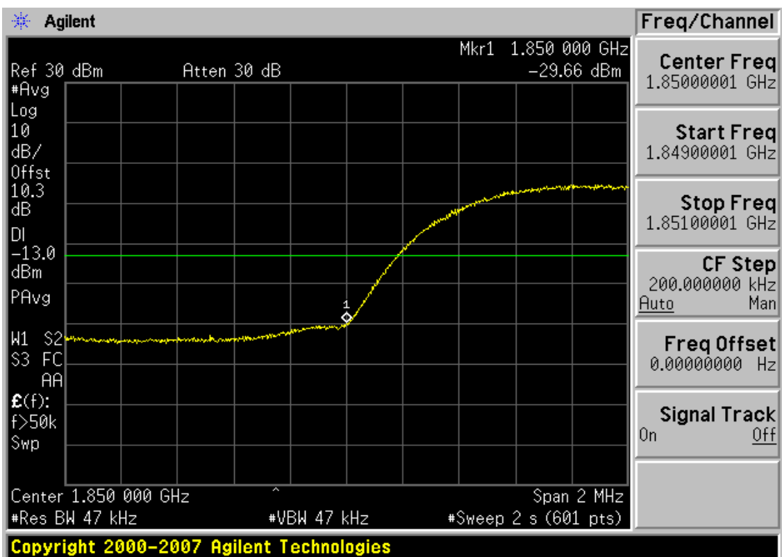
Plot 7-38. Band Edge Plot (PCS WCDMA Mode – Ch. 9262)
