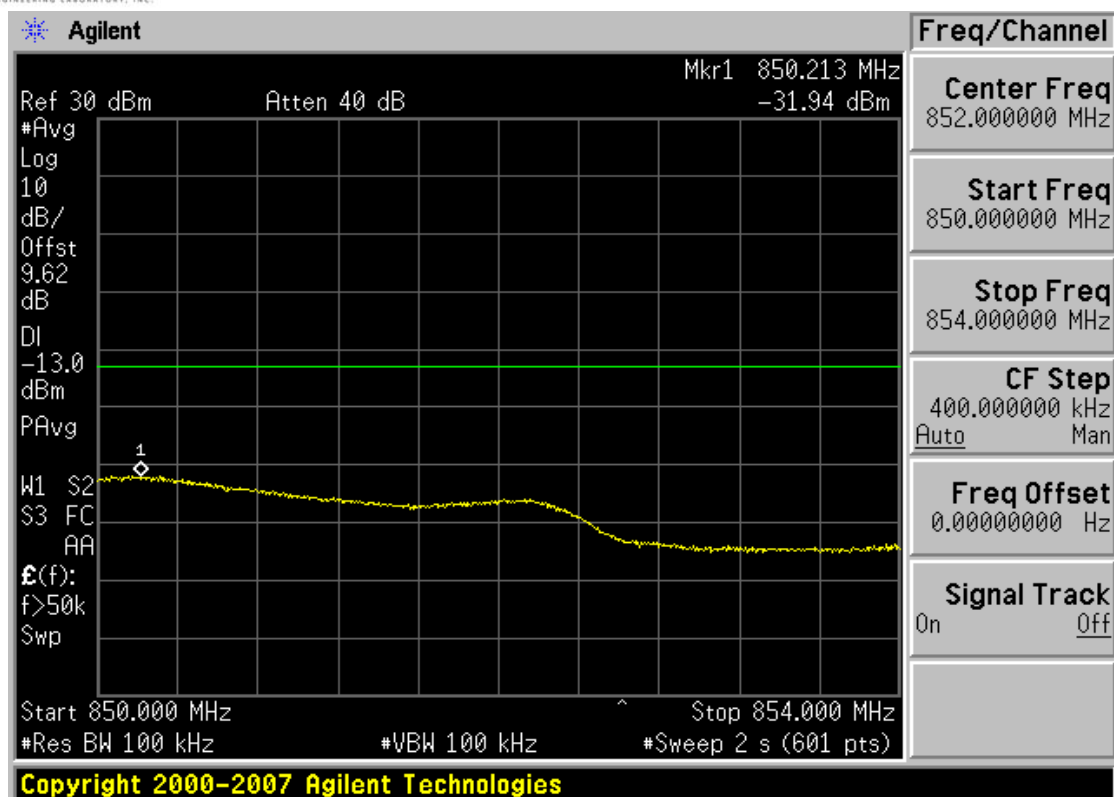
Plot 7-35. 4MHz Span Plot (Cellular WCDMA Mode – Ch. 4233)
