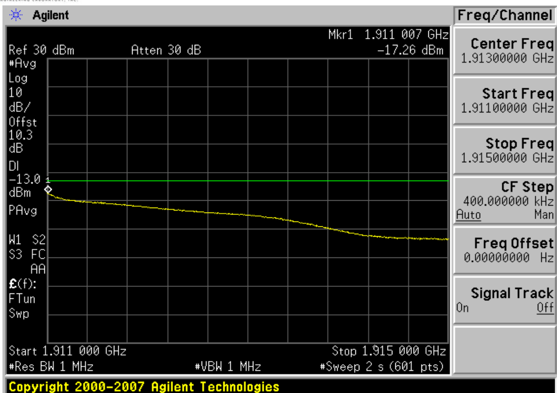
Plot 7-47. 4MHz Span Plot (PCS WCDMA Mode – Ch. 9538)
