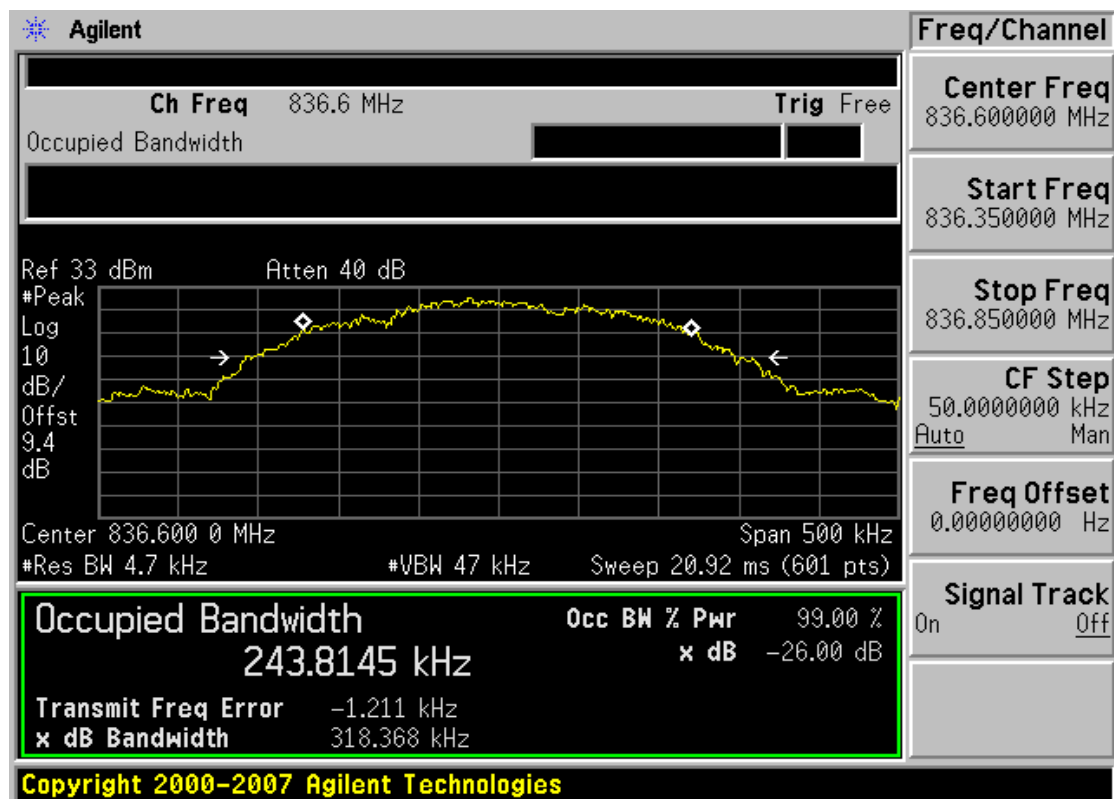
Plot 7-7. Occupied Bandwidth Plot (Cellular GSM Mode – Ch. 190)
