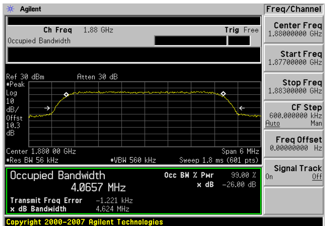
Plot 7-42. Occupied Bandwidth Plot (PCS WCDMA Mode – Ch. 9400)
