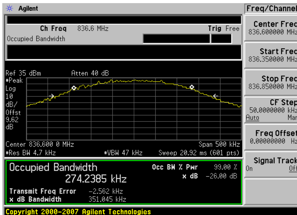
Plot 7-12. Occupied Bandwidth Plot (EDGE850 Mode – Ch. 190)
