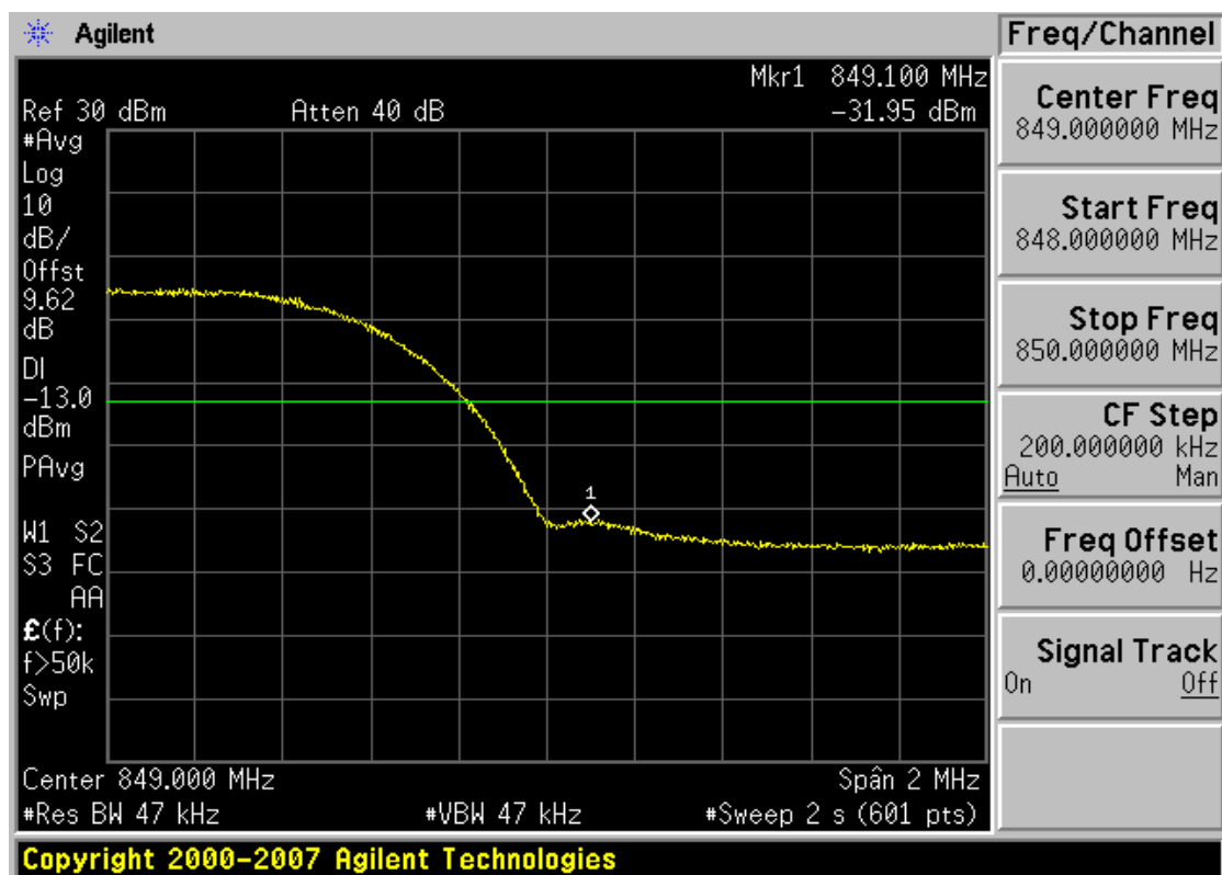
Plot 7-34. Band Edge Plot (Cellular WCDMA Mode – Ch. 4233)
