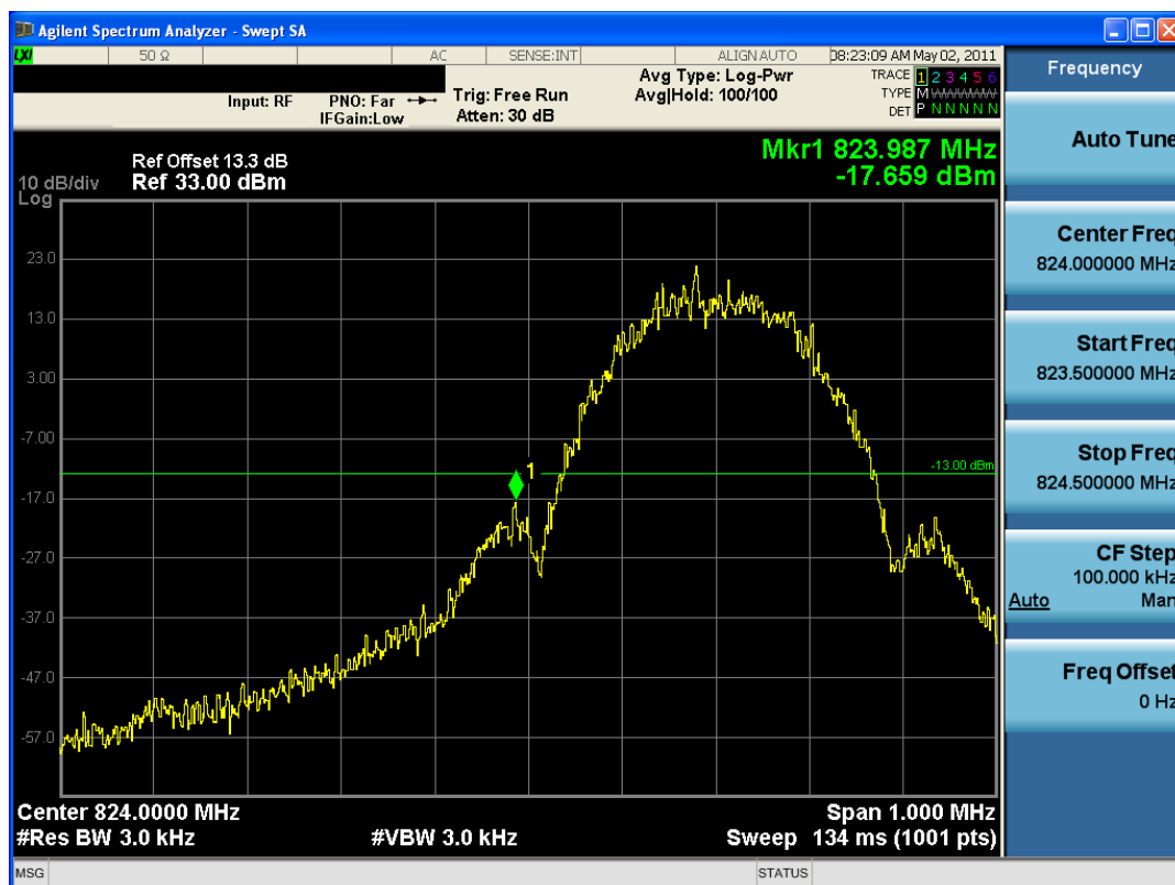
Plot 7-4. Band Edge Plot (Cellular EDGE Mode – Ch. 128)
