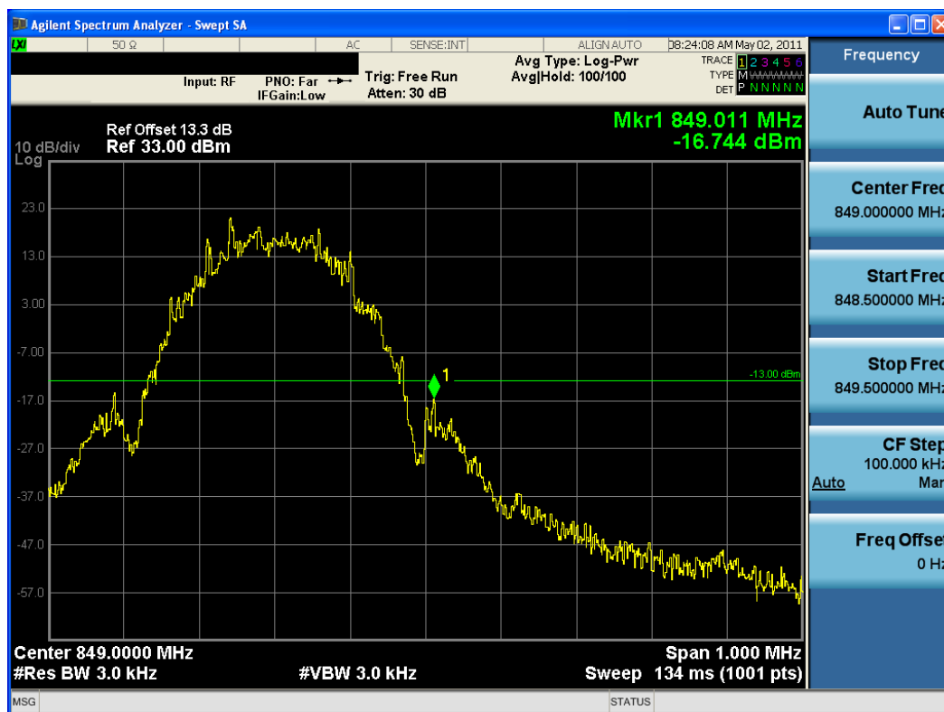
Plot 7-11. Band Edge Plot (Cellular EDGE Mode – Ch. 251)
