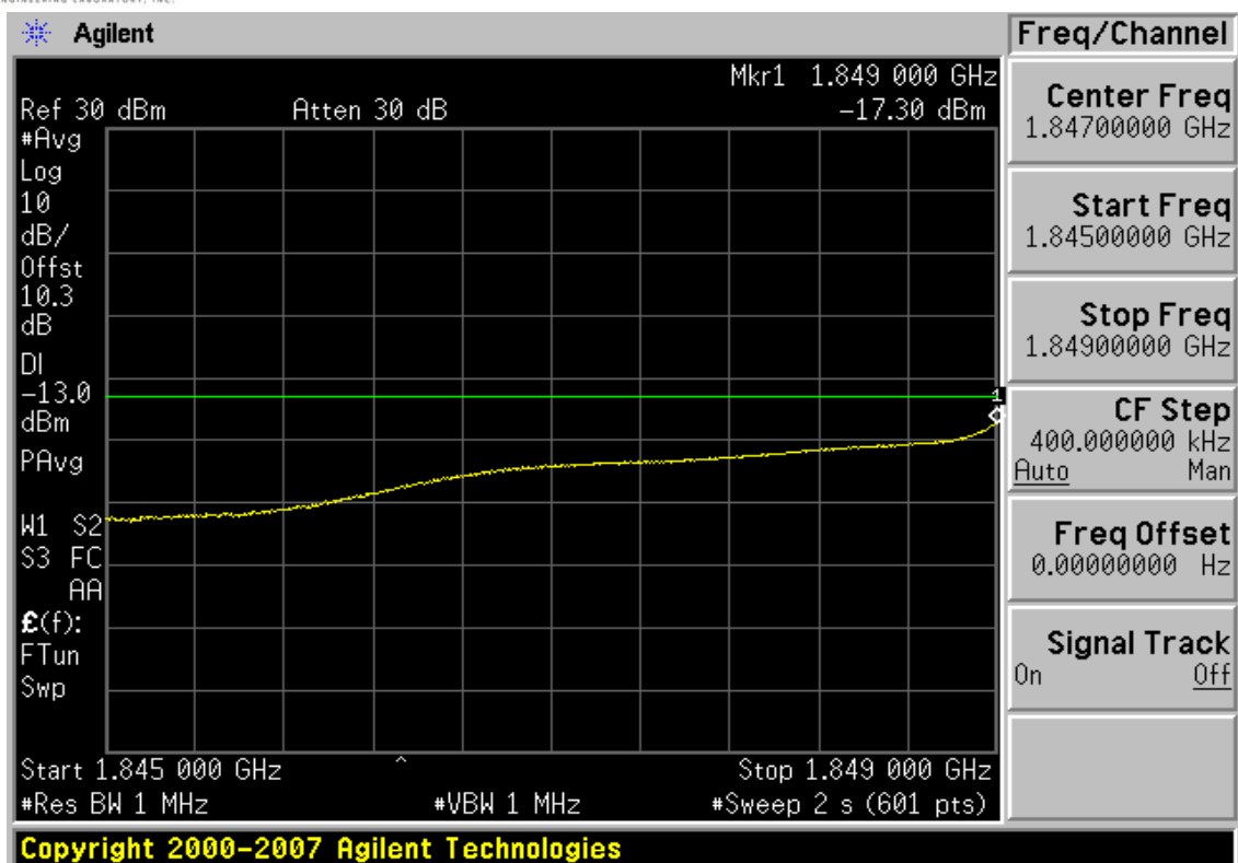
Plot 7-39. 4MHz Span Plot (PCS WCDMA Mode – Ch. 9262)
