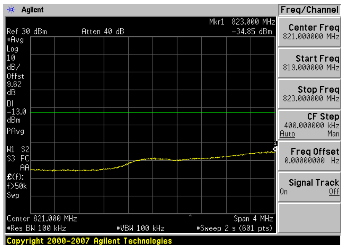
Plot 7-28. 4MHz Span Plot (Cellular WCDMA Mode – Ch. 4132)
