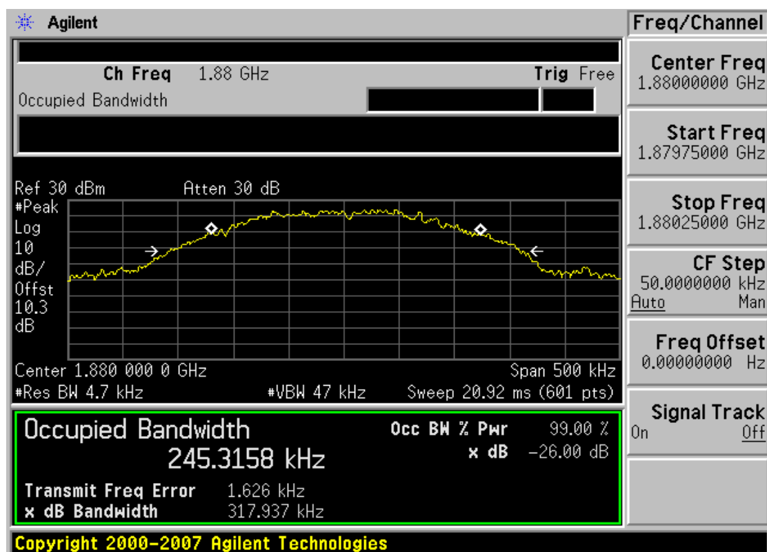
Plot 7-18. Occupied Bandwidth Plot (PCS GSM Mode – Ch. 661)
