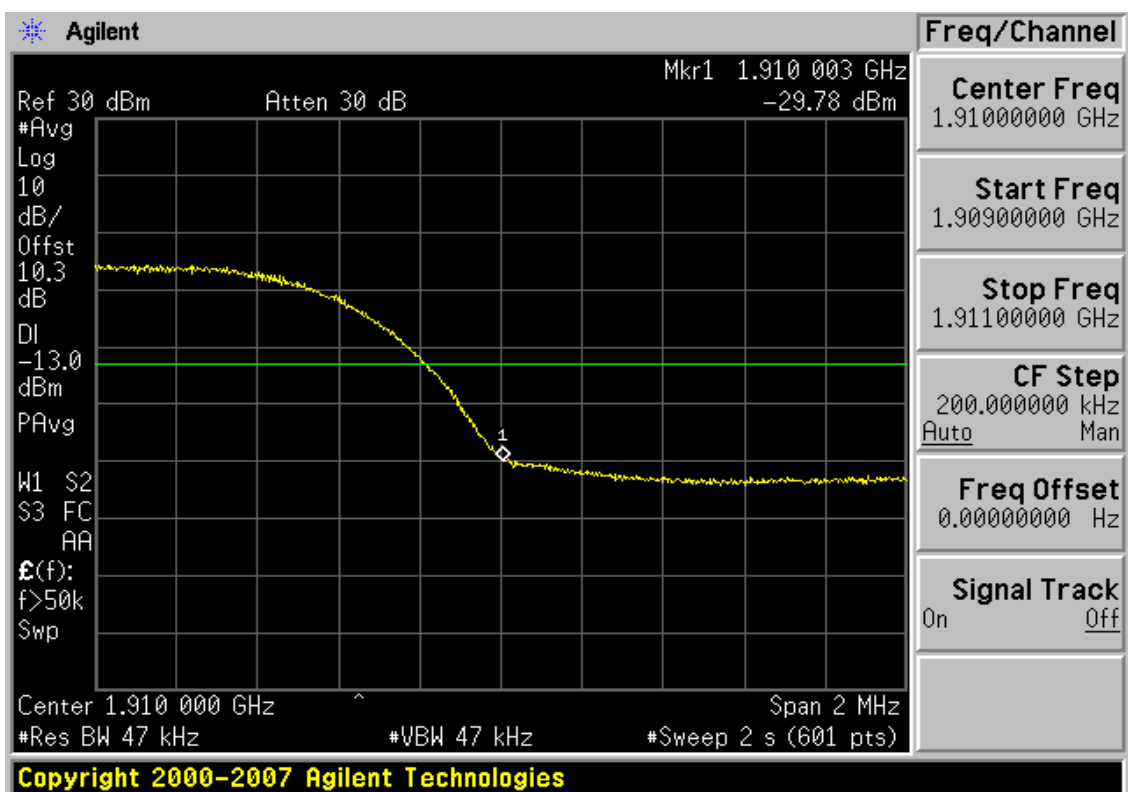
Plot 7-46. Band Edge Plot (PCS WCDMA Mode – Ch. 9538)
