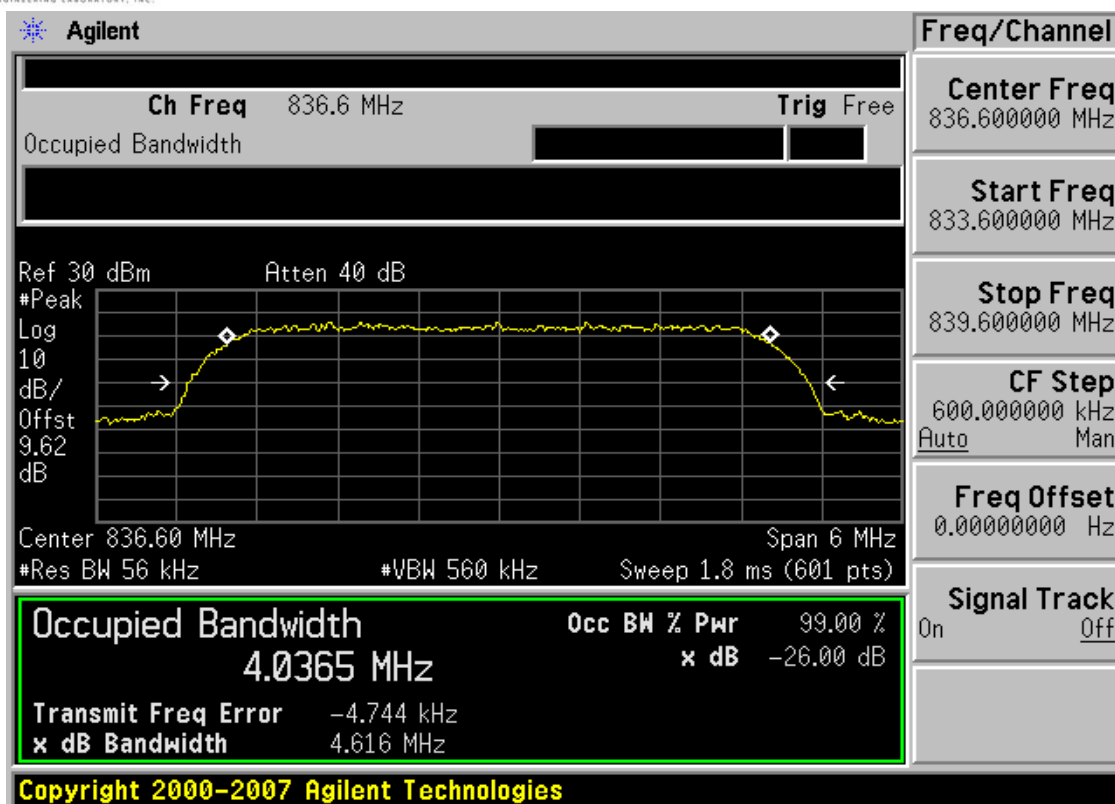
Plot 7-31. Occupied Bandwidth Plot (Cellular WCDMA Mode - Ch. 4183)
