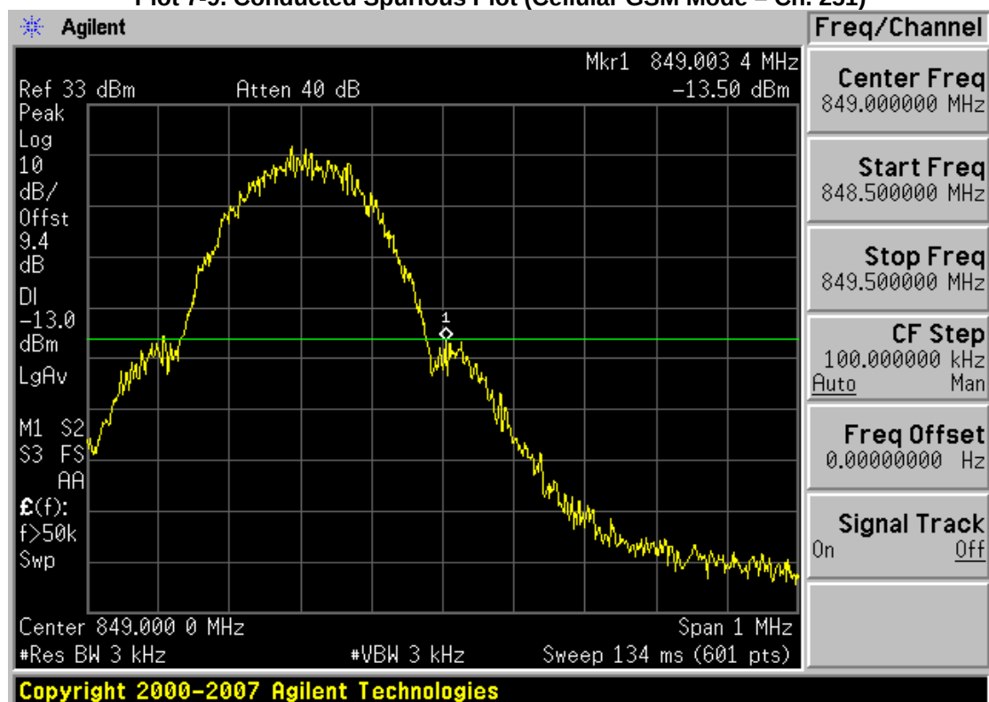
Plot 7-10. Band Edge Plot (Cellular GSM Mode – Ch. 251)
