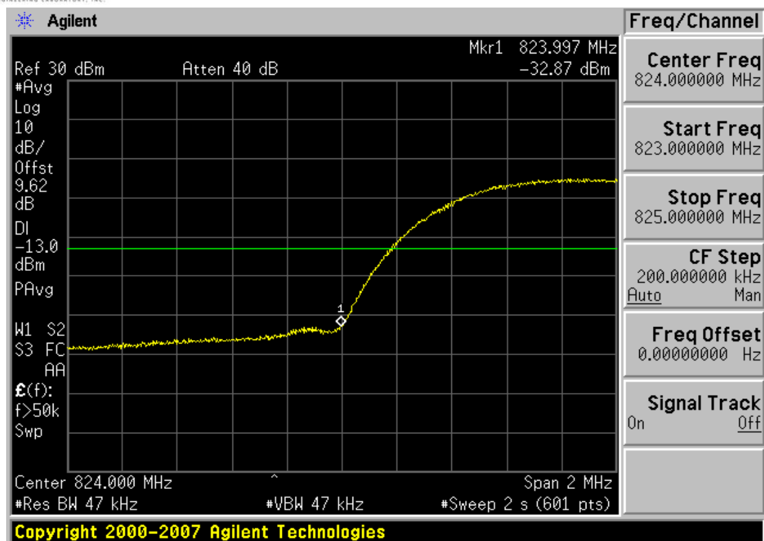
Plot 7-27. Band Edge Plot (Cellular WCDMA Mode – Ch. 4132)
