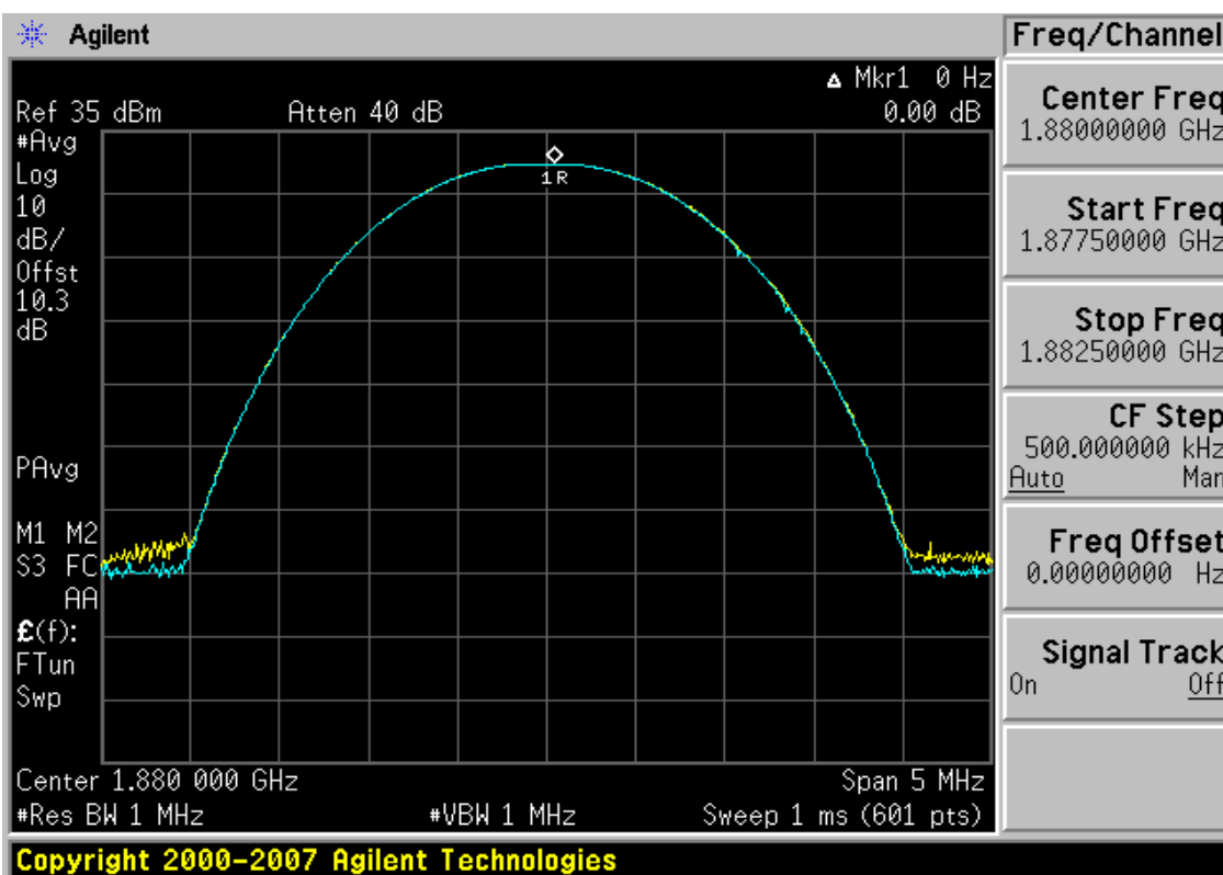
Plot 7-24. Peak-Average Ratio Plot (EDGE1900 Mode – Ch. 661)
