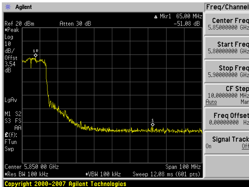
Plot 6-36. Band Edge Plot (802.11a – Ch. 161)
