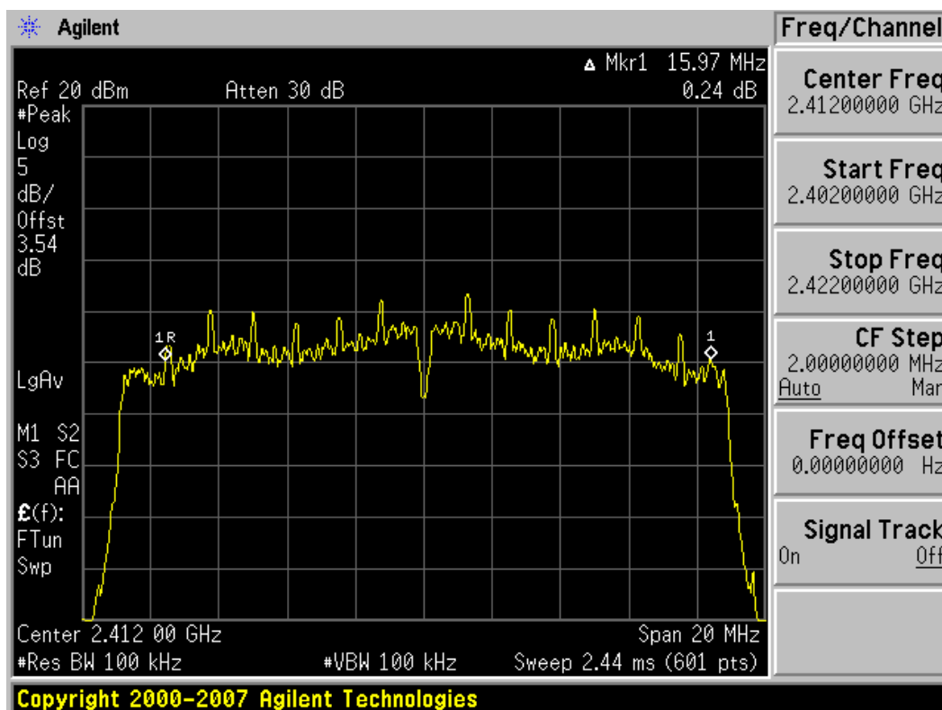
Plot 6-10. 6dB Bandwidth Plot (802.11n (2.4GHz) – Ch. 1)
