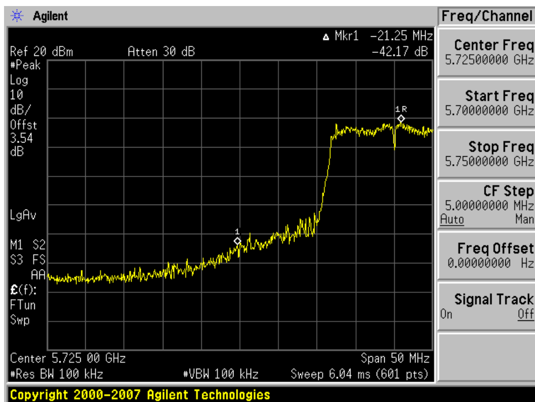
Plot 6-35. Band Edge Plot (802.11a – Ch. 149)
