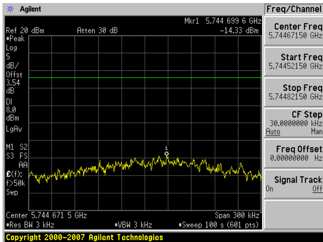
Plot 6-22. Power Spectral Density Plot (802.11a – Ch. 149)
