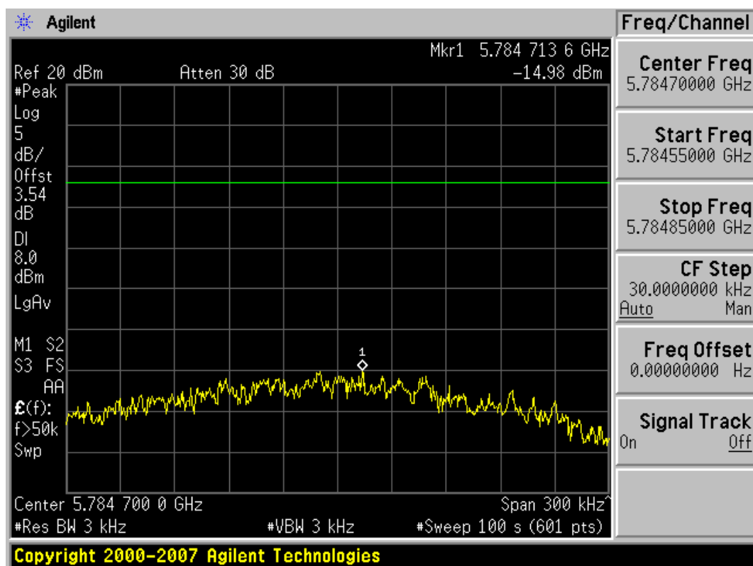
Plot 6-23. Power Spectral Density Plot (802.11a – Ch. 157)
