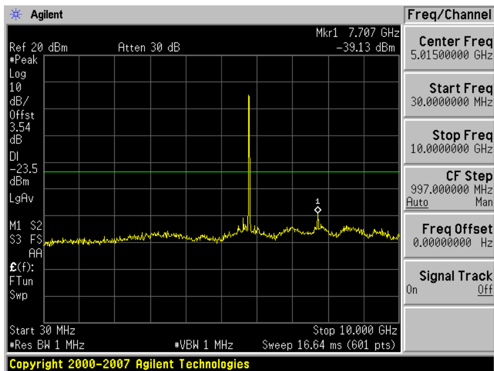
Plot 6-49. Conducted Spurious Plot (802.11a – Ch. 157)
