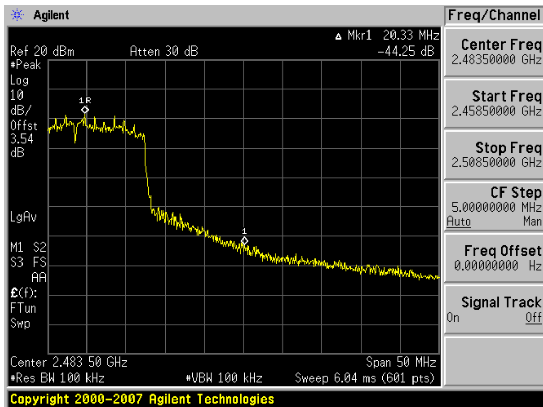
Plot 6-38. Band Edge Plot (802.11n (2.4GHz) – Ch. 11)
