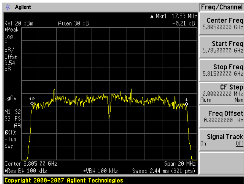
Plot 6-15. 6dB Bandwidth Plot (802.11n (5.8GHz) – Ch. 161)
