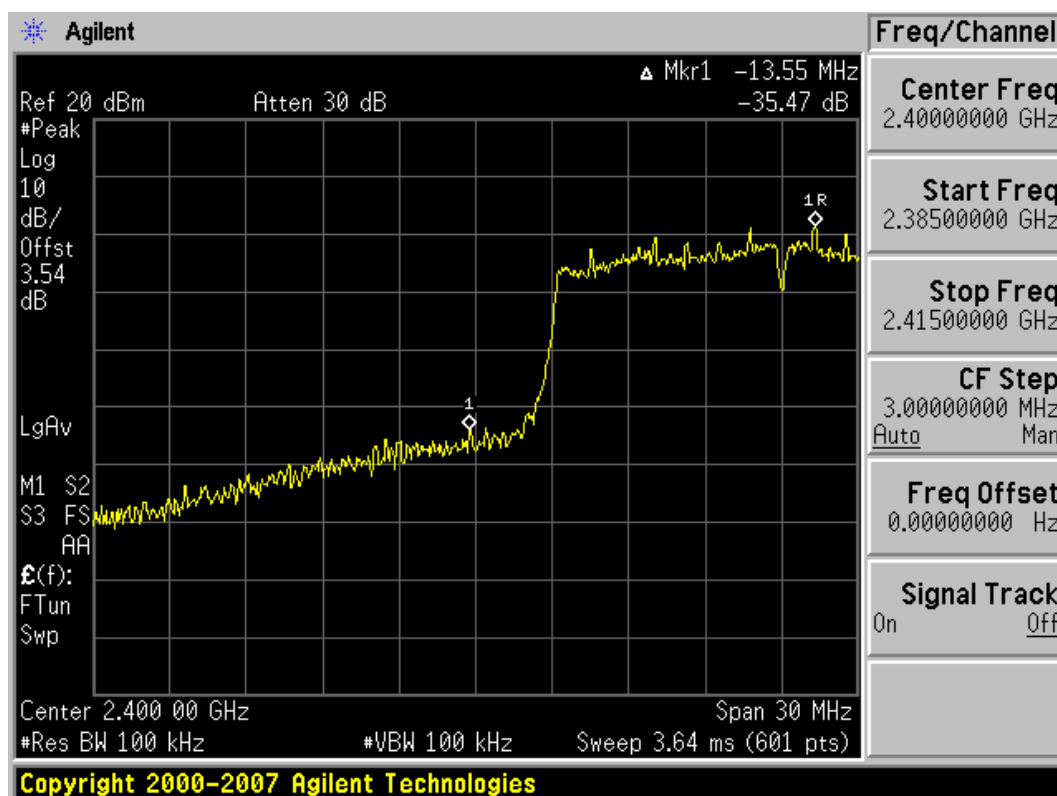
Plot 6-37. Band Edge Plot (802.11n (2.4GHz) – Ch. 1)
