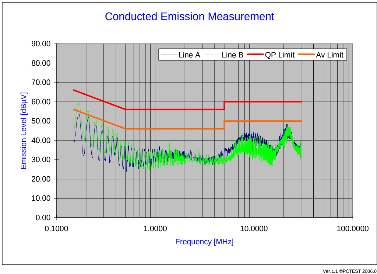
Plot 6-57. Line Conducted Plot with 802.11n (5.8GHz)
