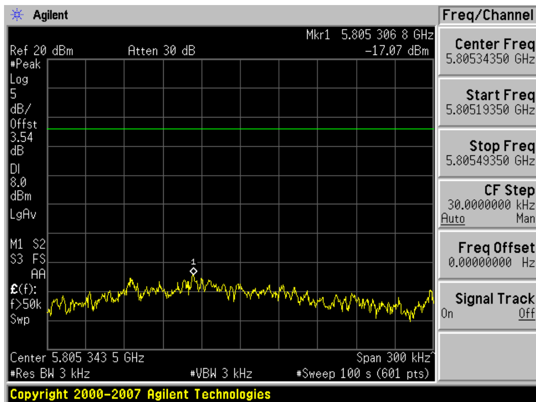
Plot 6-30. Power Spectral Density Plot (802.11n (5.8GHz) – Ch. 161)
