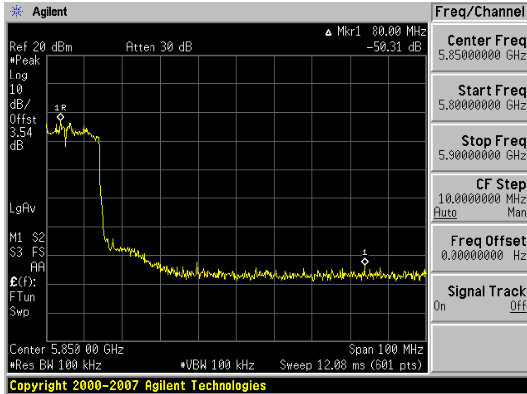
Plot 6-40. Band Edge Plot (802.11n (5.8GHz) – Ch. 161)
