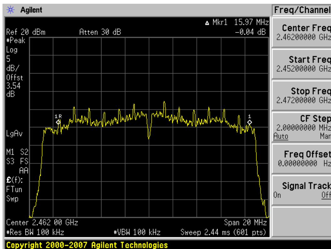
Plot 6-12. 6dB Bandwidth Plot (802.11n (2.4GHz) - Ch. 11)
