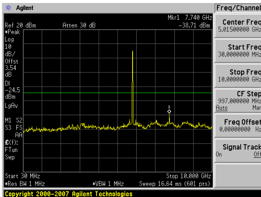
Plot 6-51. Conducted Spurious Plot (802.11a – Ch. 161)
