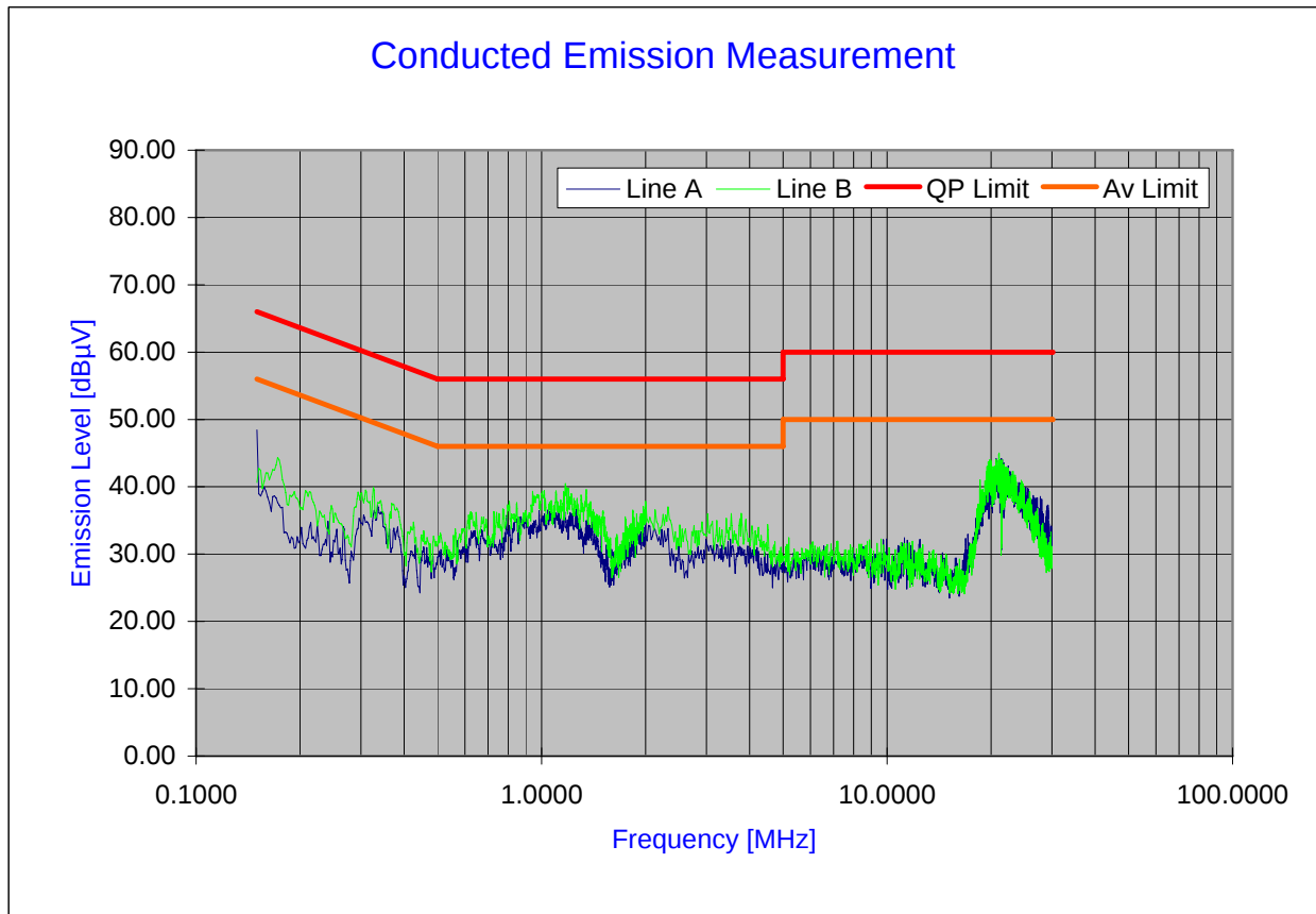
Plot 6-56. Line Conducted Plot with 802.11b
