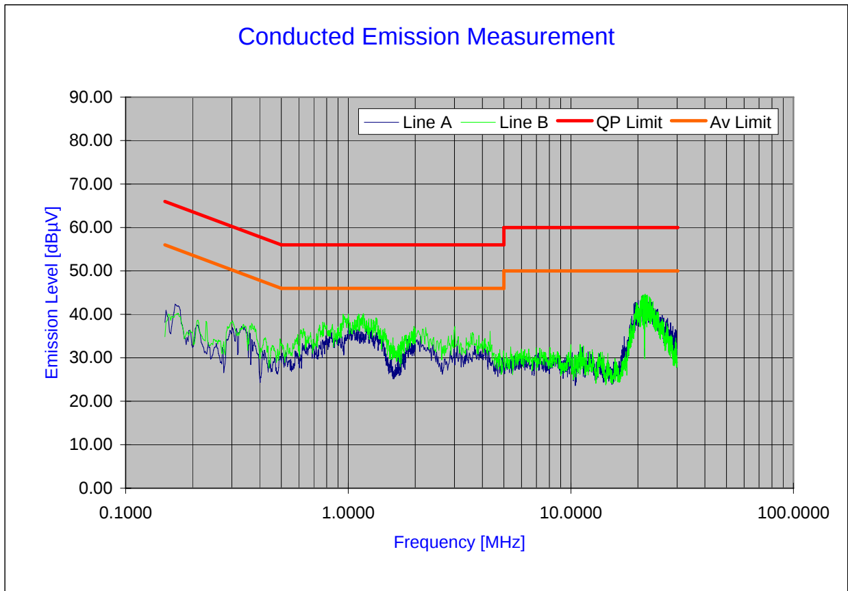
Plot 6-60. Line Conducted Plot with 802.11n (5.8GHz)
