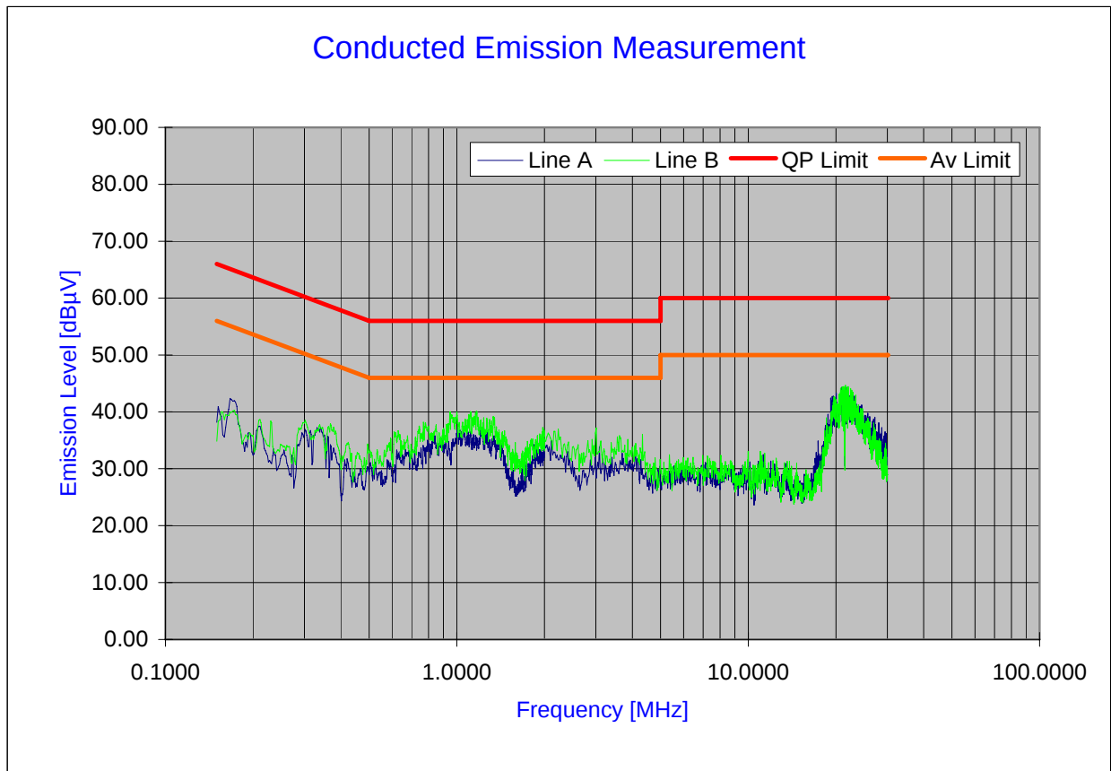
Plot 6-59. Line Conducted Plot with 802.11n (2.4GHz)
