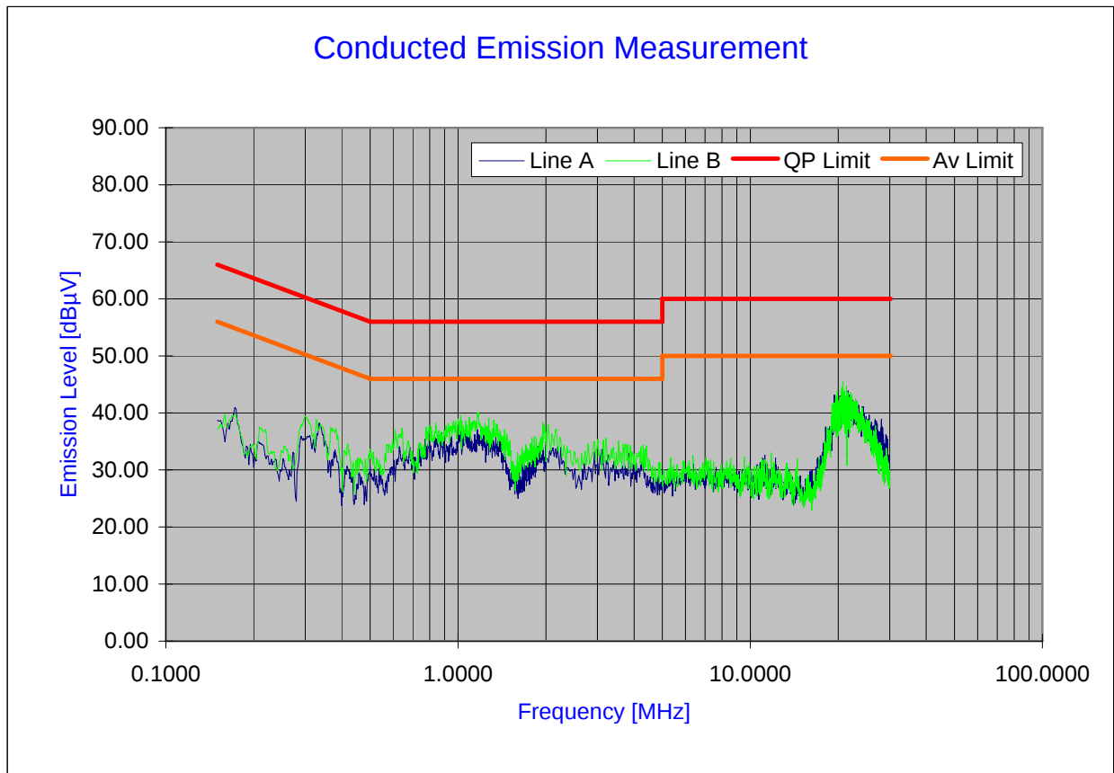
Plot 6-57. Line Conducted Plot with 802.11g
