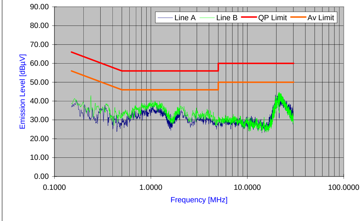
Plot 6-56. Line Conducted Plot with 802.11a (UNII Band 2)
