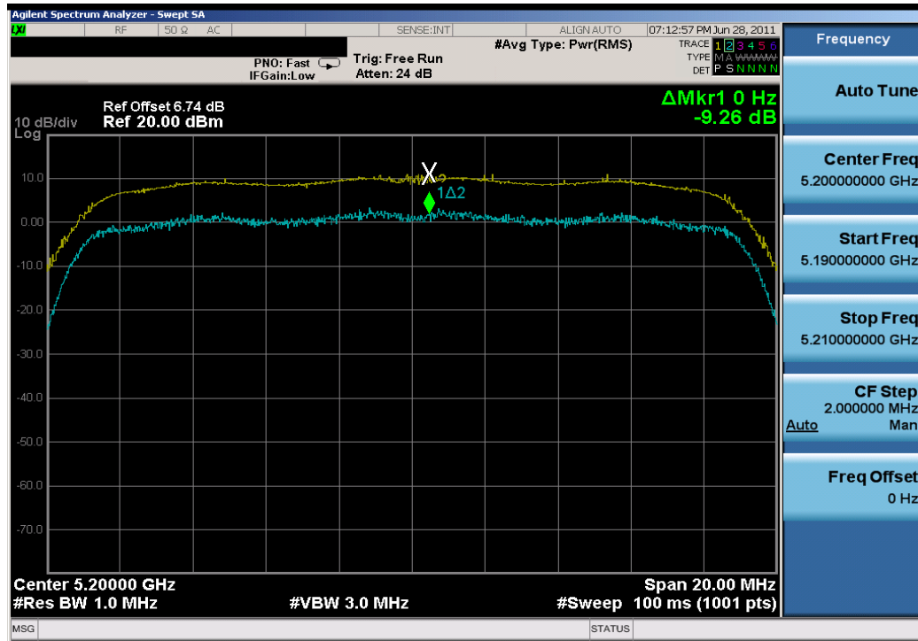
Plot 6-41. Peak Excursion Ratio Plot (802.11n (UNII Band 1) – Ch. 40)
