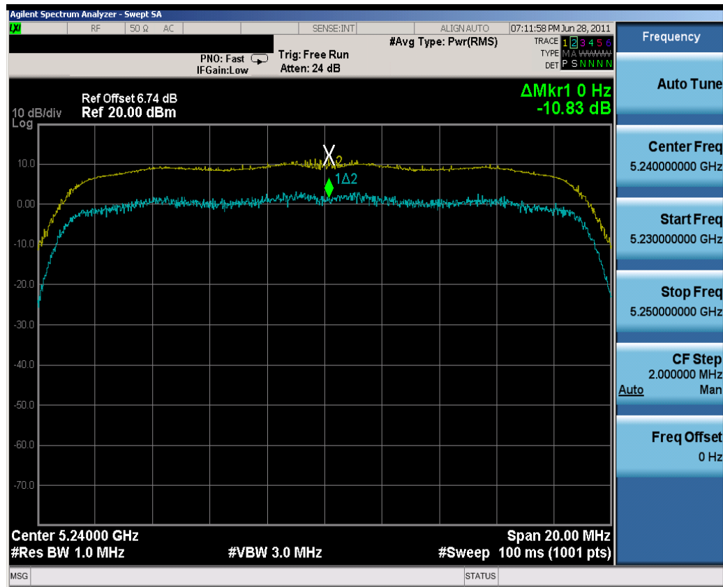
Plot 6-42. Peak Excursion Ratio Plot (802.11n (UNII Band 1) – Ch. 48)
