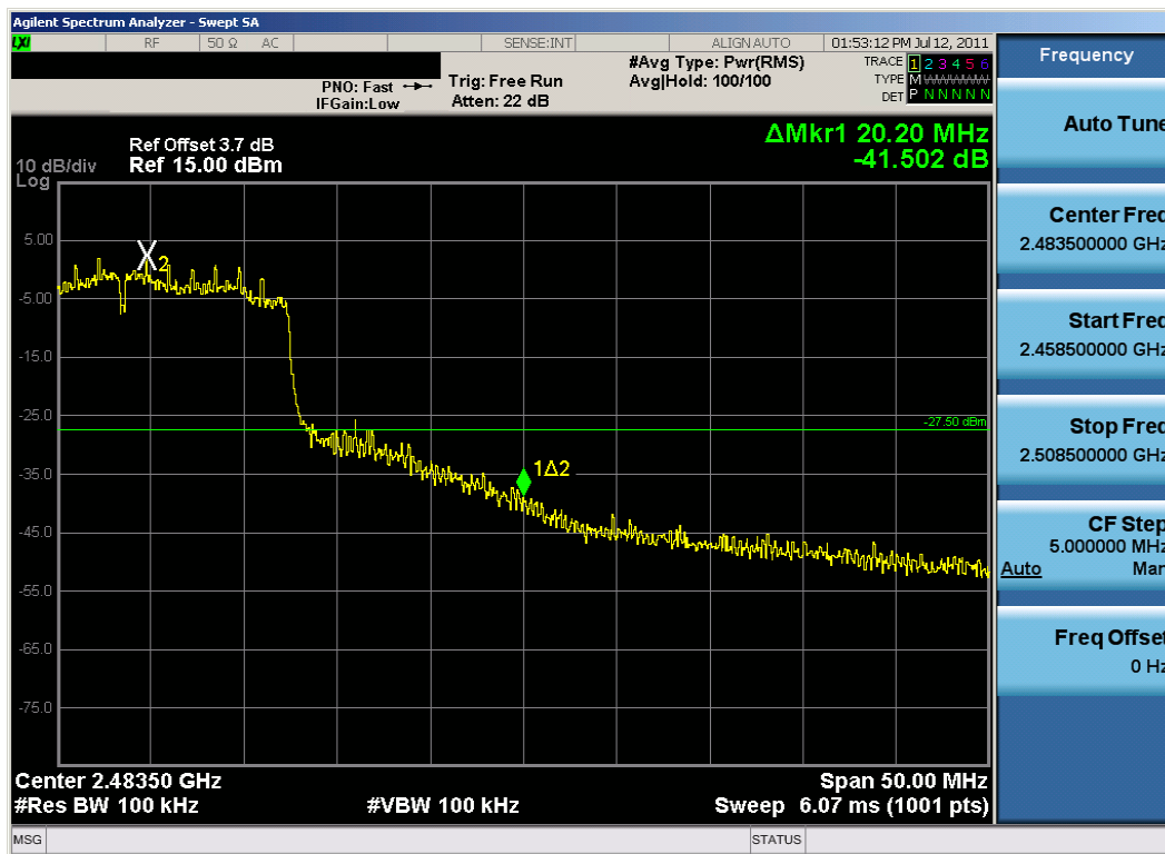
Plot 6-38. Band Edge Plot (802.11n (2.4GHz) – Ch. 11)
