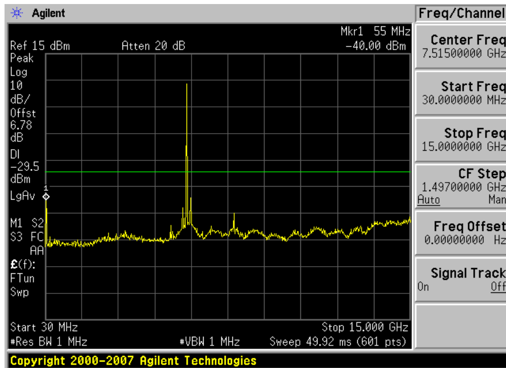
Plot 6-51. Conducted Spurious Plot (802.11a – Ch. 165)
