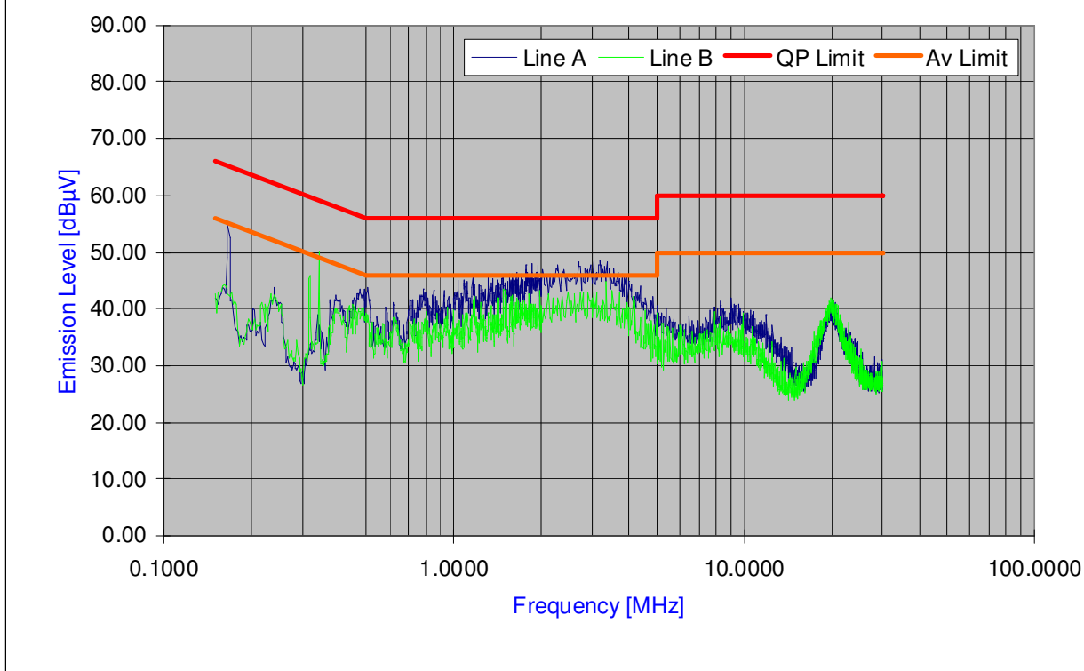
Plot 6-59. Line Conducted Plot with 802.11n (UNII Band 2)
