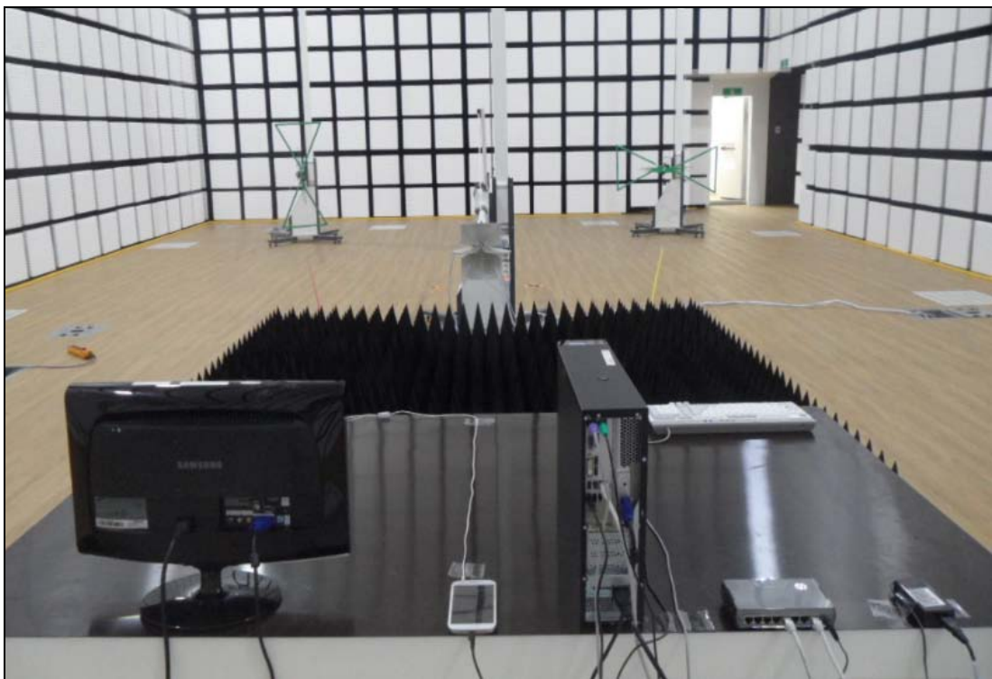
[ Radiated Disturbance for Above 1 GHz – Rear ]
