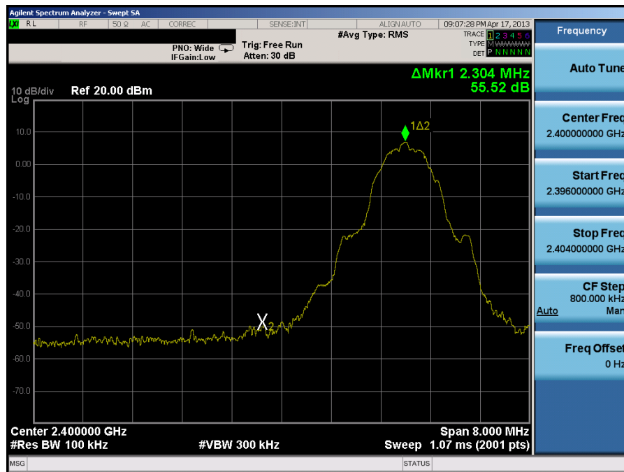
Plot 6-10. Band Edge Plot (Bluetooth (LE) – Ch. 0)
