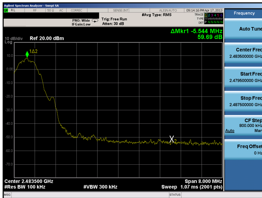
Plot 6-11. Band Edge Plot (Bluetooth (LE) – Ch. 39)
