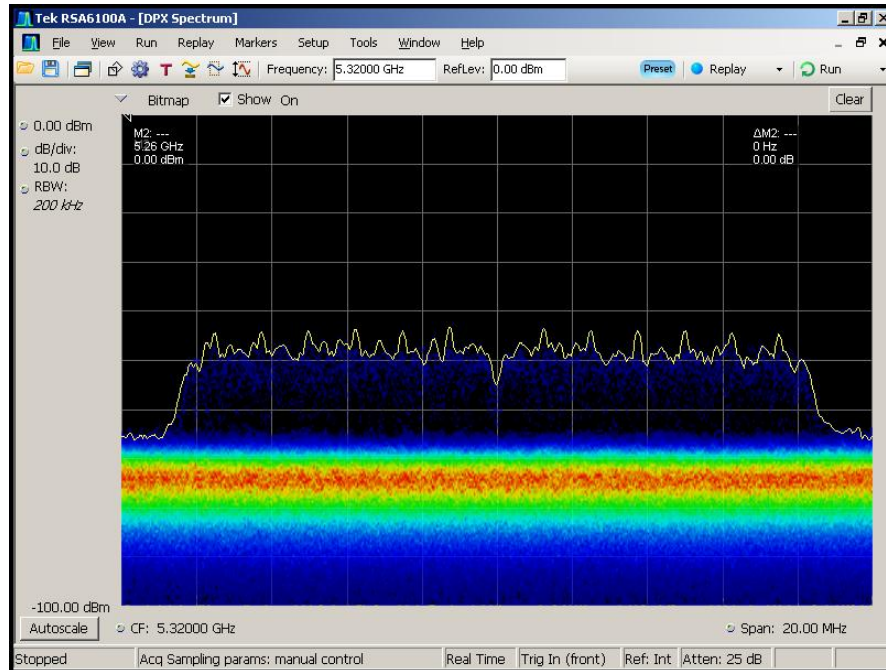
Figure 5-3. Real-Time Spectrum Display, No WLAN Traffic
