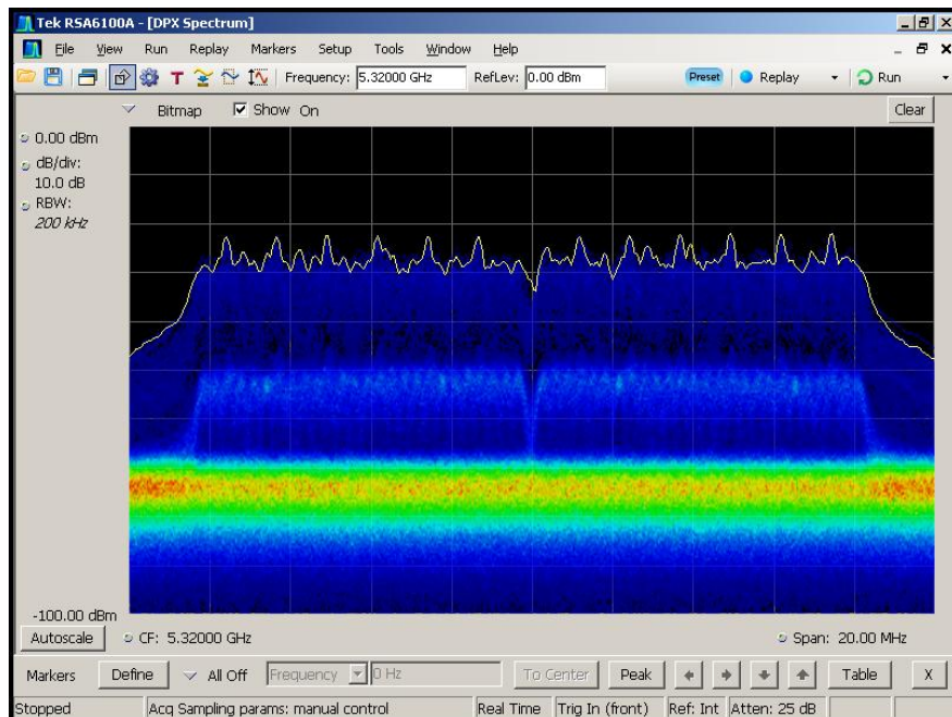
Figure 5-2. Real-Time Spectrum Display WLAN Channel Traffic (Streaming Video)
