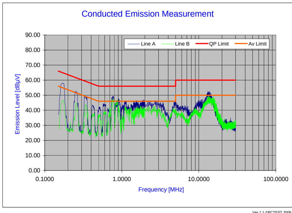
Plot 6-54. Line Conducted Plot with 802.11a UNII Band 1
