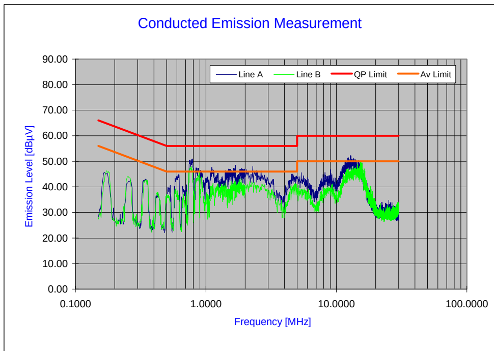
Plot 6-55. Line Conducted Plot with 802.11a UNII Band 2 (L1)
