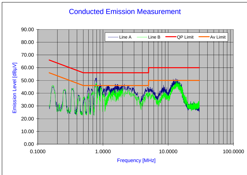
Plot 6-56. Line Conducted Plot with 802.11a UNII Band 3 (L1)
