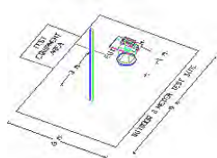
Figure 3-7. Turntable and System Setup
