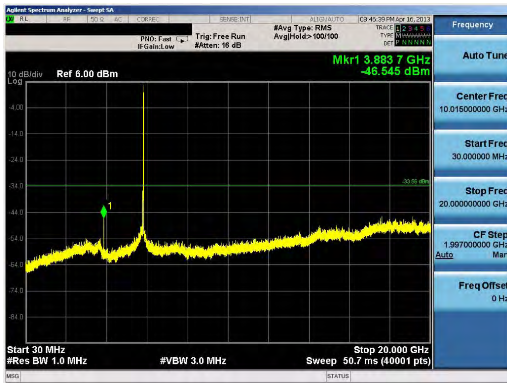
Plot 6-57. Conducted Spurious Plot (802.11a – Ch. 165)
