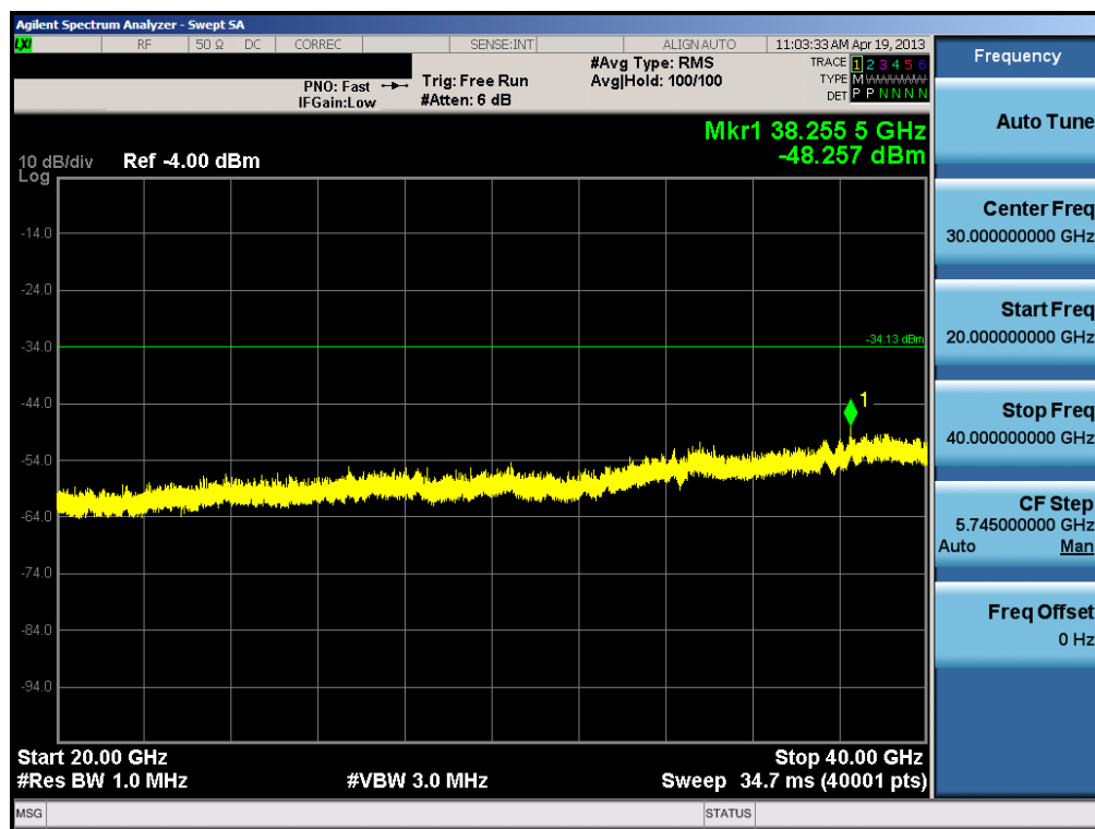
Plot 6-56. Conducted Spurious Plot (802.11a – Ch. 157)
