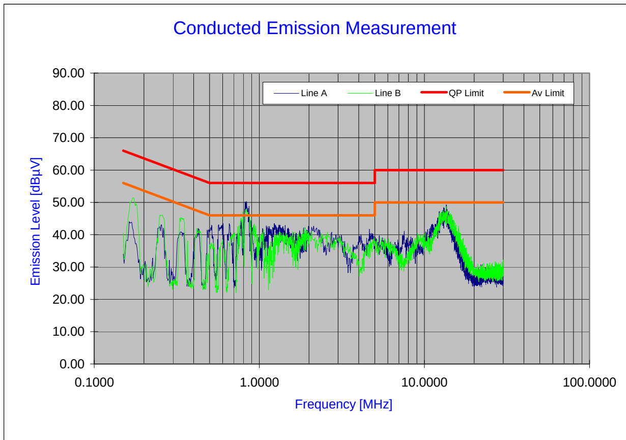
Plot 6-63. Line Conducted Plot with 802.11a
