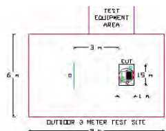
Figure 3-6. Dimensions of Outdoor Test Site
