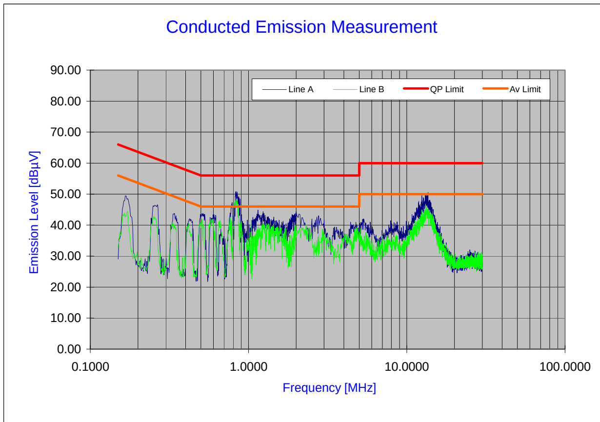
Plot 6-64. Line Conducted Plot with 802.11b
