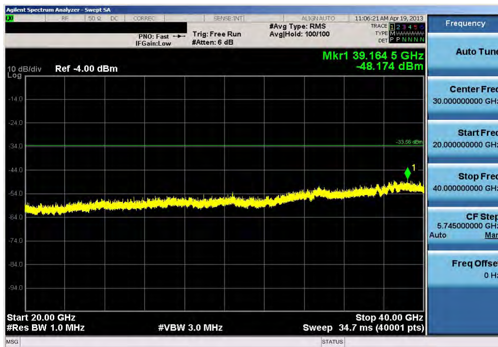
Plot 6-58. Conducted Spurious Plot (802.11a – Ch. 165)
