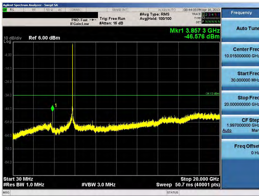
Plot 6-55. Conducted Spurious Plot (802.11a – Ch. 157)
