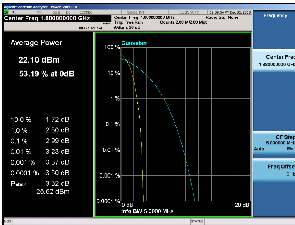
Plot 6-46. Peak-Average Ratio Plot (PCS WCDMA Mode – Ch. 9400)
