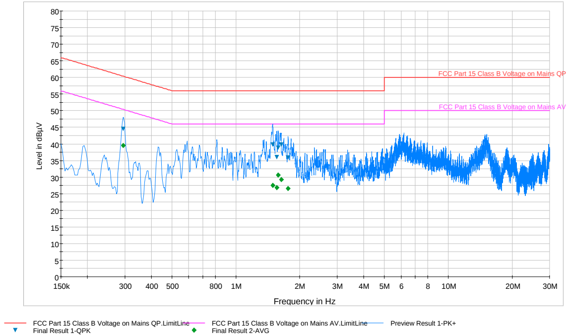
Plot 6-75. Line Conducted Plot with 802.11a UNII Band 2a (N)
