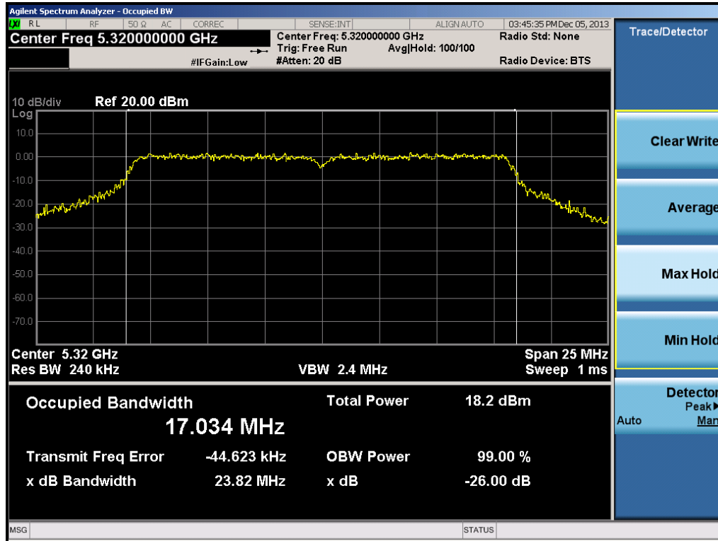
Plot 6-11. 26dB Bandwidth Plot (802.11a Ch. 64)
