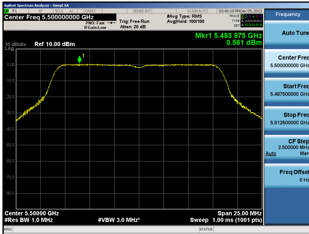
Plot 6-46. Peak Power Spectral Density Plot (802.11a Ch. 100)
