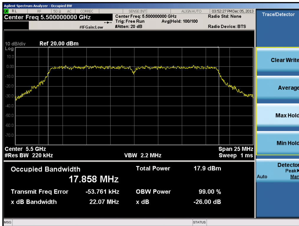
Plot 6-20. 26dB Bandwidth Plot (20MHz BW 802.11n Ch. 100)
