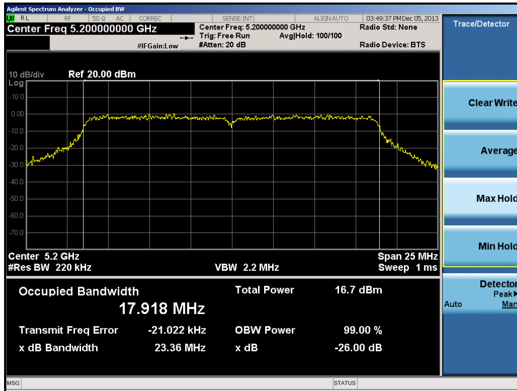
Plot 6-5. 26dB Bandwidth Plot (20MHz BW 802.11n Ch. 40)
