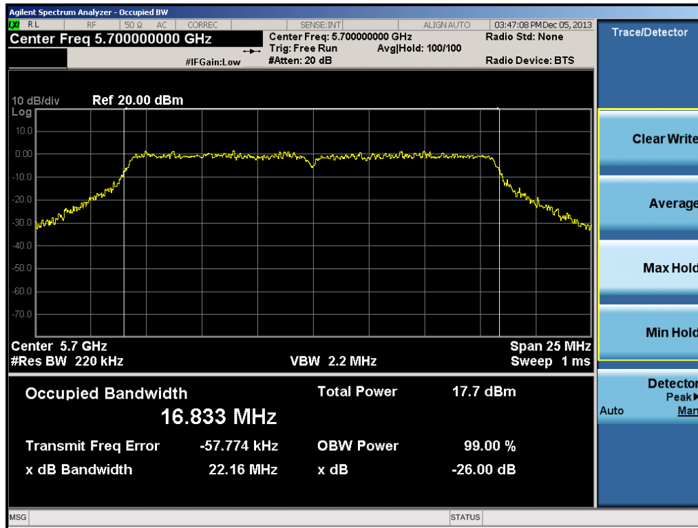
Plot 6-19. 26dB Bandwidth Plot (802.11a Ch. 140)
