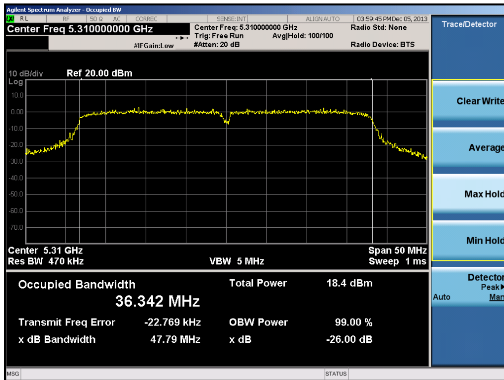
Plot 6-16. 26dB Bandwidth Plot (40MHz BW 802.11n Ch. 62)
