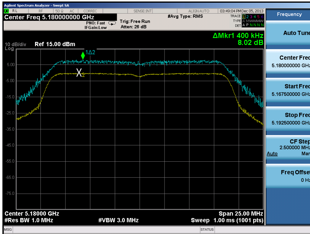
Plot 6-56. Peak Excursion Ratio Plot (20MHz BW 802.11n)
