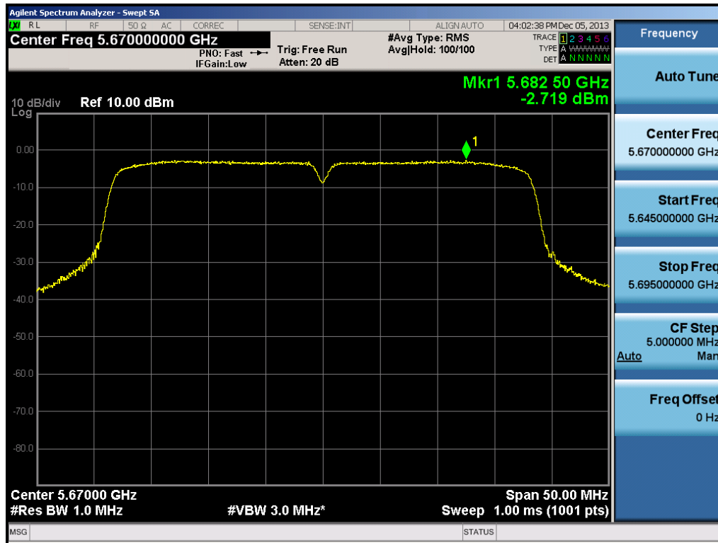
Plot 6-54. Peak Power Spectral Density Plot (40MHz BW 802.11n Ch. 134)
