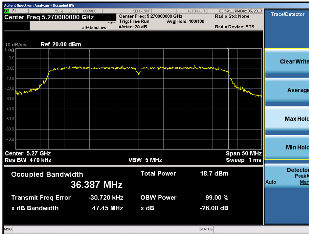
Plot 6-15. 26dB Bandwidth Plot (40MHz BW 802.11n Ch. 54)
