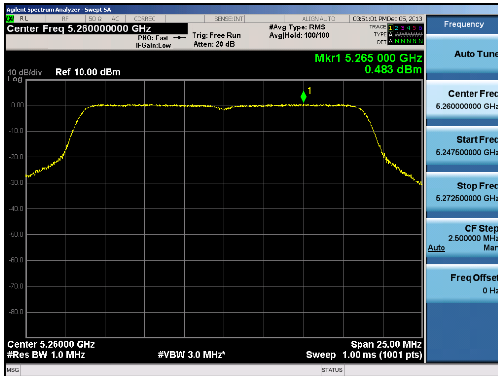
Plot 6-41. Peak Power Spectral Density Plot (20MHz BW 802.11n Ch. 52)
