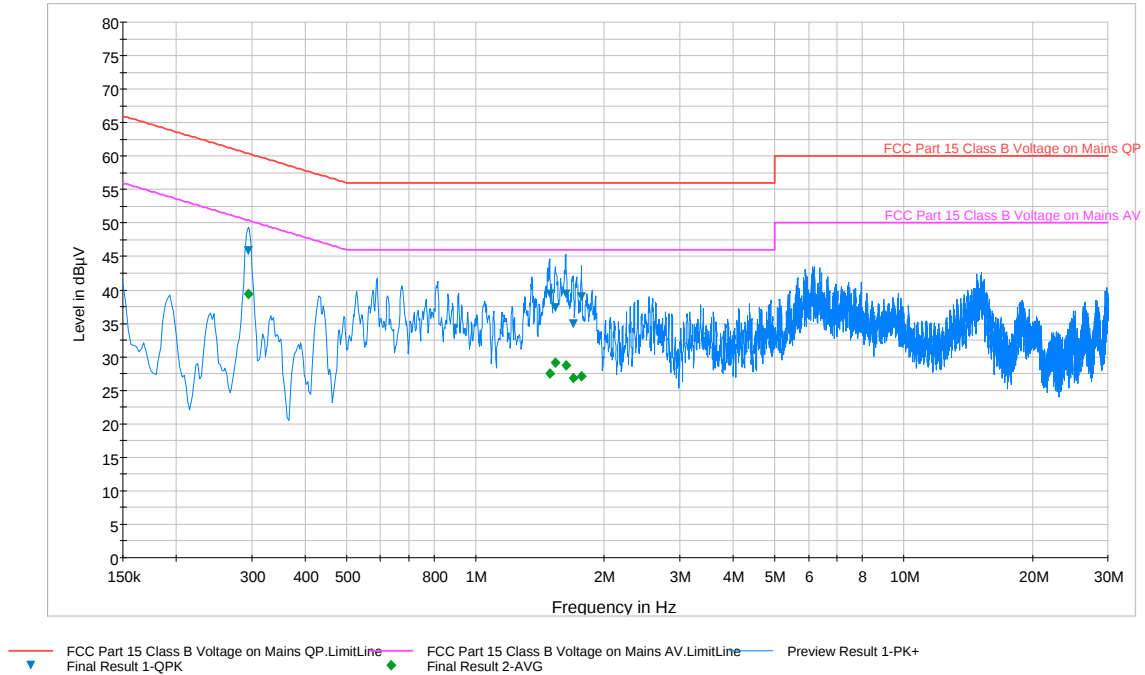
Plot 6-73. Line Conducted Plot with 802.11a UNII Band 1 (N)
