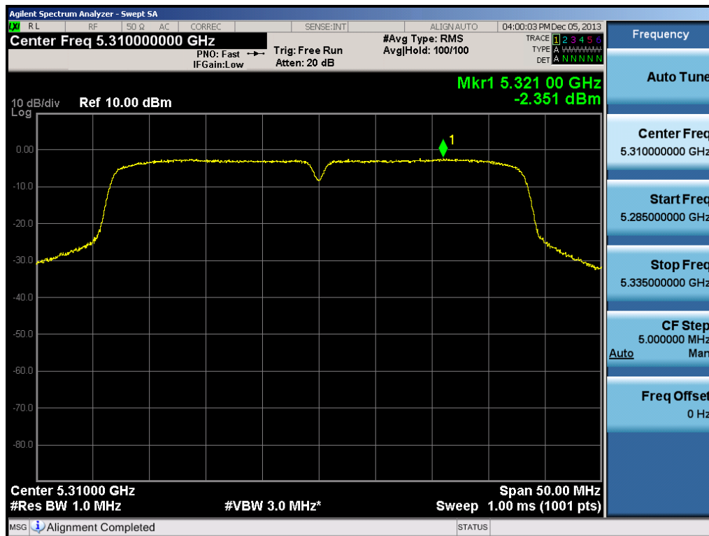
Plot 6-45. Peak Power Spectral Density Plot (40MHz BW 802.11n Ch. 62)
