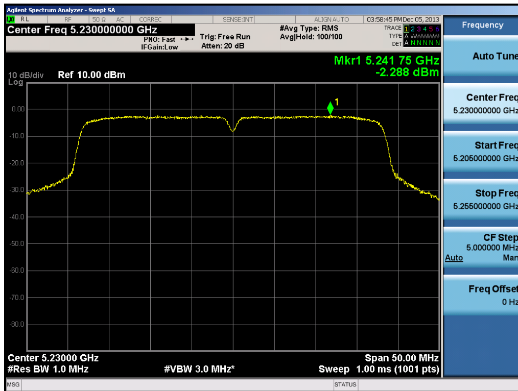
Plot 6-37. Peak Power Spectral Density Plot (40MHz BW 802.11n Ch. 46)
