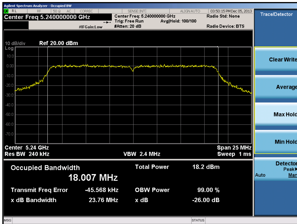
Plot 6-6. 26dB Bandwidth Plot (20MHz BW 802.11n Ch. 48)
