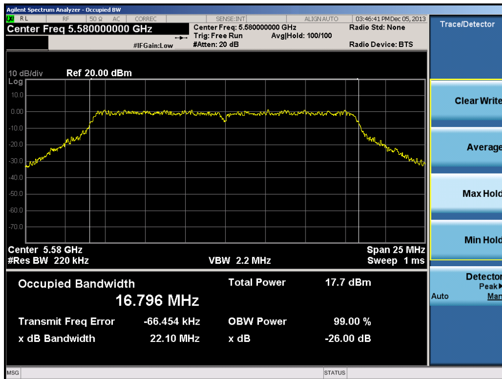
Plot 6-18. 26dB Bandwidth Plot (802.11a Ch. 116)
