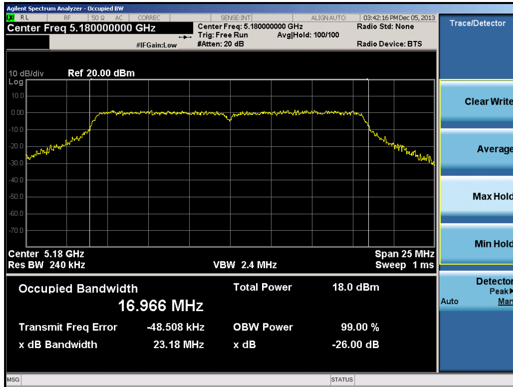
Plot 6-1. 26dB Bandwidth Plot (802.11a Ch. 36)
