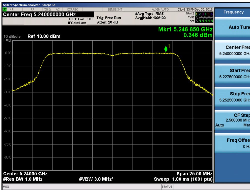
Plot 6-32. Peak Power Spectral Density Plot (802.11a Ch. 48)
