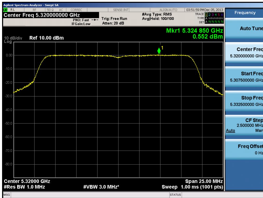
Plot 6-43. Peak Power Spectral Density Plot (20MHz BW 802.11n Ch. 64)
