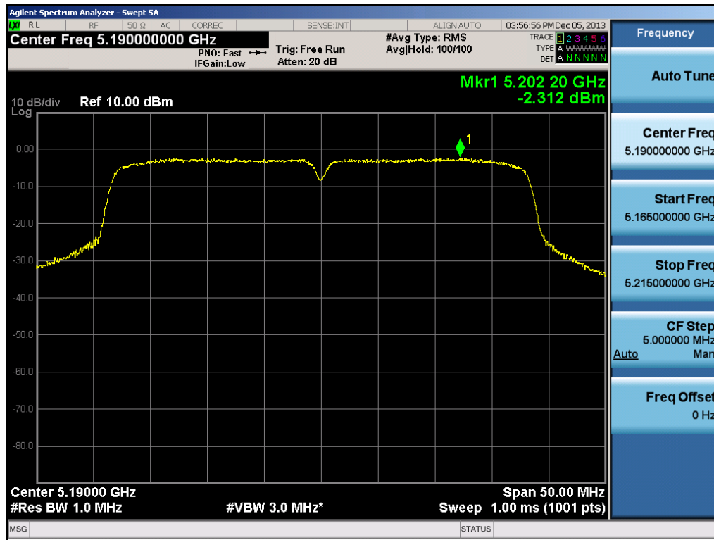
Plot 6-36. Peak Power Spectral Density Plot (40MHz BW 802.11n Ch. 38)
