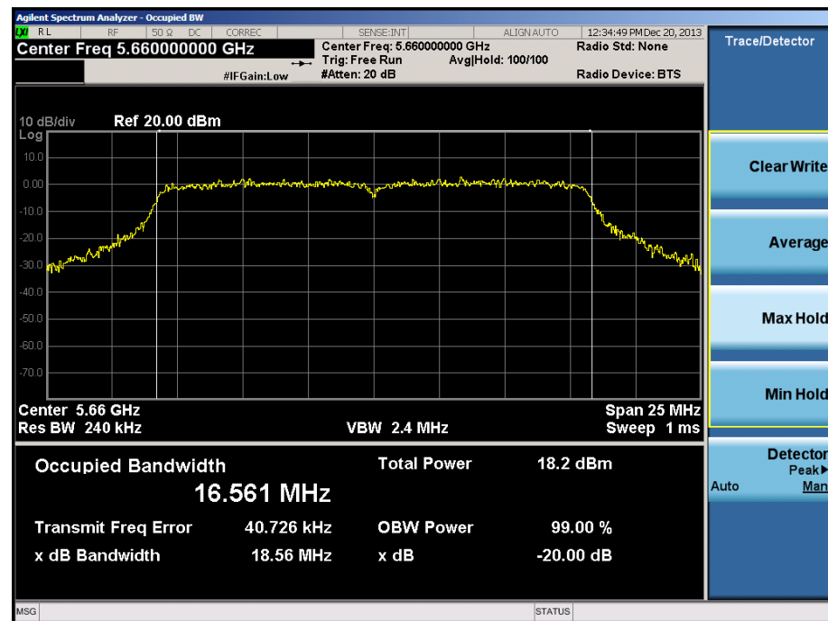
Plot 6-28. 20dB Bandwidth Plot (20MHz BW 802.11n Ch. 132)
