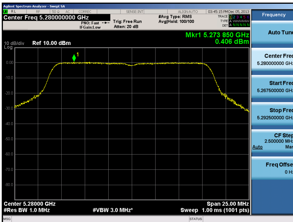
Plot 6-39. Peak Power Spectral Density Plot (802.11a Ch. 56)
