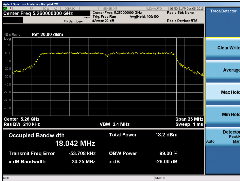
Plot 6-12. 26dB Bandwidth Plot (20MHz BW 802.11n Ch. 52)
