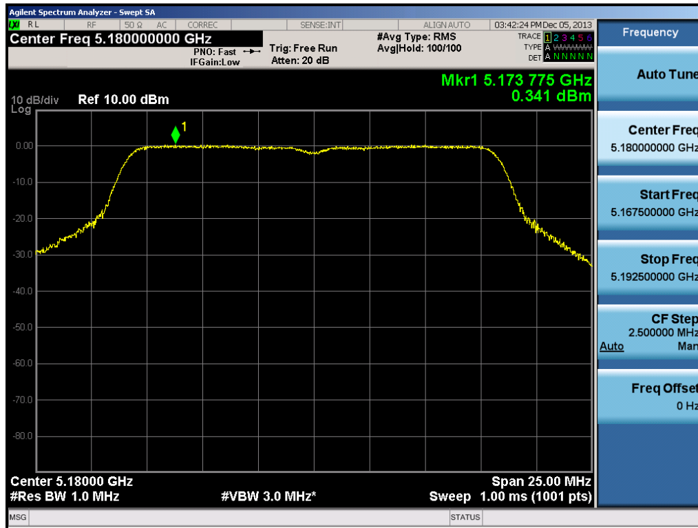
Plot 6-30. Peak Power Spectral Density Plot (802.11a Ch. 36)
