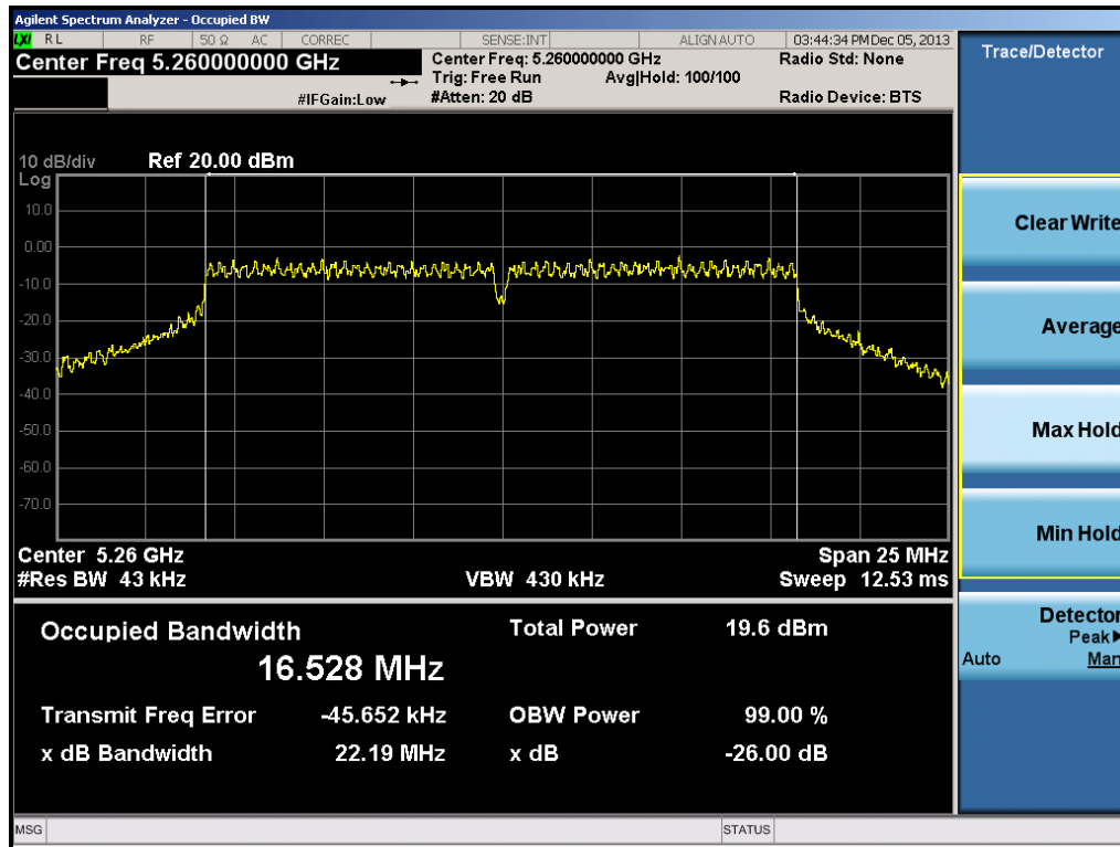
Plot 6-9. 26dB Bandwidth Plot (802.11a Ch. 52)
