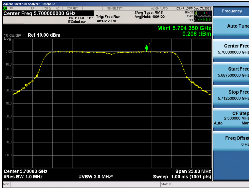
Plot 6-48. Peak Power Spectral Density Plot (802.11a Ch. 140)
