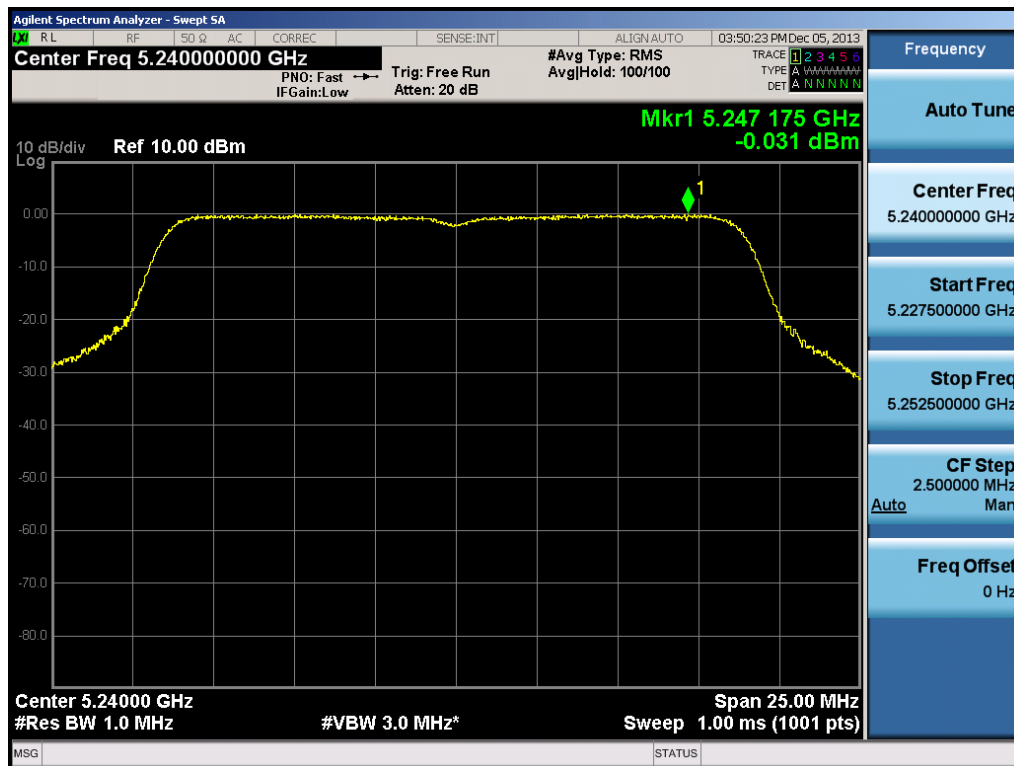
Plot 6-35. Peak Power Spectral Density Plot (20MHz BW 802.11n Ch. 48)
