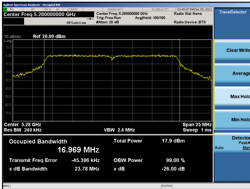
Plot 6-10. 26dB Bandwidth Plot (802.11a Ch. 56)
