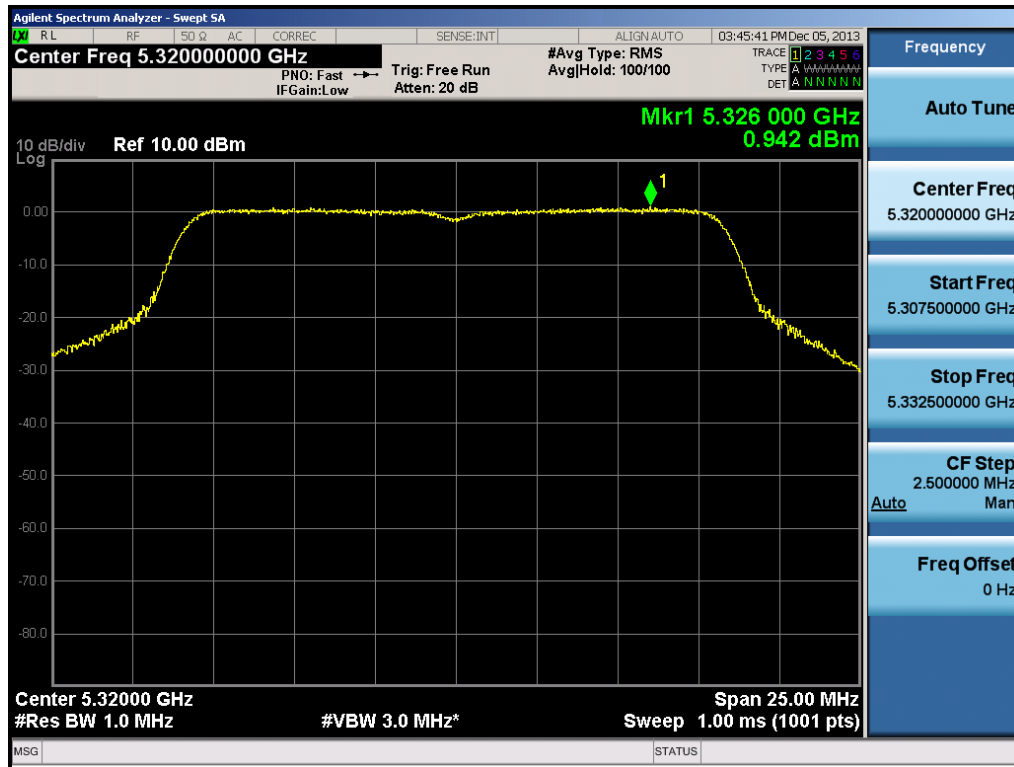
Plot 6-40. Peak Power Spectral Density Plot (802.11a Ch. 64)
