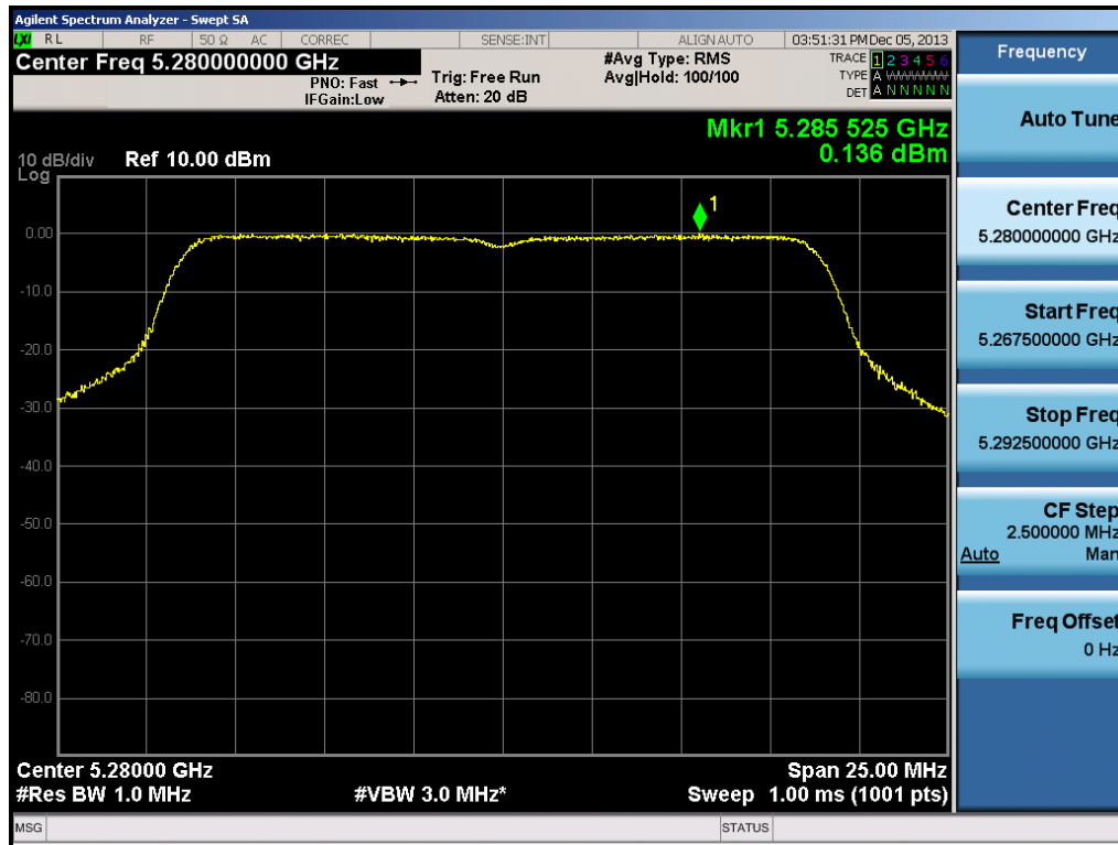
Plot 6-42. Peak Power Spectral Density Plot (20MHz BW 802.11n Ch. 56)
