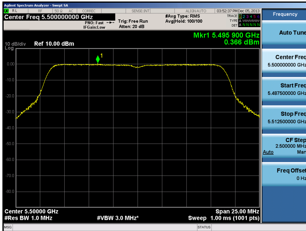
Plot 6-49. Peak Power Spectral Density Plot (20MHz BW 802.11n Ch. 100)
