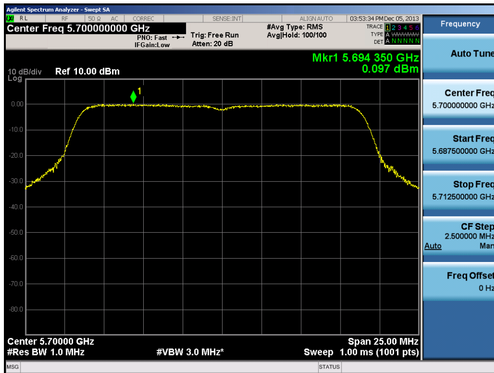
Plot 6-51. Peak Power Spectral Density Plot (20MHz BW 802.11n Ch. 140)
