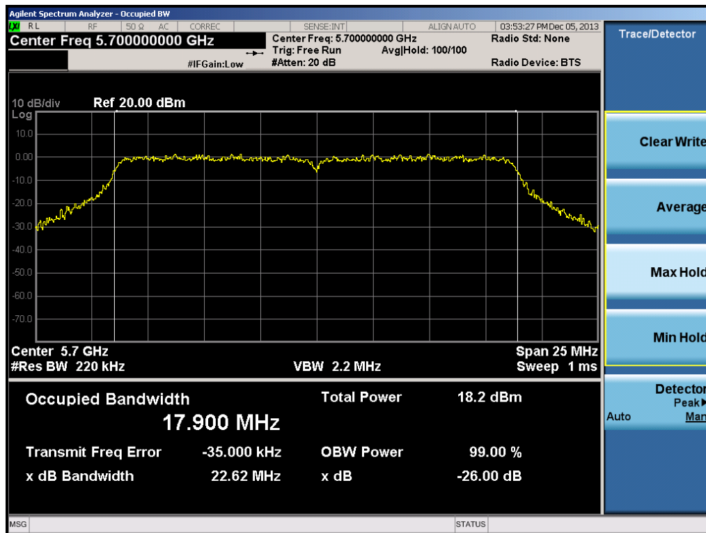
Plot 6-22. 26dB Bandwidth Plot (20MHz BW 802.11n Ch. 140)
