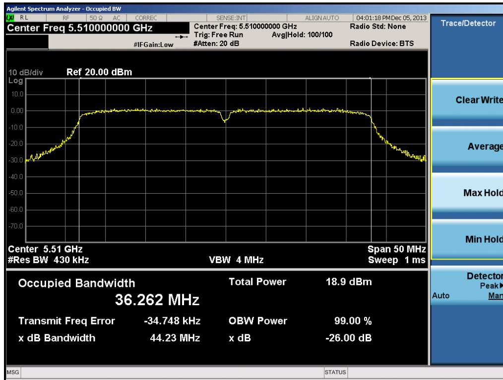
Plot 6-23. 26dB Bandwidth Plot (40MHz BW 802.11n Ch. 102)
