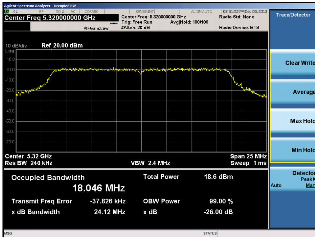
Plot 6-14. 26dB Bandwidth Plot (20MHz BW 802.11n Ch. 64)
