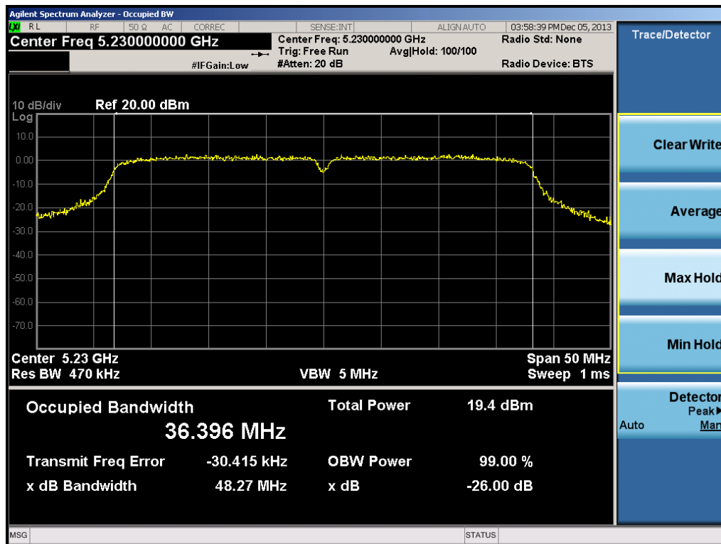
Plot 6-8. 26dB Bandwidth Plot (40MHz BW 802.11n Ch. 46)
