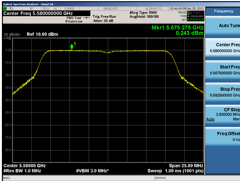
Plot 6-47. Peak Power Spectral Density Plot (802.11a Ch. 116)
