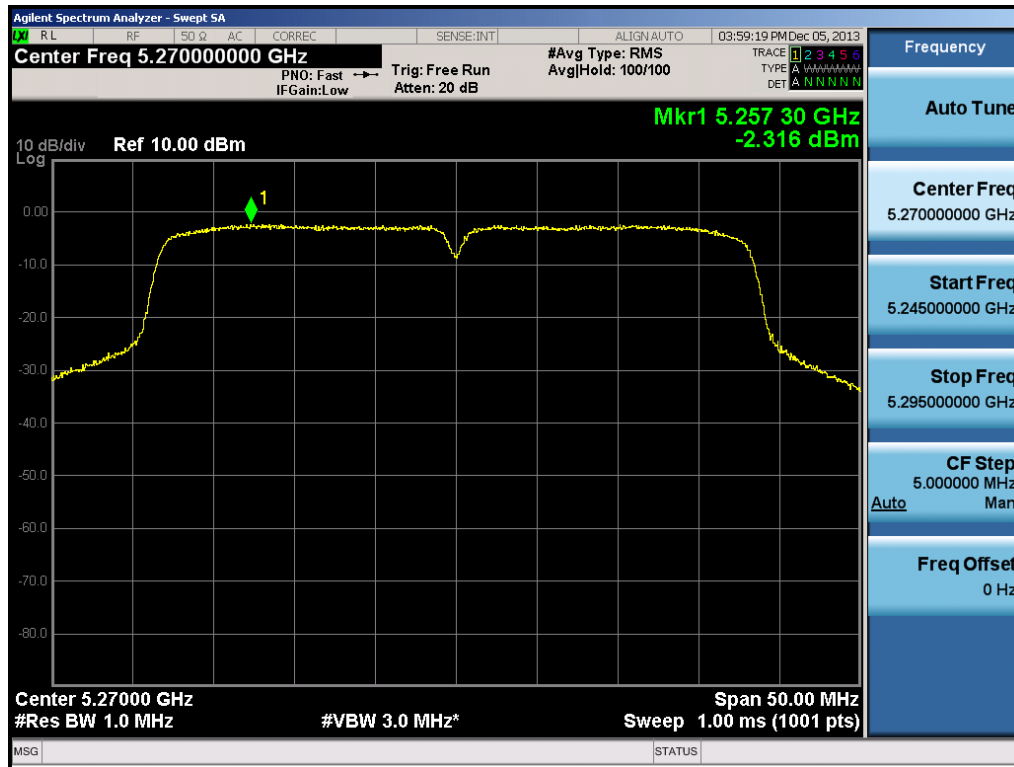
Plot 6-44. Peak Power Spectral Density Plot (40MHz BW 802.11n Ch. 54)
