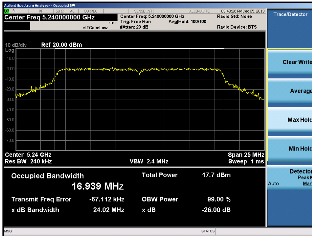
Plot 6-3. 26dB Bandwidth Plot (802.11a (Ch. 48))
