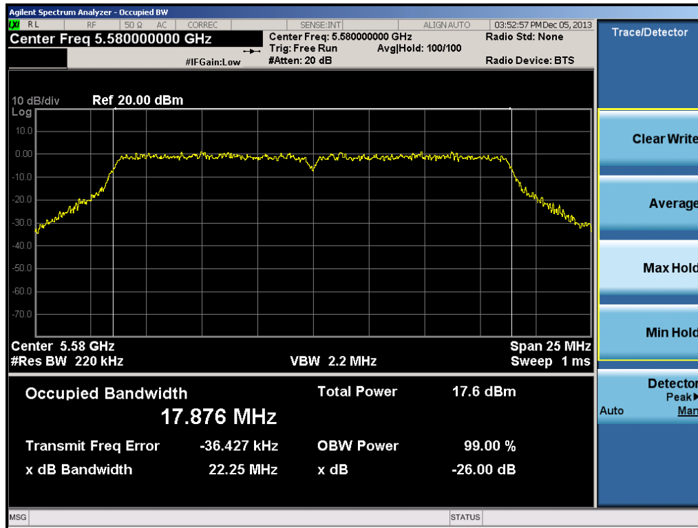
Plot 6-21. 26dB Bandwidth Plot (20MHz BW 802.11n Ch. 116)
