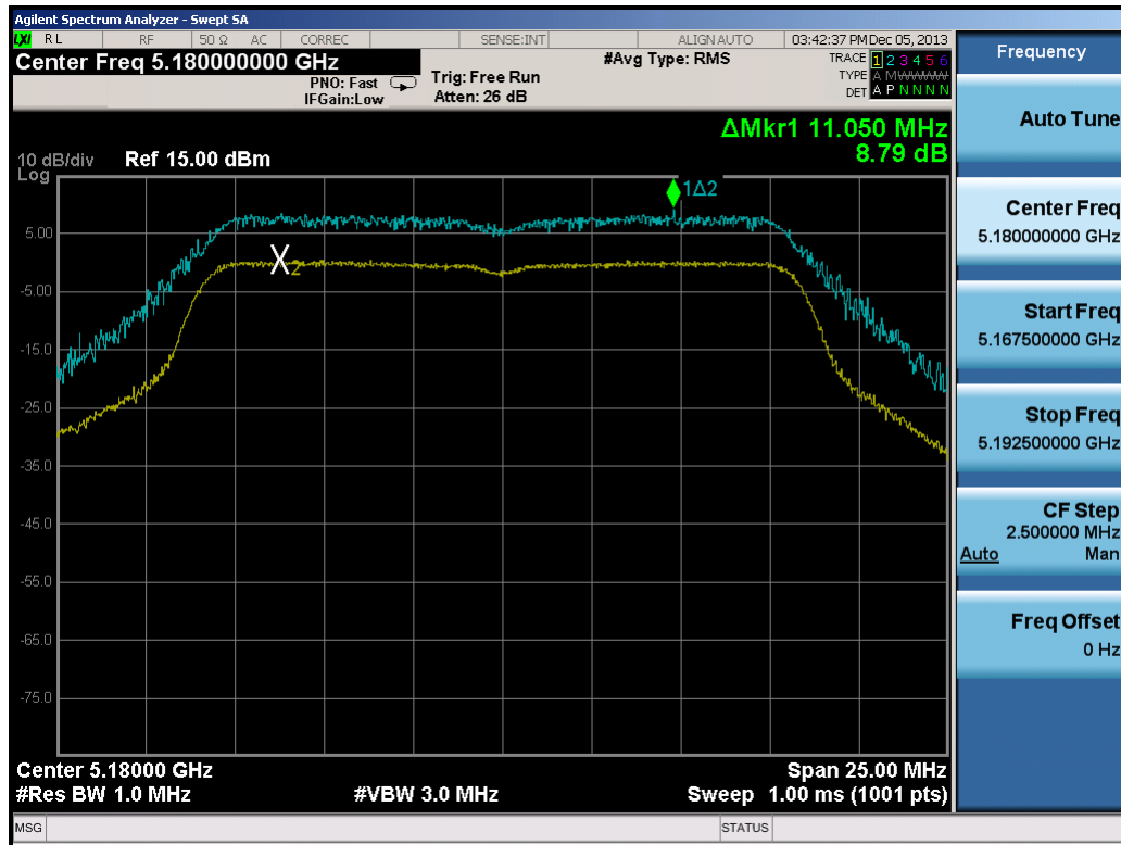
Plot 6-55. Peak Excursion Ratio Plot (802.11a)
