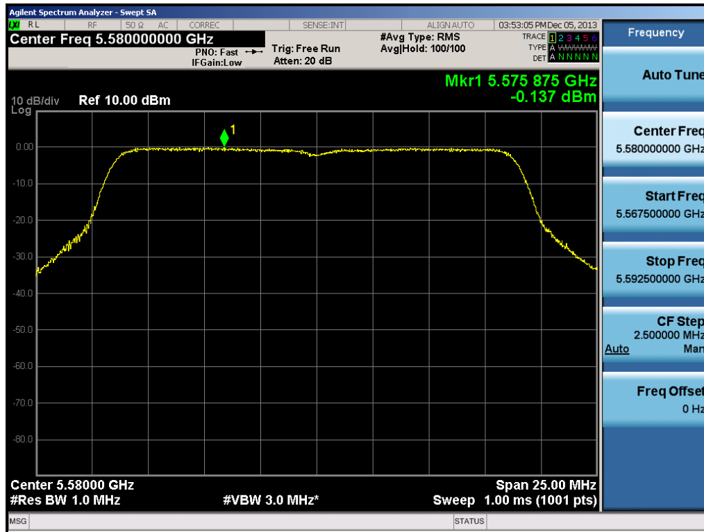
Plot 6-50. Peak Power Spectral Density Plot (20MHz BW 802.11n Ch. 116)
