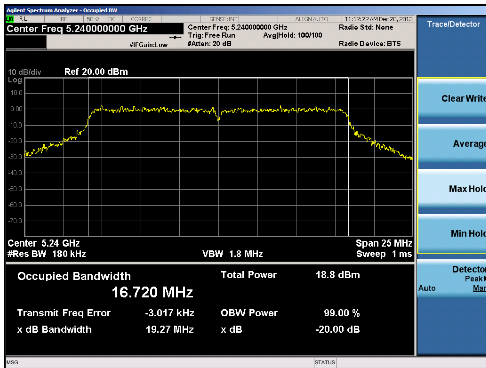
Plot 6-26. 20dB Bandwidth Plot (20MHz BW 802.11a Ch. 48)
