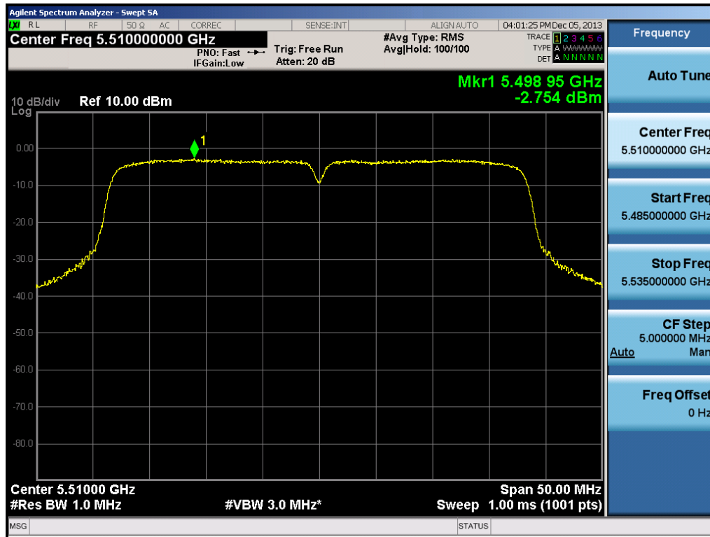
Plot 6-52. Peak Power Spectral Density Plot (40MHz BW 802.11n Ch. 102)
