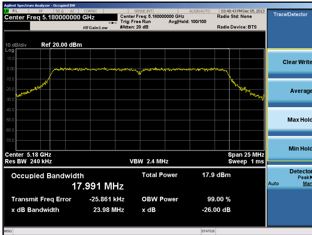
Plot 6-4. 26dB Bandwidth Plot (20MHz BW 802.11n Ch. 36)
