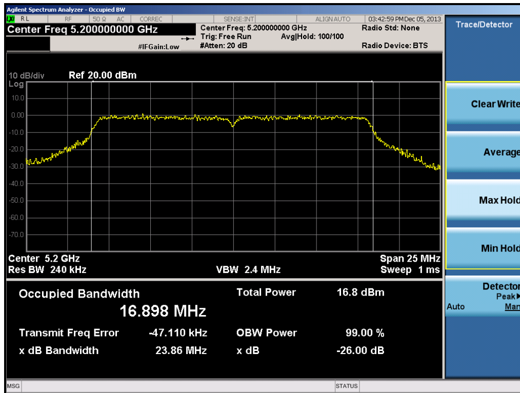
Plot 6-2. 26dB Bandwidth Plot (802.11a Ch. 40)
