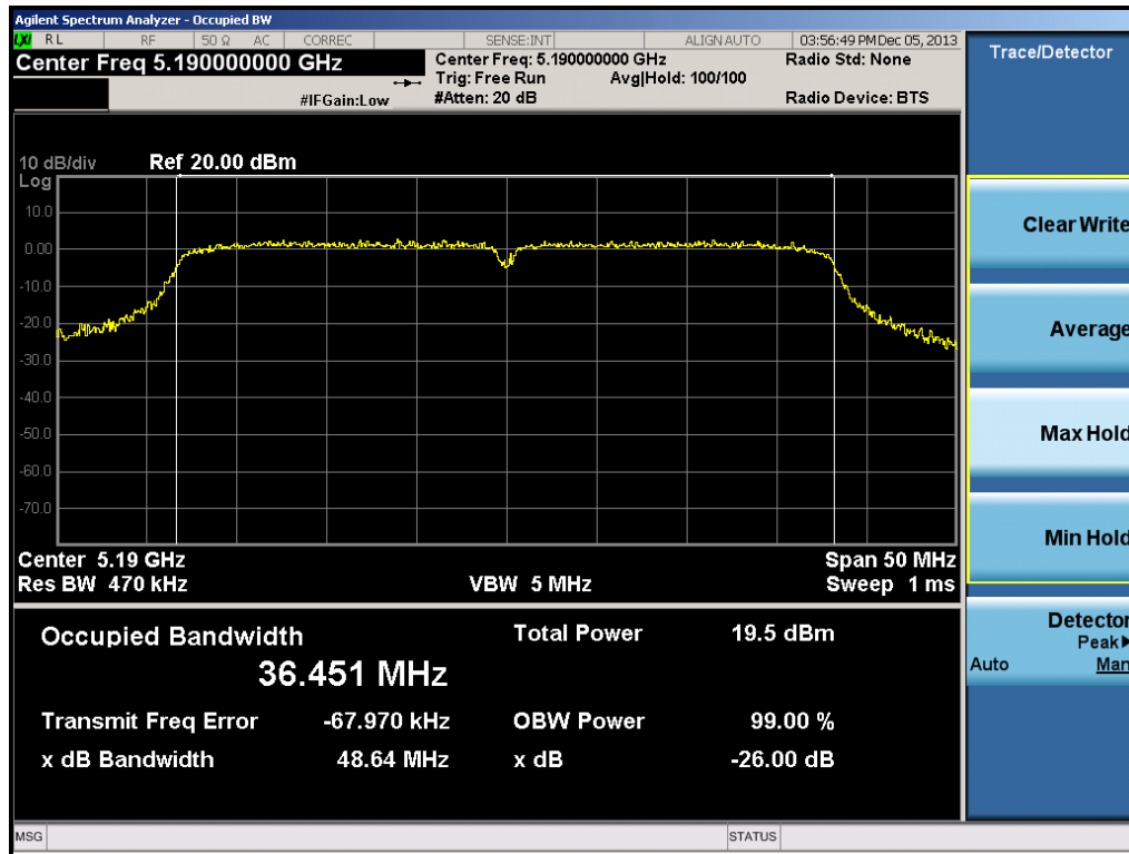
Plot 6-7. 26dB Bandwidth Plot (40MHz BW 802.11n Ch. 38)
