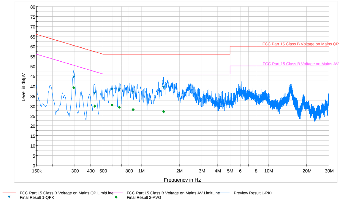
Plot 6-76. Line Conducted Plot with 802.11a UNII Band 2c (L1)
