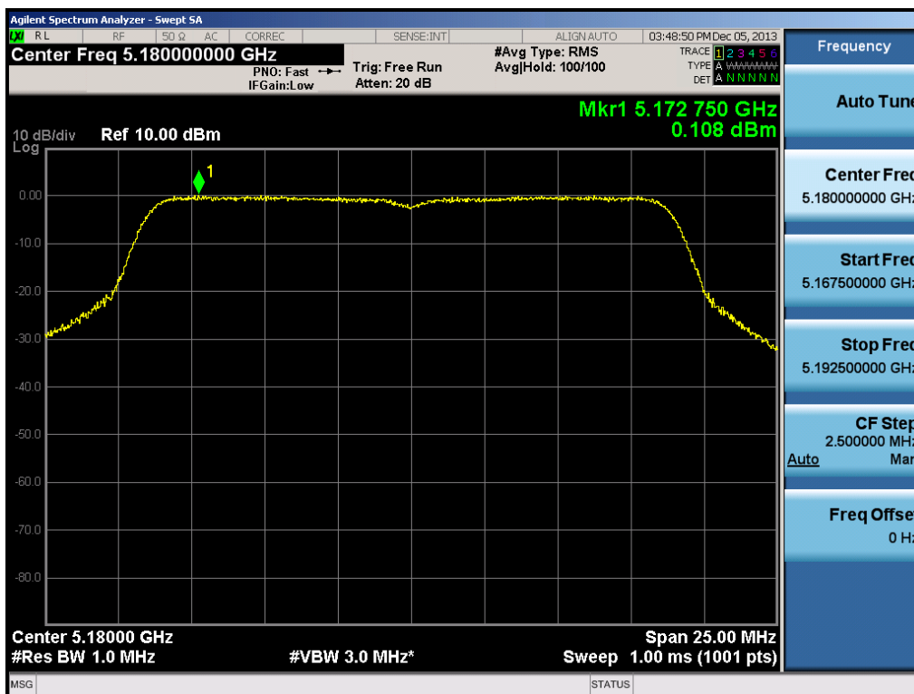
Plot 6-33. Peak Power Spectral Density Plot (20MHz BW 802.11n Ch. 36)
