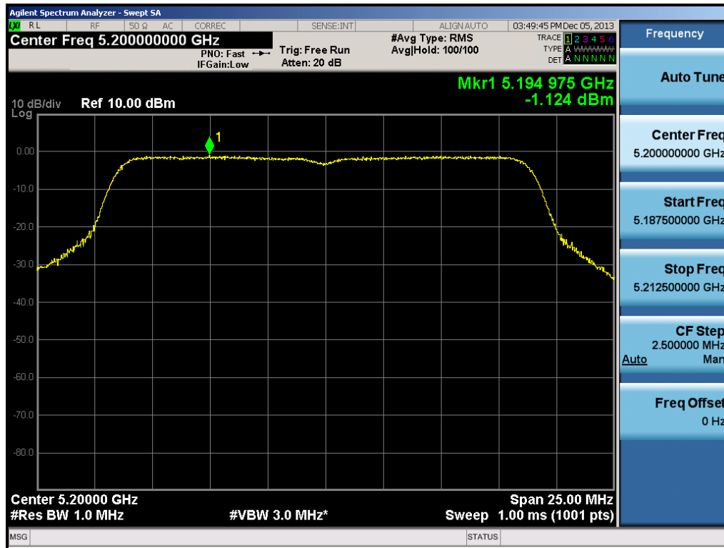
Plot 6-34. Peak Power Spectral Density Plot (20MHz BW 802.11n Ch. 40)
