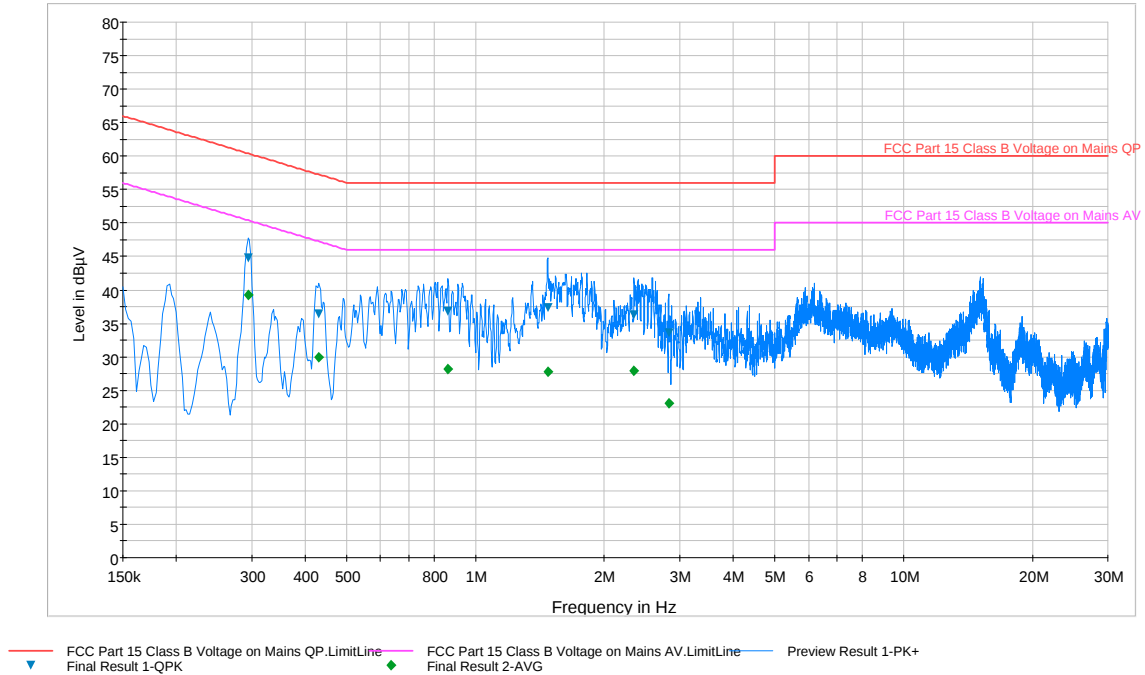
Plot 6-74. Line Conducted Plot with 802.11a UNII Band 2a (L1)
