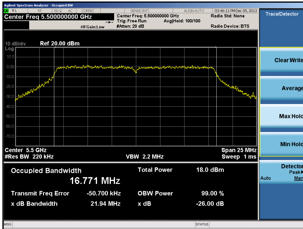
Plot 6-17. 26dB Bandwidth Plot (802.11a Ch. 100)
