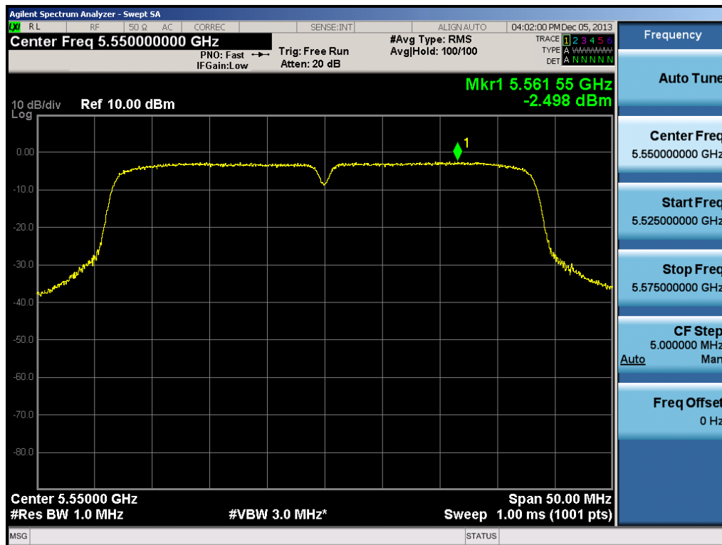
Plot 6-53. Peak Power Spectral Density Plot (40MHz BW 802.11n Ch. 110)
