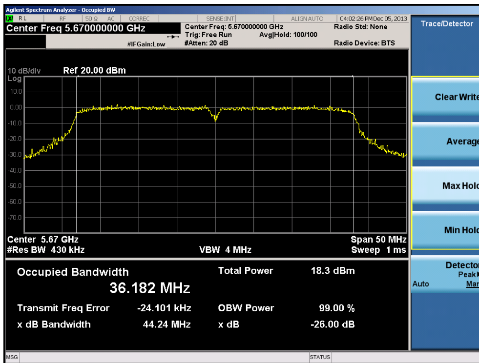
Plot 6-25. 26dB Bandwidth Plot (40MHz BW 802.11n Ch. 134)
