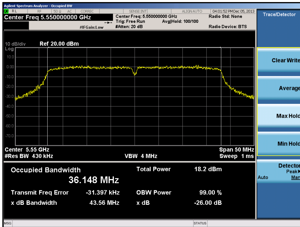
Plot 6-24. 26dB Bandwidth Plot (40MHz BW 802.11n Ch. 110)
