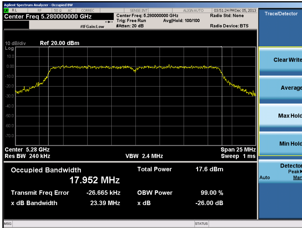
Plot 6-13. 26dB Bandwidth Plot (20MHz BW 802.11n Ch. 56)
