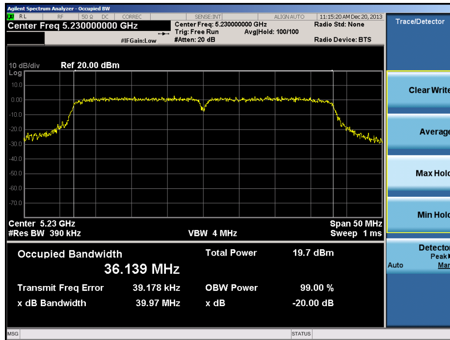
Plot 6-27. 20dB Bandwidth Plot (40MHz BW 802.11n Ch. 46)
