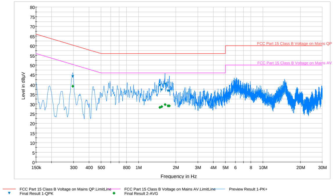
Plot 6-77. Line Conducted Plot with 802.11a UNII Band 2c (N)
