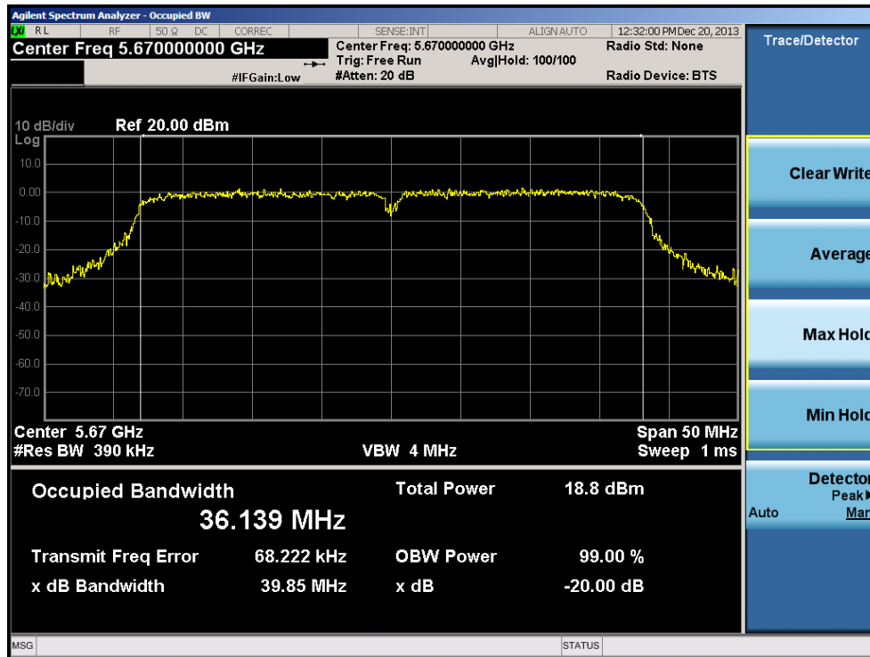
Plot 6-29. 20dB Bandwidth Plot (40MHz BW 802.11n Ch. 134)
