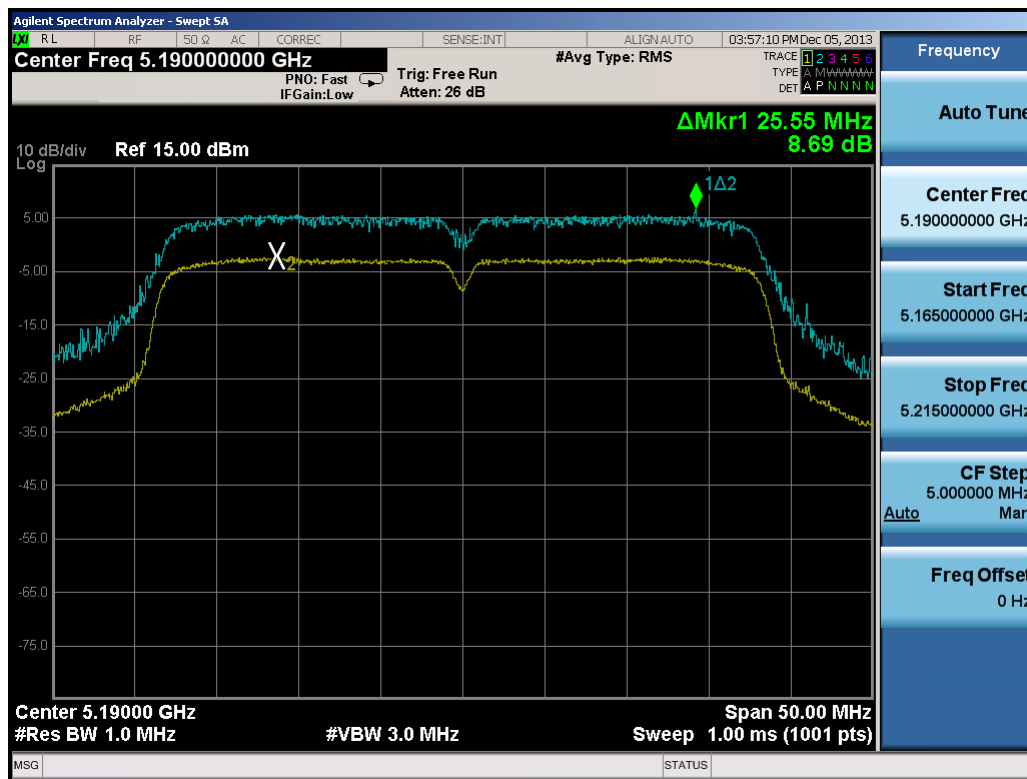
Plot 6-57. Peak Excursion Ratio Plot (40MHz BW 802.11n)
