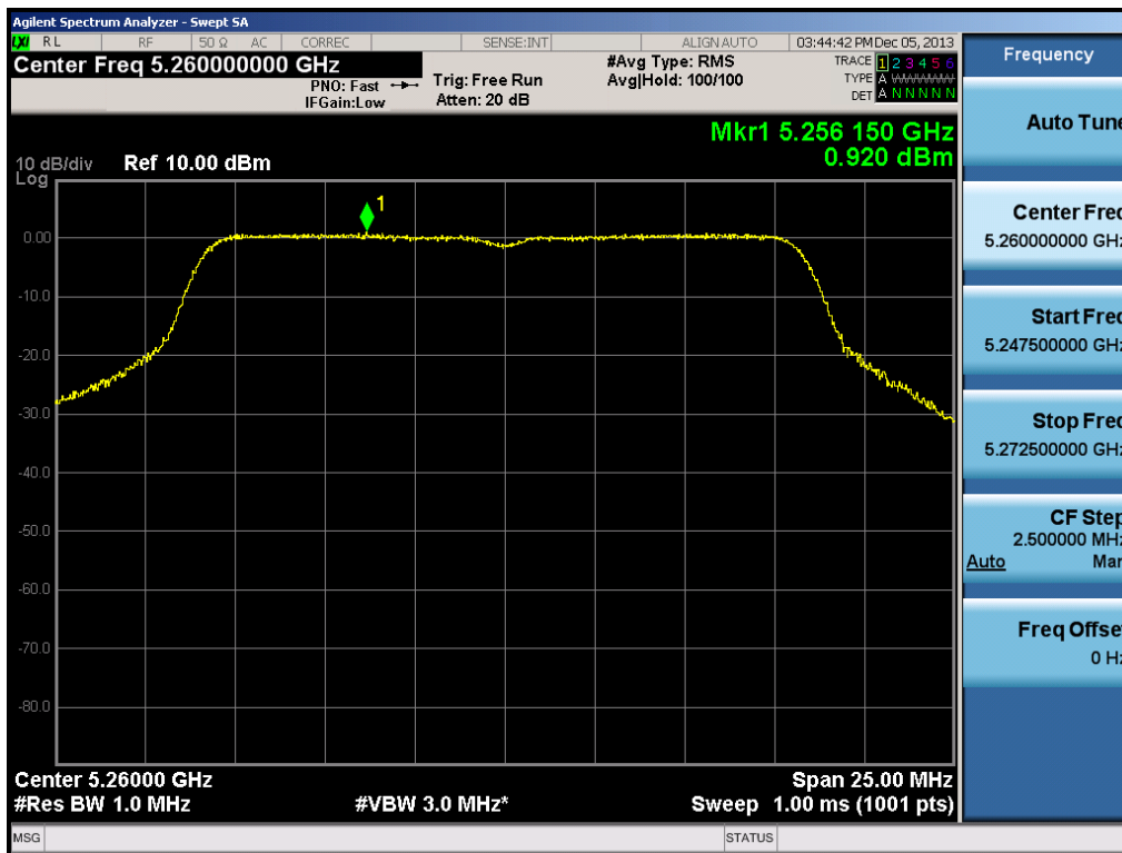
Plot 6-38. Peak Power Spectral Density Plot (802.11a Ch. 52)
