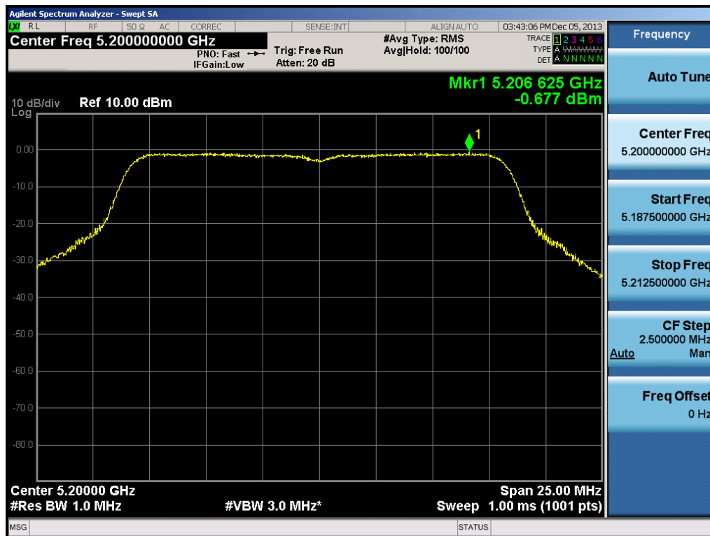
Plot 6-31. Peak Power Spectral Density Plot (802.11a Ch. 40)
