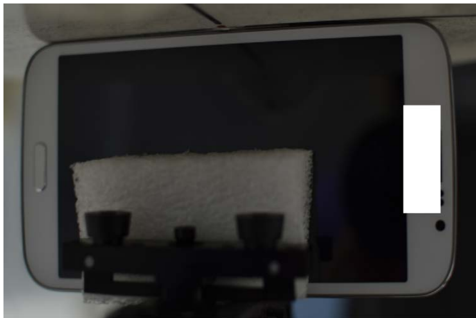
SAR Test Setup Photo 12 – Left Edge at 0.0 cm
