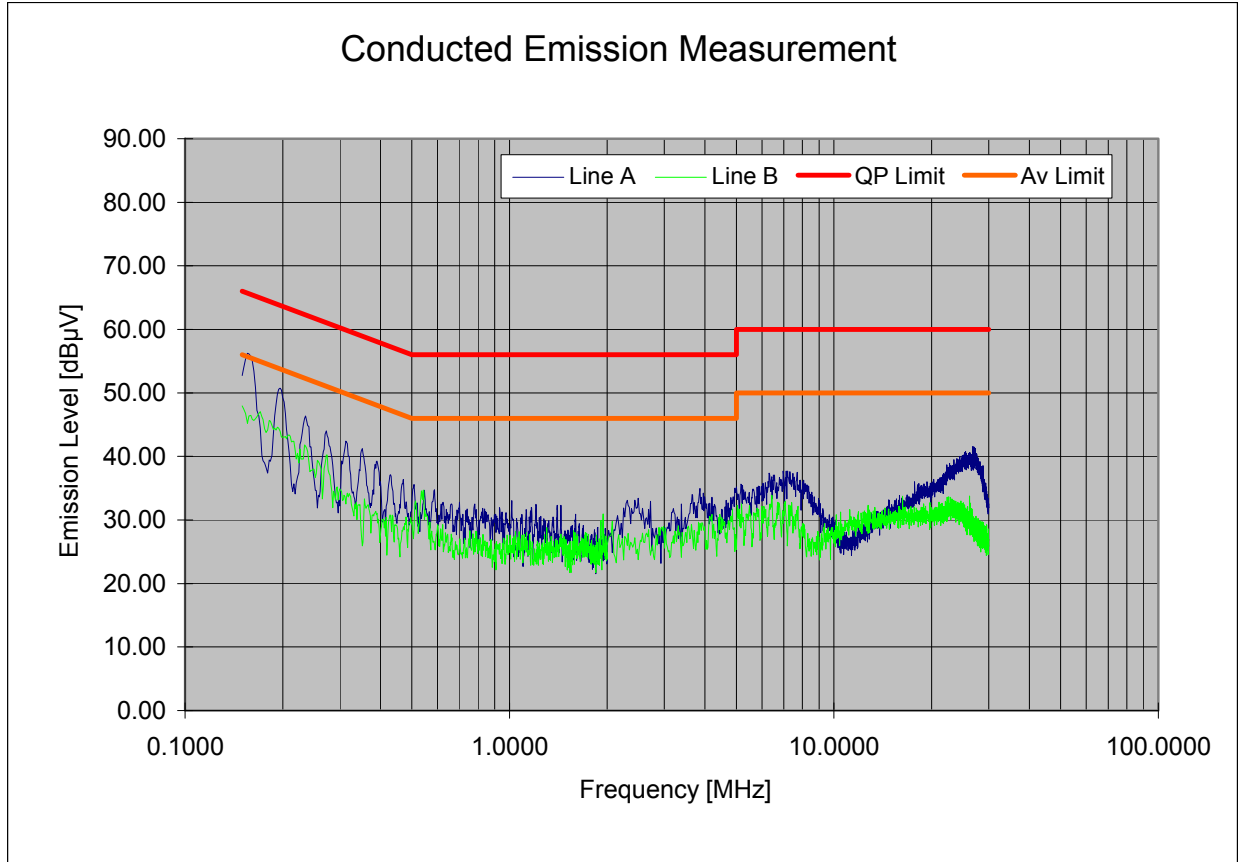
Plot 6-18. Line Conducted Plot with Bluetooth (LE)
