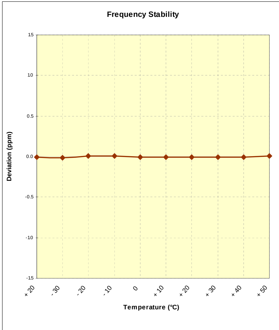
Figure 6-1. Frequency Stability Graph (PCS GSM Mode – Ch. 661)
