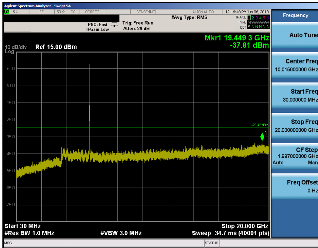
Plot 6-57. Conducted Spurious Plot (802.11a – Ch. 165)
