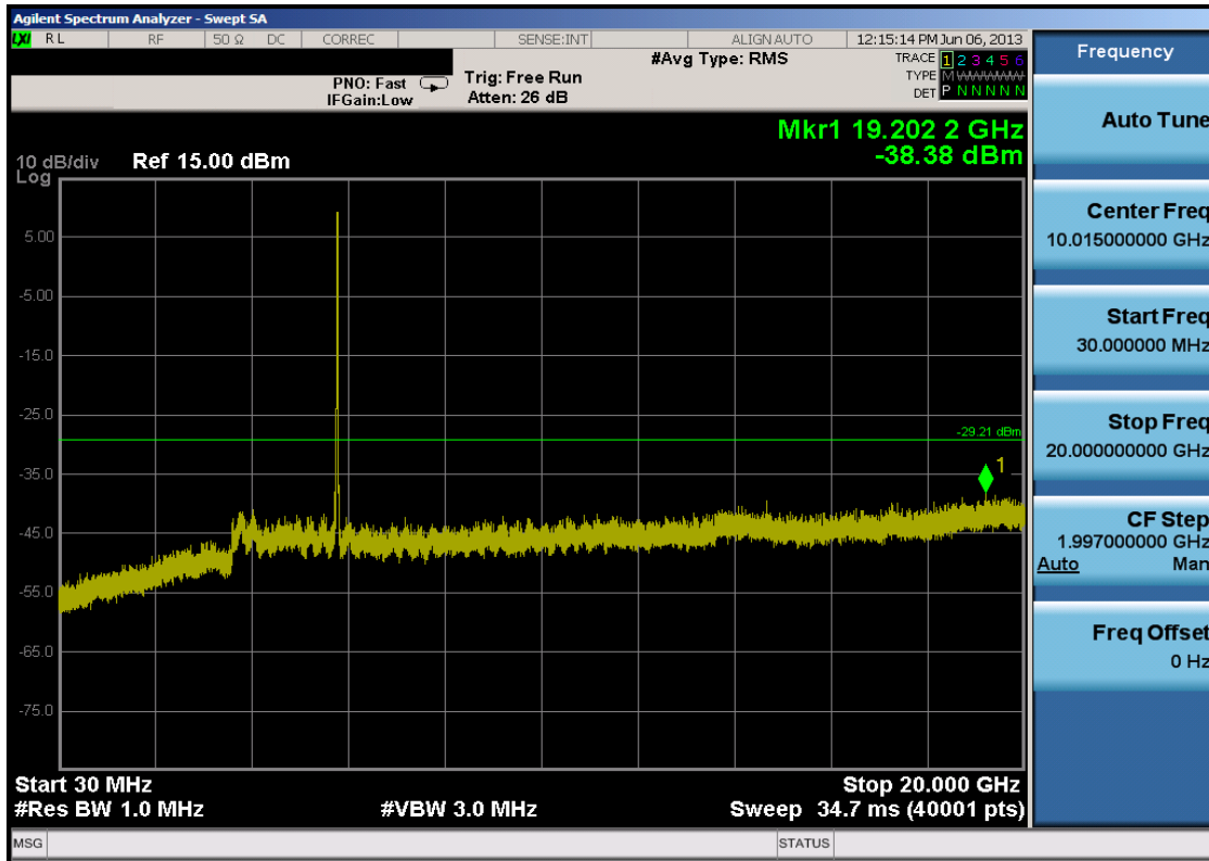
Plot 6-55. Conducted Spurious Plot (802.11a – Ch. 157)
