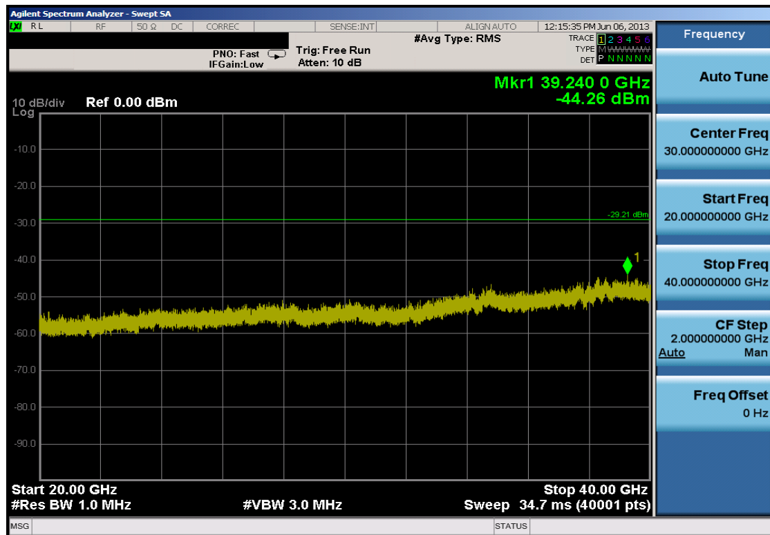
Plot 6-56. Conducted Spurious Plot (802.11a – Ch. 157)
