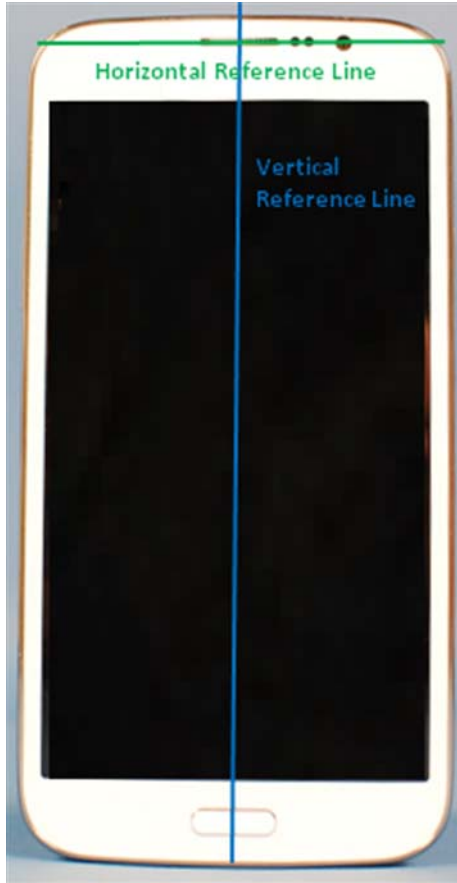
SAR Test Setup Photo 13: Vertical and Horizontal Reference Lines
