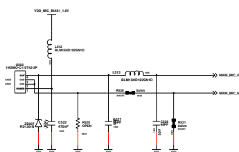
MAIN MIC
