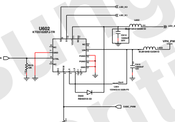
10 LED LCD DCDC
