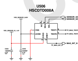
Magnetic Sensor
