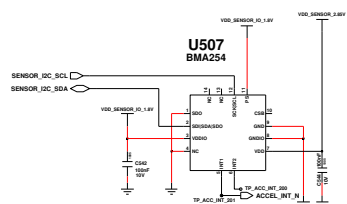
Accel. Sensor
