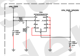
OVP for protecting Audio AMP AMR
