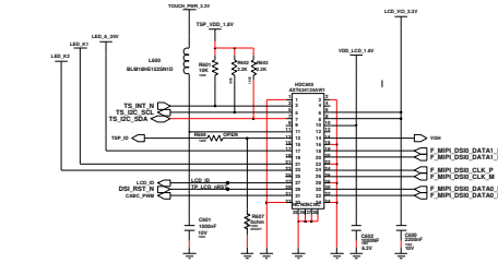
SMD LCD 5.8" QHD WITH TSP CON
