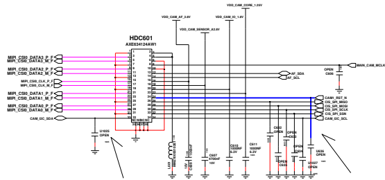
8M CAMERA
