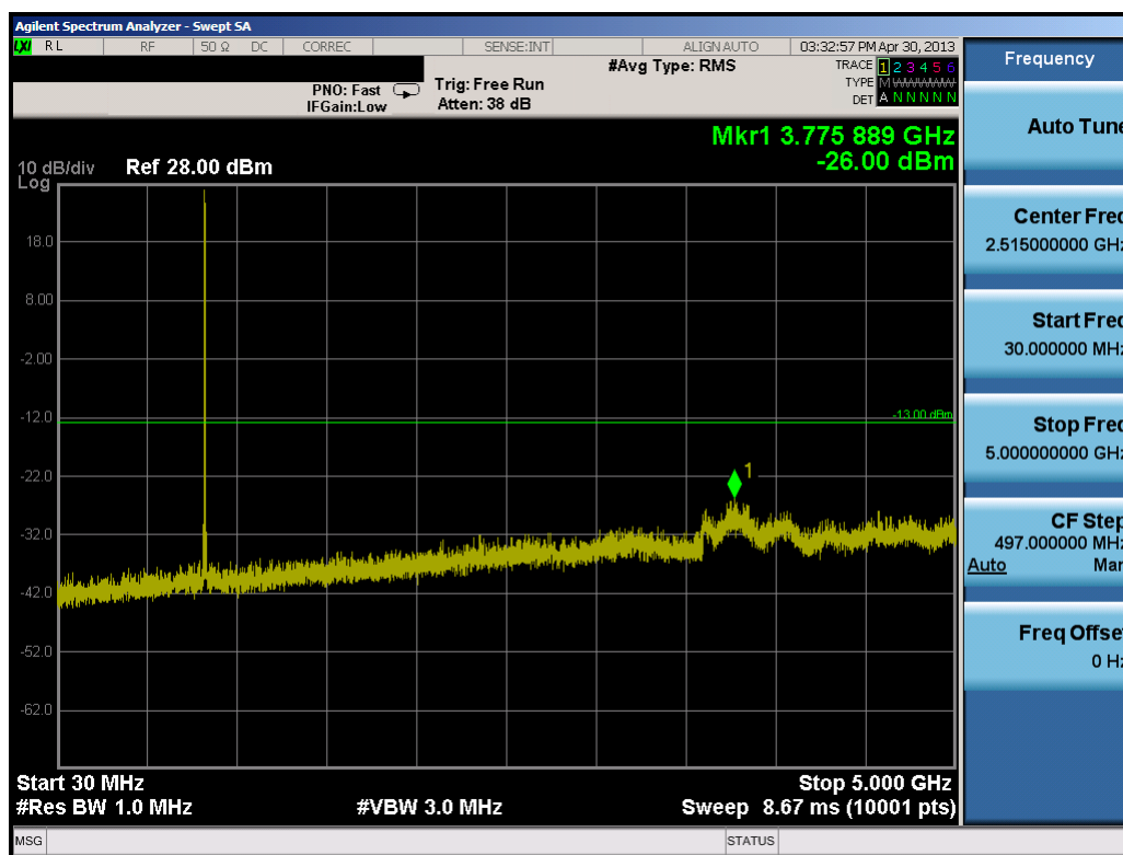
Plot 7-29. Conducted Spurious Plot (5.0MHz QPSK – RB Size 1, RB Offset 0 – High Channel)
