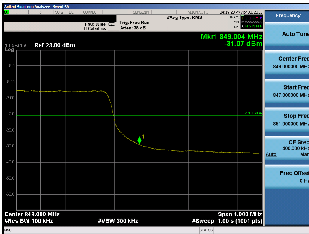
Plot 7-42. Upper Band Edge Plot (10.0MHz QPSK – RB Size 50)
