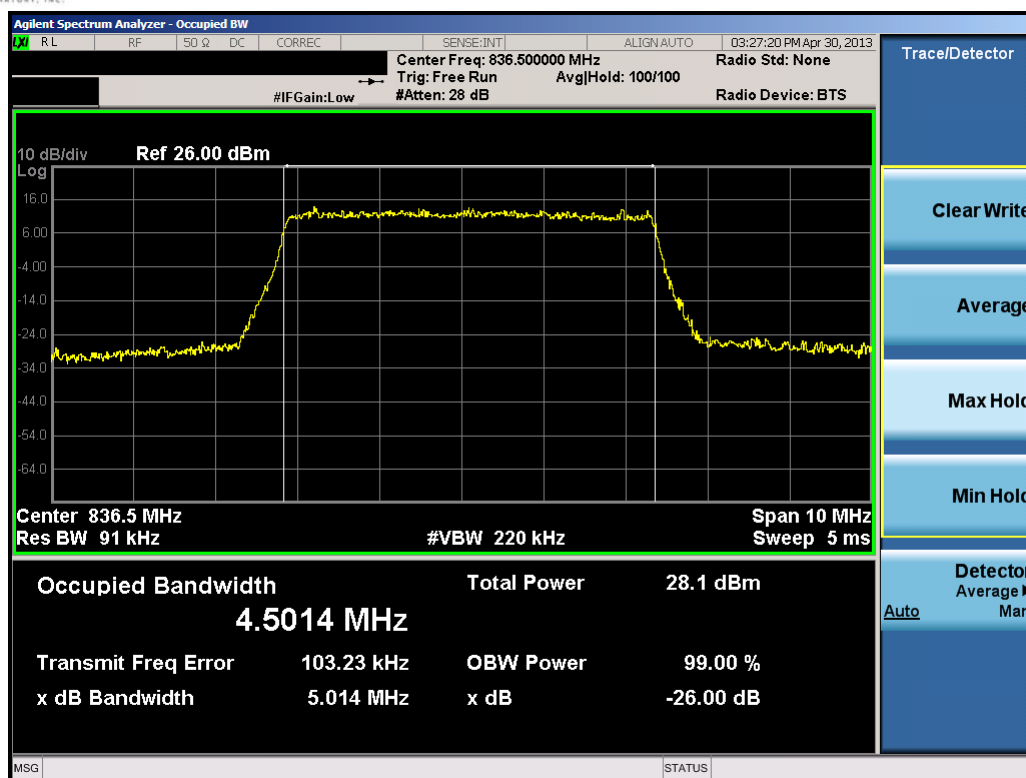
Plot 7-24. Occupied Bandwidth Plot (5.0MHz 16-QAM – RB Size 25)
