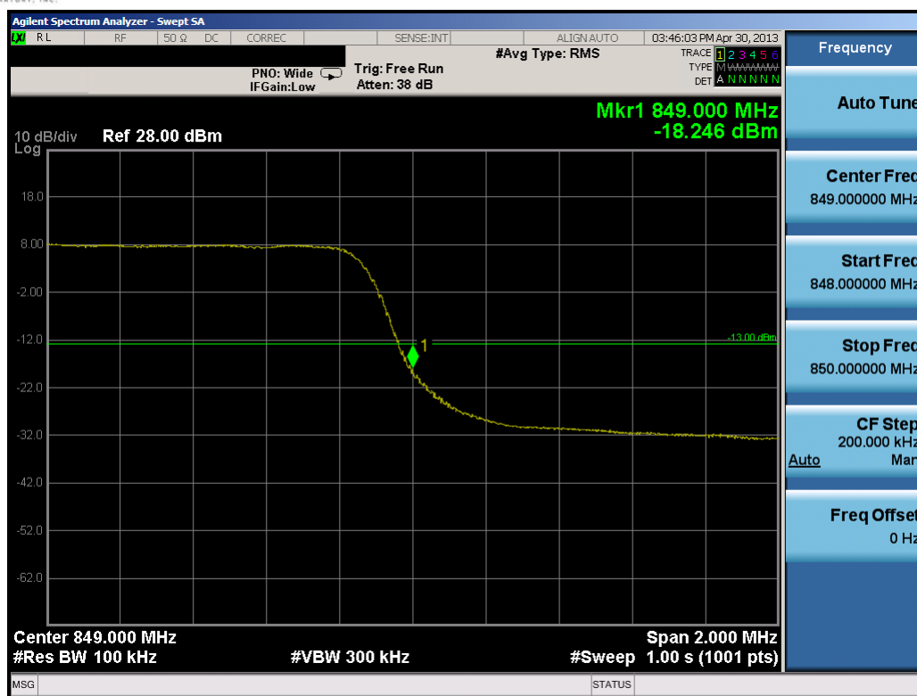
Plot 7-20. Upper Band Edge Plot (3.0MHz QPSK – RB Size 15)
