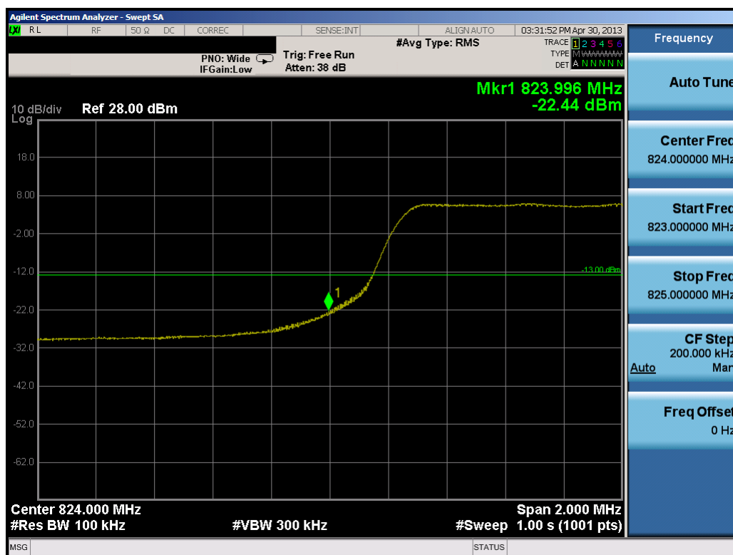
Plot 7-21. Lower Band Edge Plot (5.0MHz QPSK – RB Size 25)
