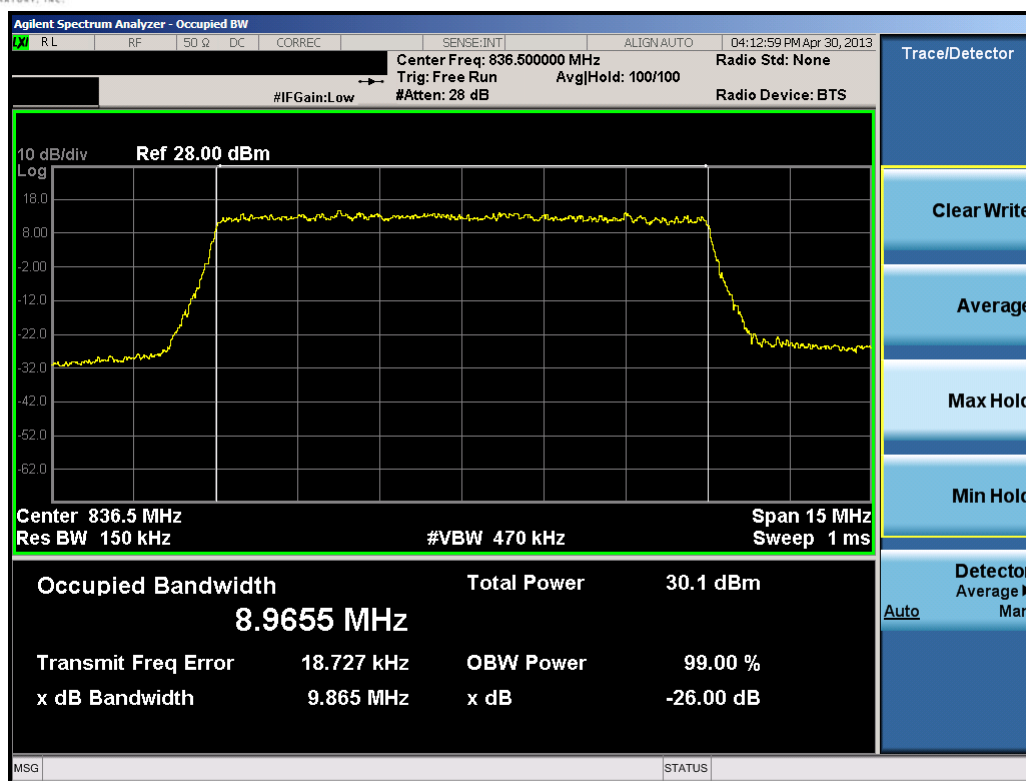
Plot 7-34. Occupied Bandwidth Plot (10.0MHz QPSK – RB Size 50)
