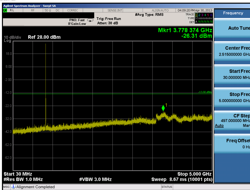
Plot 7-8. Conducted Spurious Plot (1.4MHz QPSK – RB Size 1, RB Offset 0 – High Channel)
