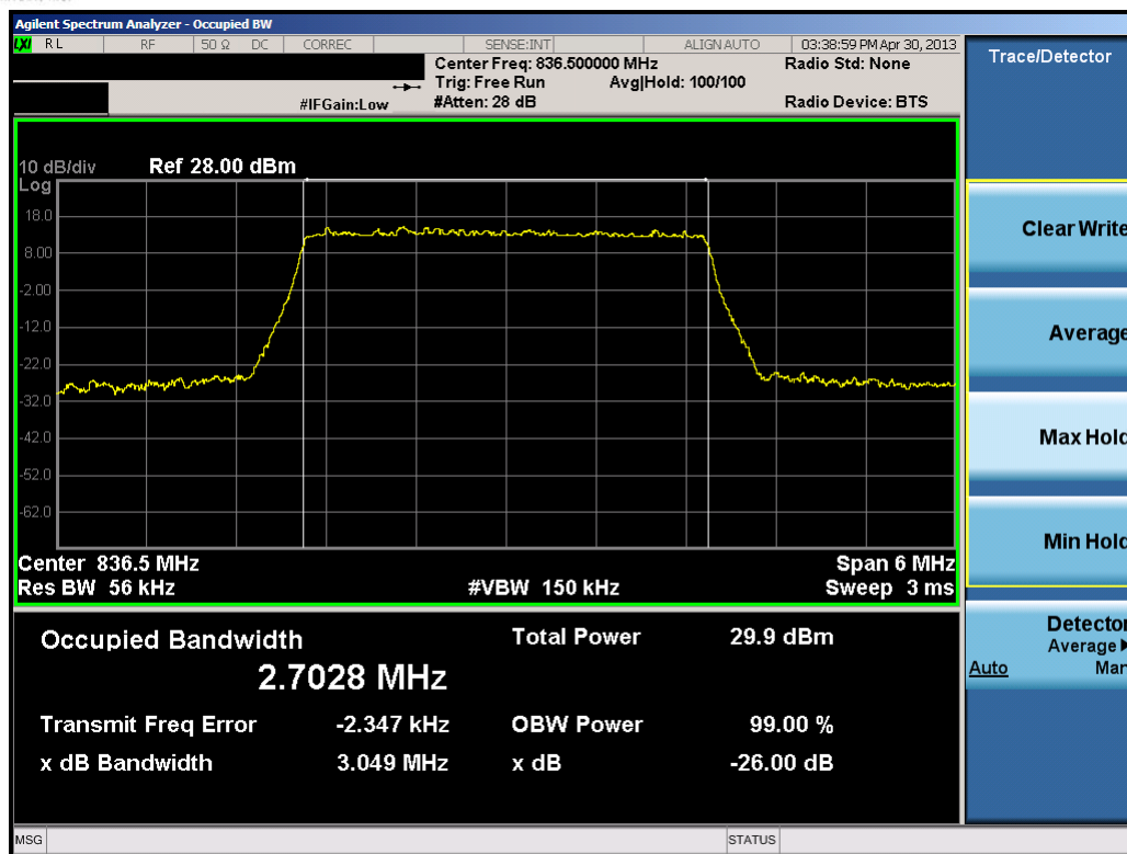
Plot 7-12. Occupied Bandwidth Plot (3.0MHz QPSK – RB Size 15)
