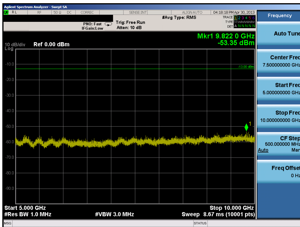
Plot 7-41. Conducted Spurious Plot (10.0MHz QPSK – RB Size 1, RB Offset 0 – High Channel)
