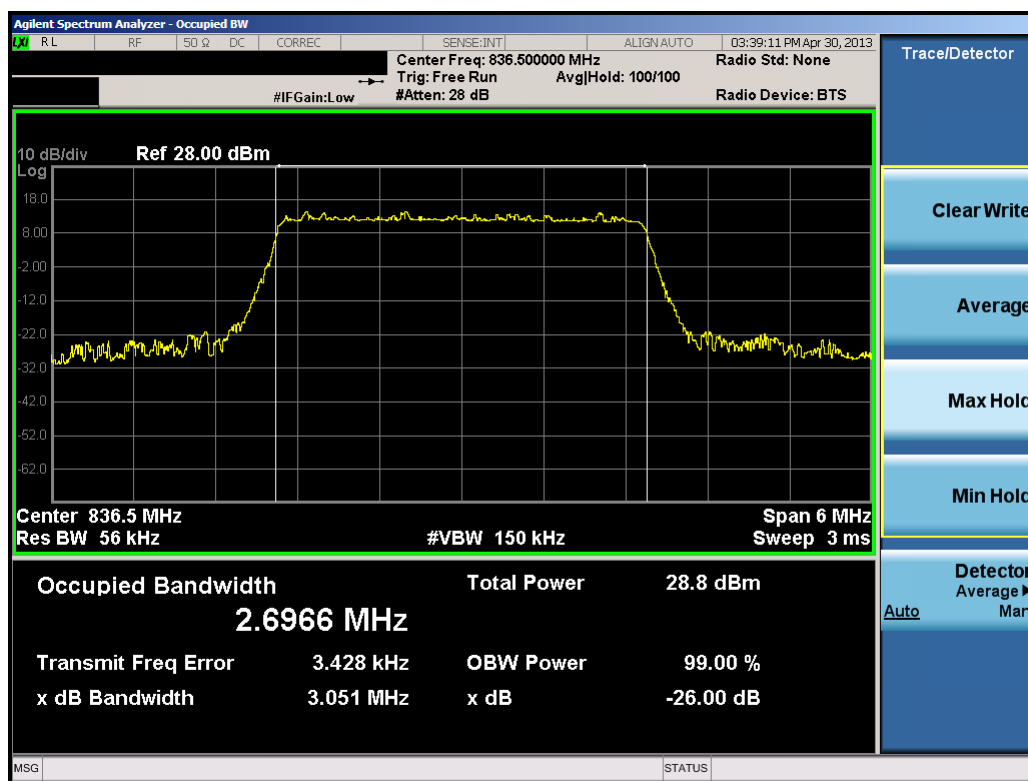
Plot 7-13. Occupied Bandwidth Plot (3.0MHz 16-QAM – RB Size 15)
