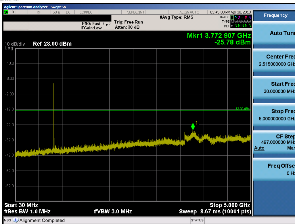
Plot 7-18. Conducted Spurious Plot (3.0MHz QPSK – RB Size 1, RB Offset 0 – High Channel)
