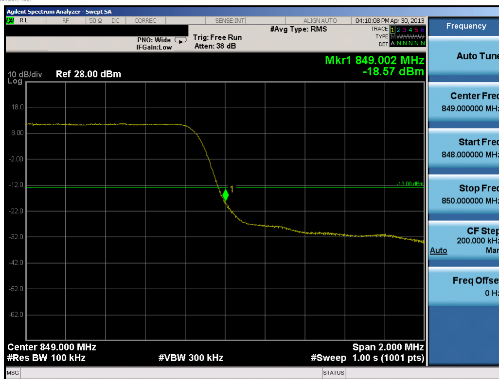
Plot 7-10. Upper Band Edge Plot (1.4MHz QPSK – RB Size 6)
