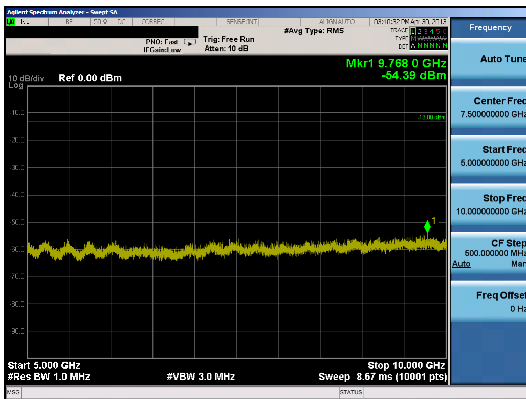
Plot 7-17. Conducted Spurious Plot (3.0MHz QPSK – RB Size 1, RB Offset 0 – Mid Channel)
