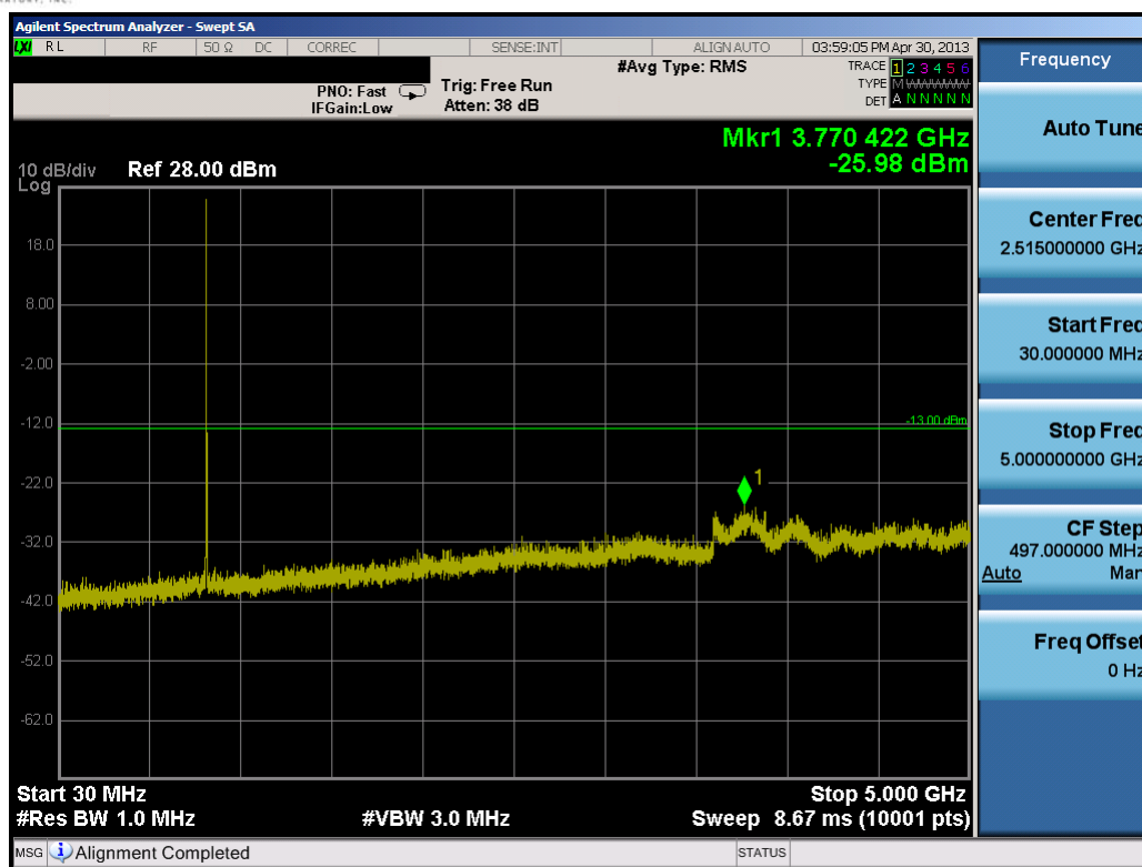
Plot 7-6. Conducted Spurious Plot (1.4MHz QPSK – RB Size 1, RB Offset 0 – Mid Channel)
