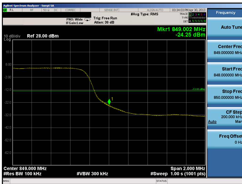
Plot 7-31. Upper Band Edge Plot (5.0MHz QPSK – RB Size 25)
