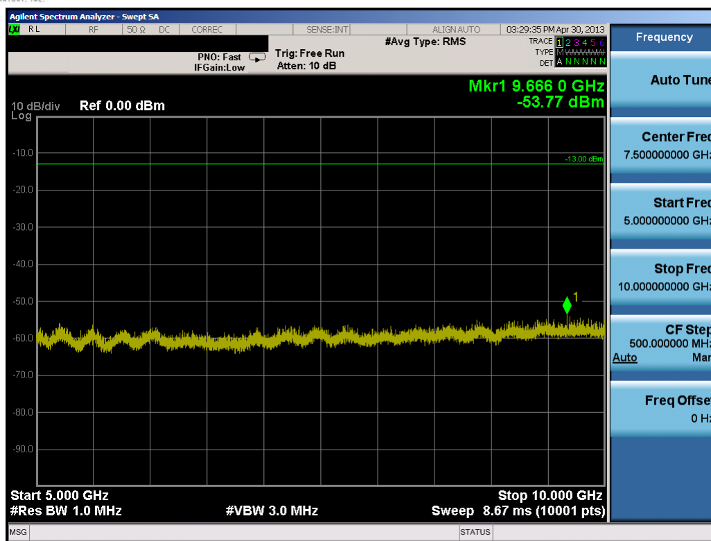
Plot 7-28. Conducted Spurious Plot (5.0MHz QPSK – RB Size 1, RB Offset 0 – Mid Channel)
