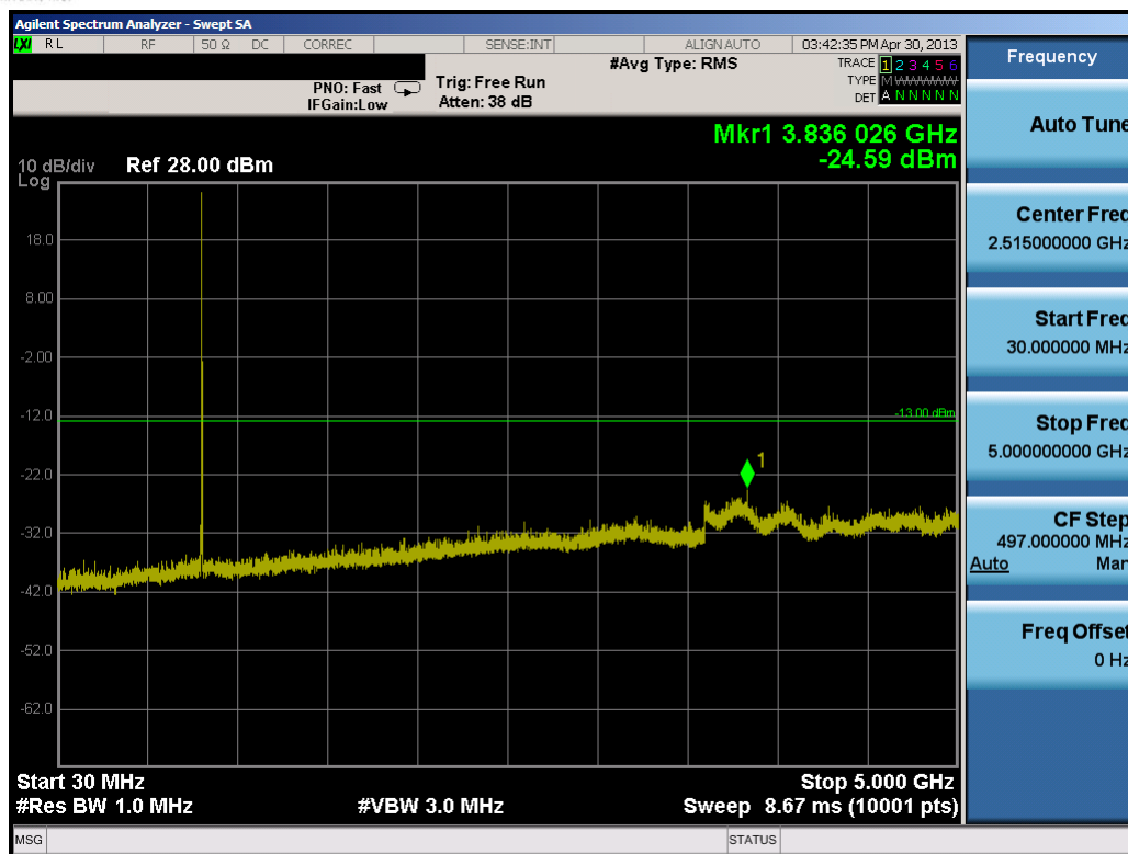
Plot 7-14. Conducted Spurious Plot (3.0MHz QPSK – RB Size 1, RB Offset 0 – Low Channel)
