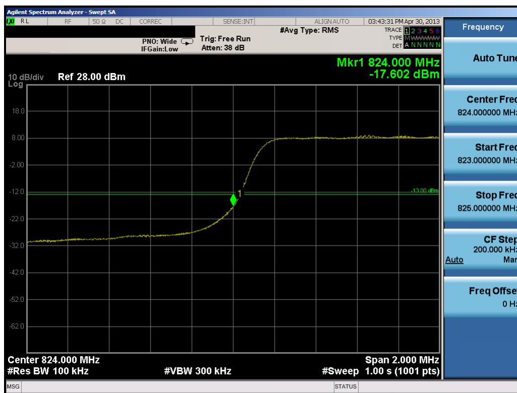
Plot 7-11. Lower Band Edge Plot (3.0MHz QPSK – RB Size 15)
