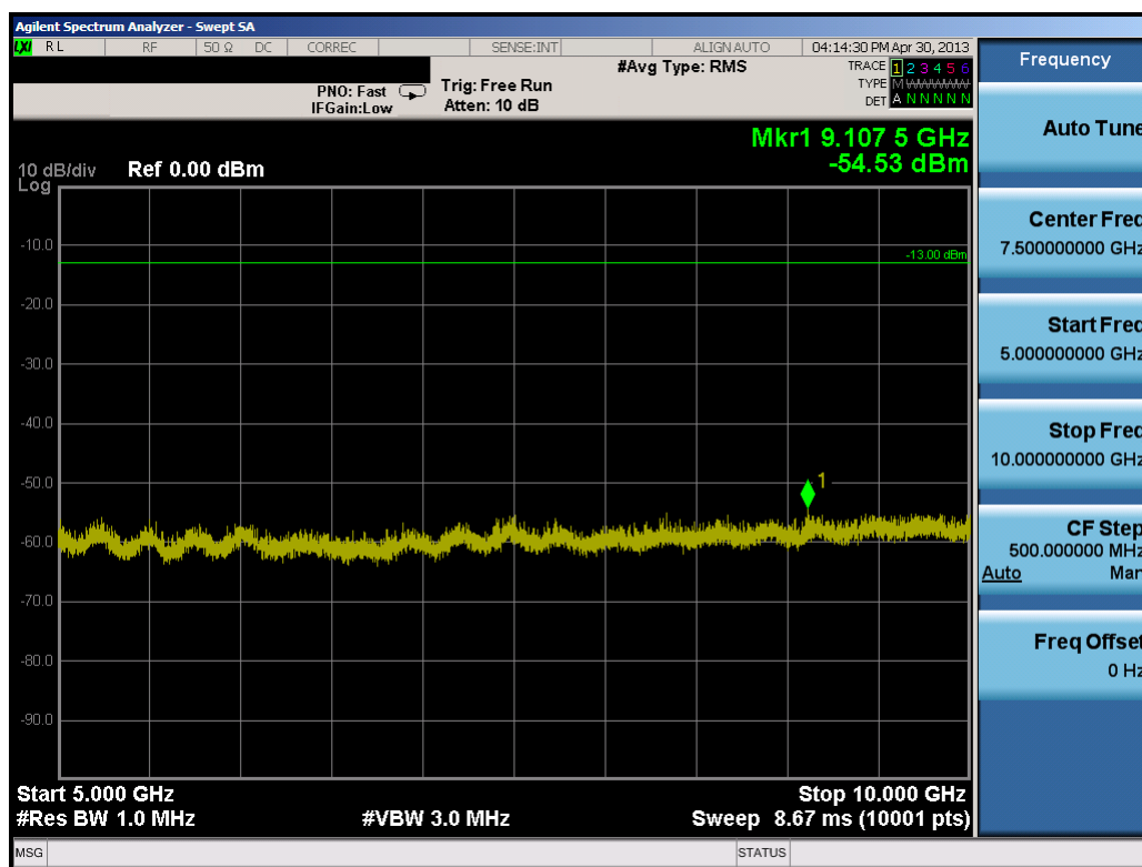
Plot 7-39. Conducted Spurious Plot (10.0MHz QPSK – RB Size 1, RB Offset 0 – Mid Channel)
