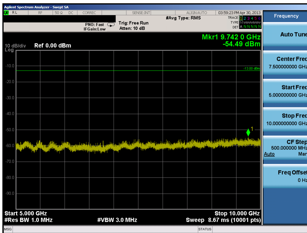
Plot 7-7. Conducted Spurious Plot (1.4MHz QPSK – RB Size 1, RB Offset 0 – Mid Channel)
