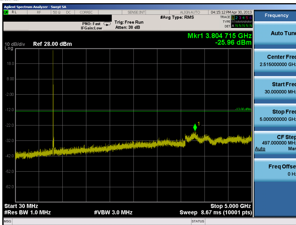
Plot 7-36. Conducted Spurious Plot (10.0MHz QPSK – RB Size 1, RB Offset 0– Low Channel)
