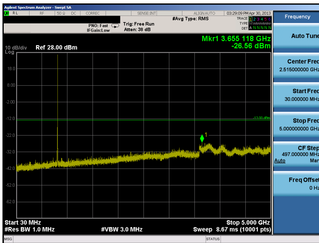
Plot 7-27. Conducted Spurious Plot (5.0MHz QPSK – RB Size 1, RB Offset 0 – Mid Channel)
