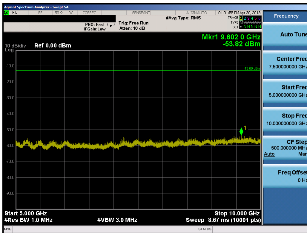
Plot 7-5. Conducted Spurious Plot (1.4MHz QPSK – RB Size 1, RB Offset 0 – Low Channel)
