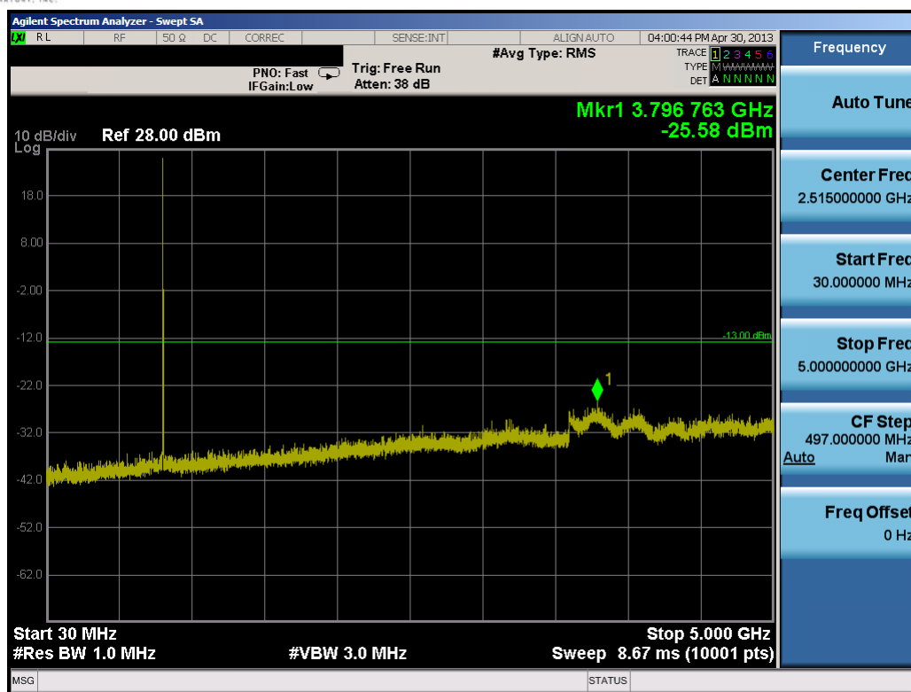
Plot 7-4. Conducted Spurious Plot (1.4MHz QPSK – RB Size 1, RB Offset 0 – Low Channel)
