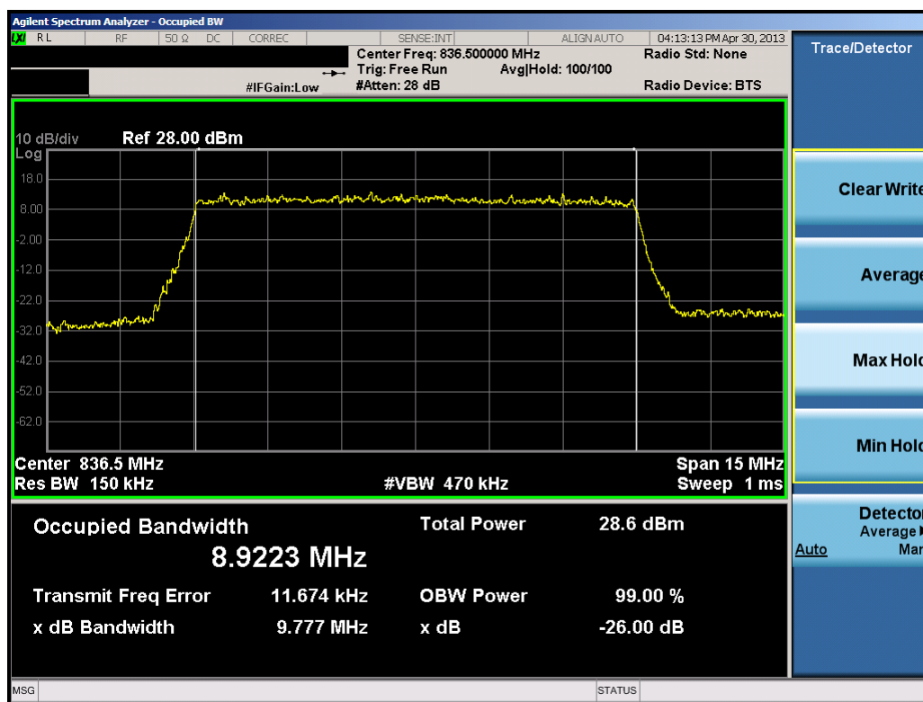
Plot 7-35. Occupied Bandwidth Plot (10.0MHz 16-QAM – RB Size 50)
