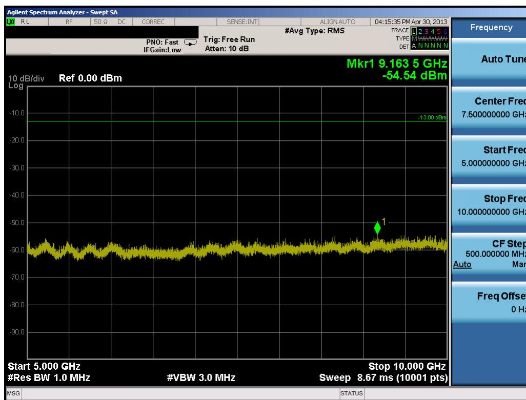
Plot 7-37. Conducted Spurious Plot (10.0MHz QPSK – RB Size 1, RB Offset 0 – Low Channel)
