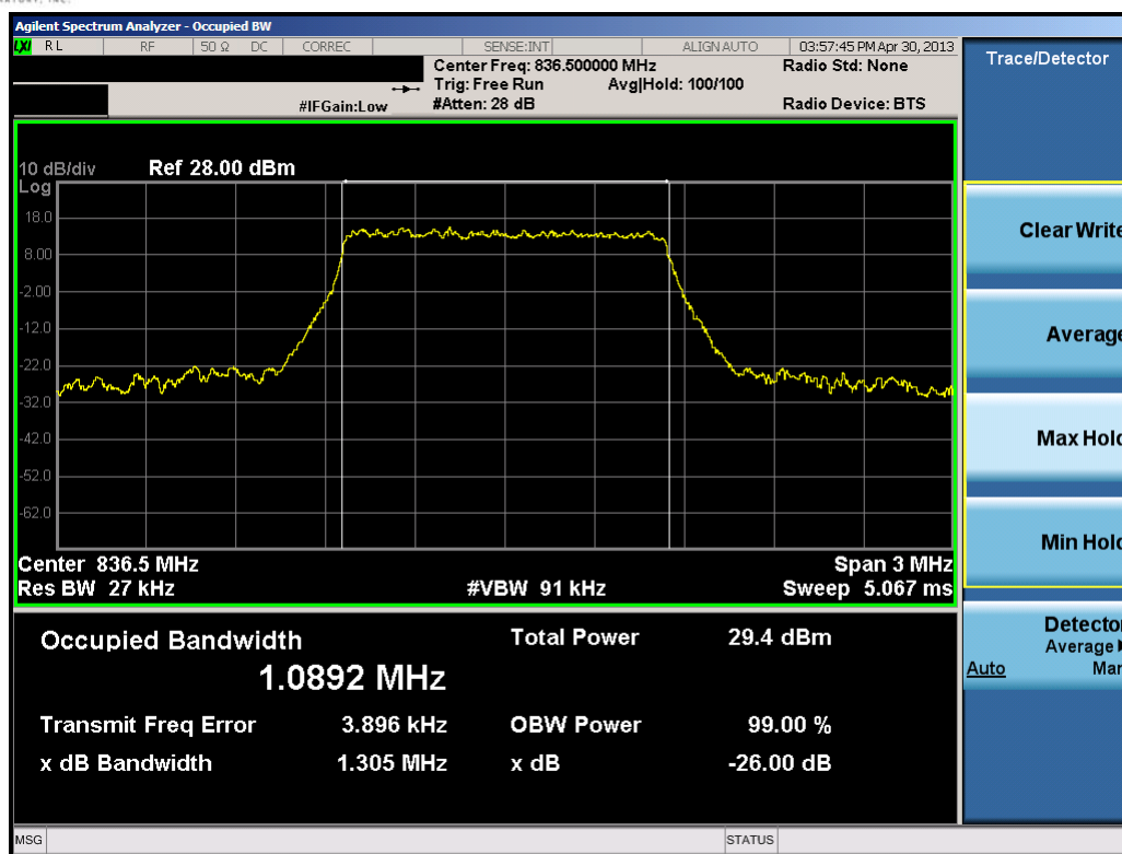
Plot 7-2. Occupied Bandwidth Plot (1.4MHz QPSK – RB Size 6)
