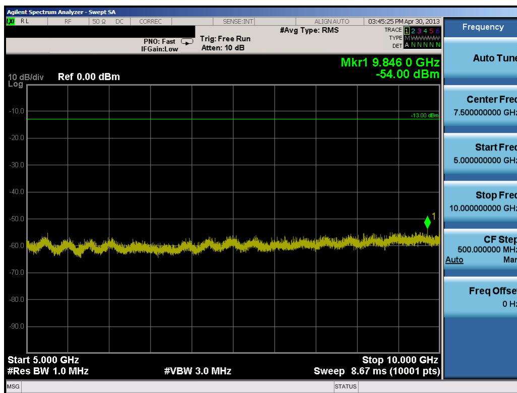
Plot 7-19. Conducted Spurious Plot (3.0MHz QPSK – RB Size 1, RB Offset 0 – High Channel)
