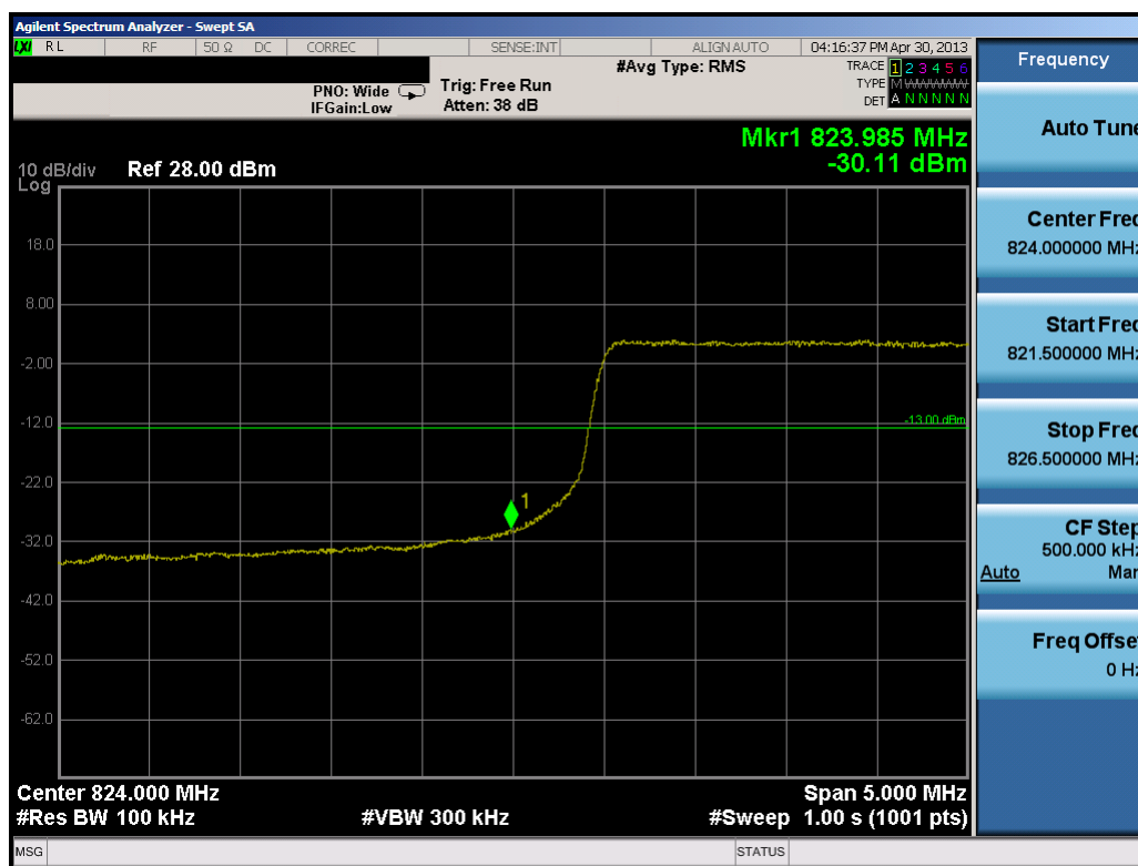
Plot 7-33. Lower Band Edge Plot (10.0MHz QPSK – RB Size 50)
