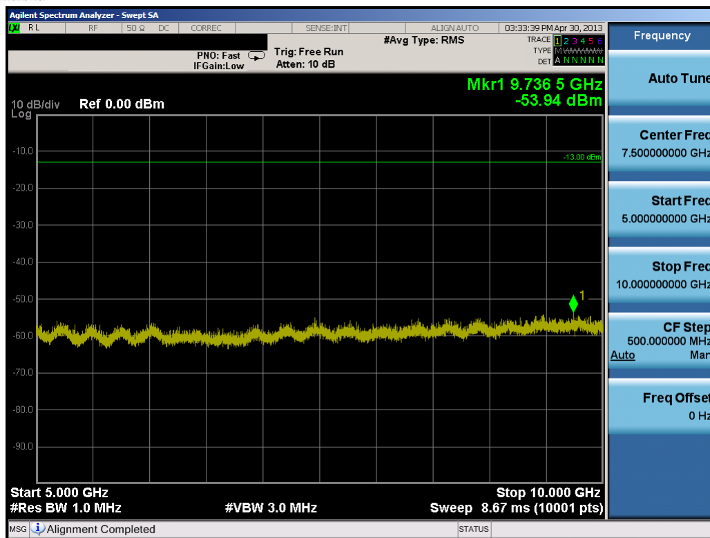
Plot 7-30. Conducted Spurious Plot (5.0MHz QPSK – RB Size 1, RB Offset 0 – High Channel)
