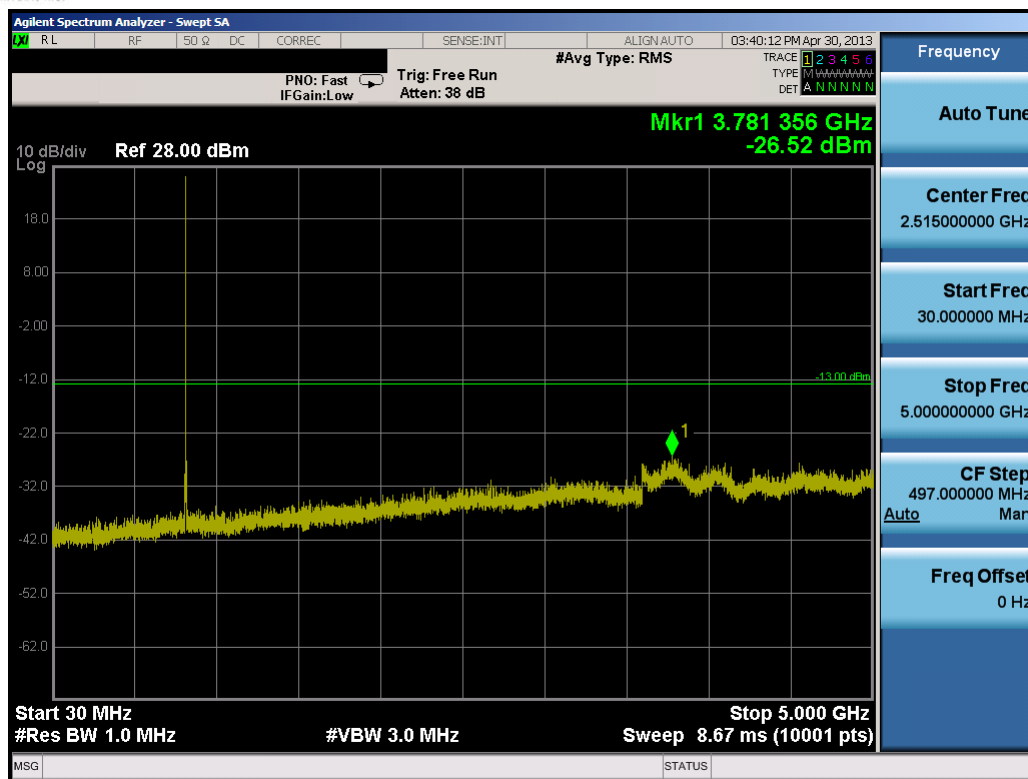
Plot 7-16. Conducted Spurious Plot (3.0MHz QPSK – RB Size 1, RB Offset 0 – Mid Channel)
