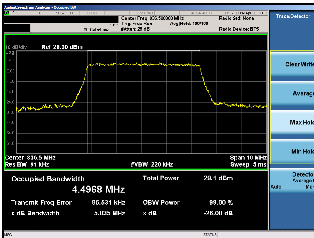
Plot 7-23. Occupied Bandwidth Plot (5.0MHz QPSK – RB Size 25)
