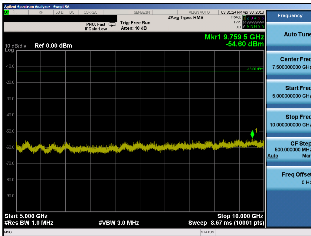
Plot 7-26. Conducted Spurious Plot (5.0MHz QPSK – RB Size 1, RB Offset 0 – Low Channel)
