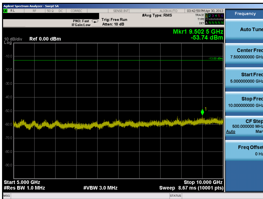
Plot 7-15. Conducted Spurious Plot (3.0MHz QPSK – RB Size 1, RB Offset 0 – Low Channel)
