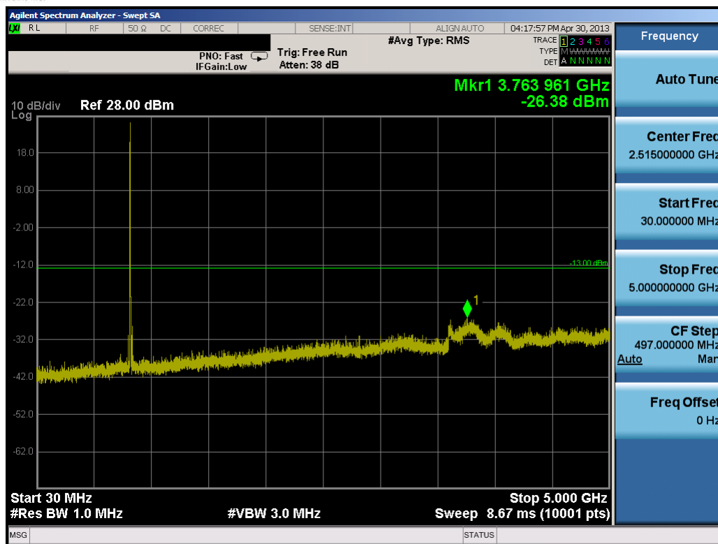
Plot 7-40. Conducted Spurious Plot (10.0MHz QPSK – RB Size 1, RB Offset 0 – High Channel)
