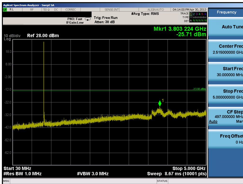
Plot 7-38. Conducted Spurious Plot (10.0MHz QPSK – RB Size 1, RB Offset 0 – Mid Channel)
