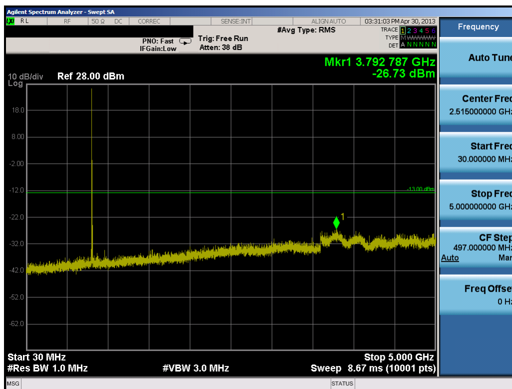
Plot 7-25. Conducted Spurious Plot (5.0MHz QPSK – RB Size 1, RB Offset 0 – Low Channel)
