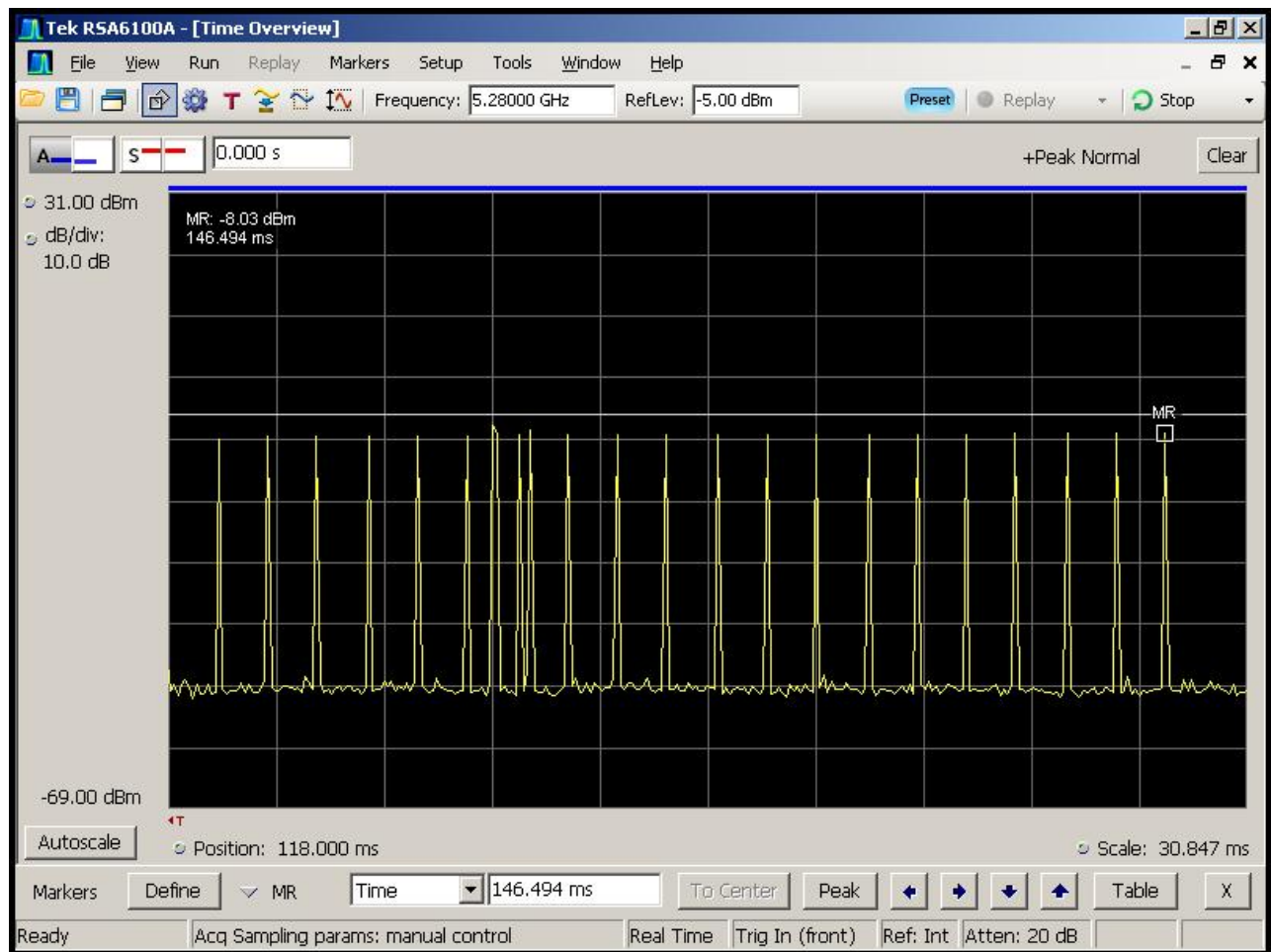
Figure 5-1. Type 1 Radar Pulse
