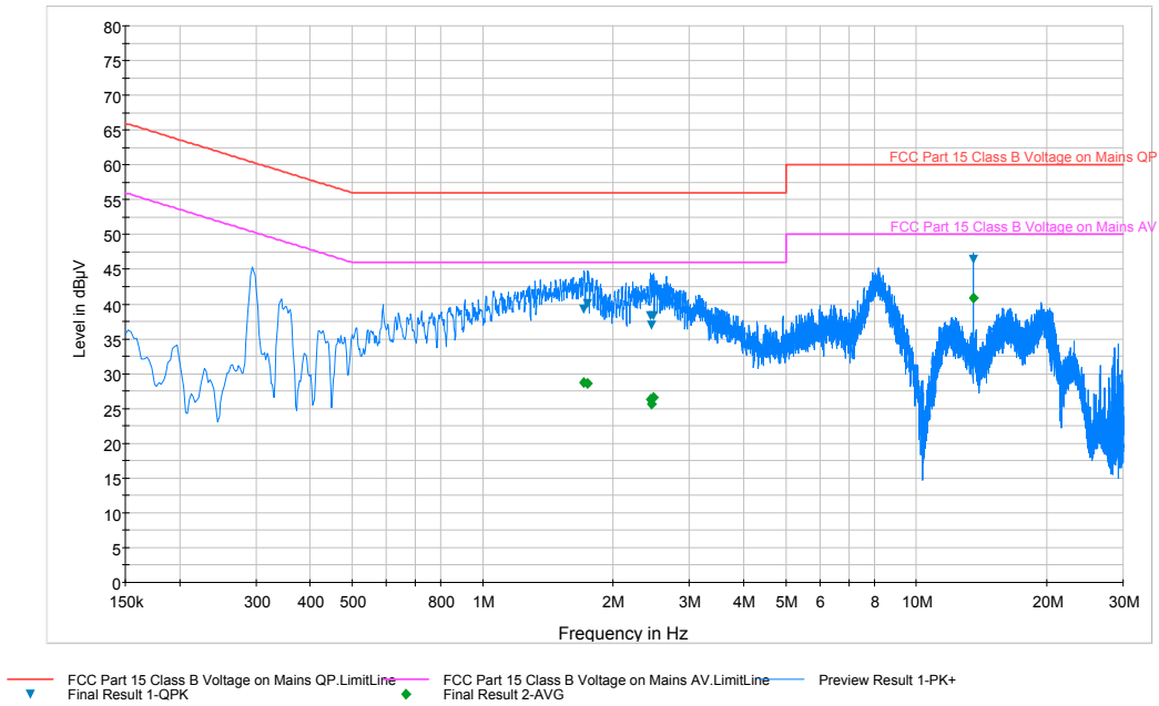
Plot 8-2. Line-Conducted Test Plot (N)
