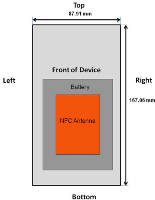
Figure 1-2 NFC Antenna Locations
