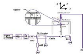
Figure 9-1 System Verification Setup Diagram
