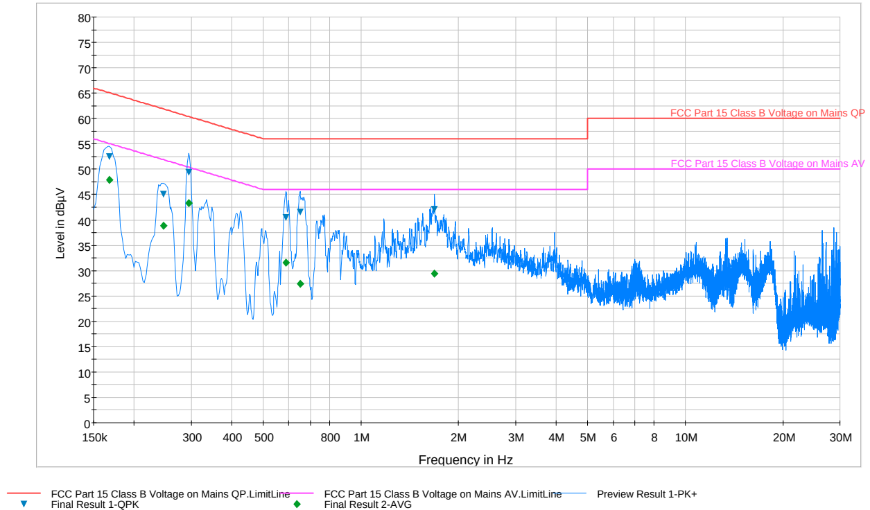
Plot 6-83. Line Conducted Plot with 802.11a UNII Band 2 (L1)
