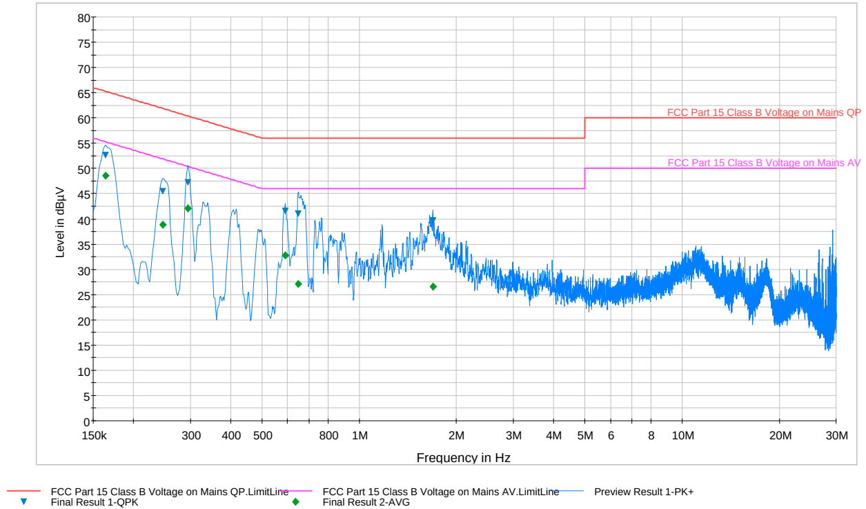
Plot 6-85. Line Conducted Plot with 802.11a UNII Band 3 (L1)
