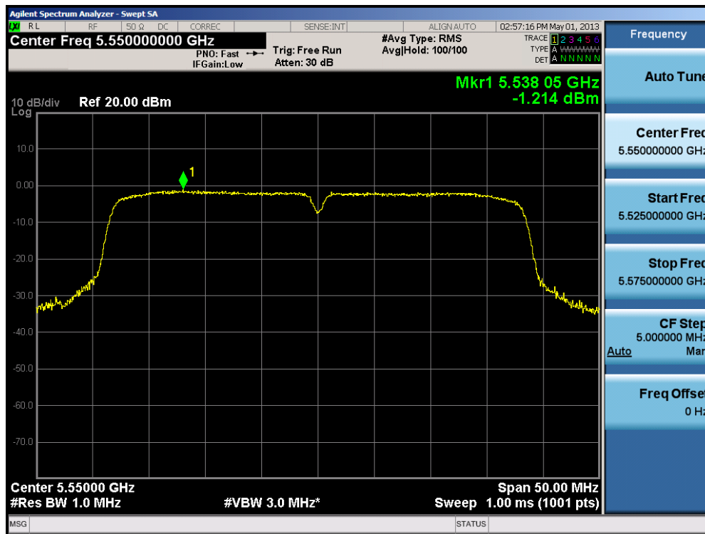
Plot 6-54. Peak Power Spectral Density Plot (40MHz BW 802.11a (UNII Band 3) – Ch. 110)
