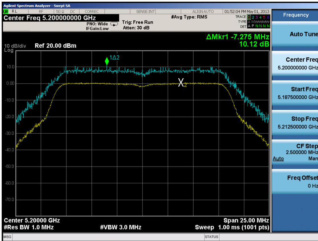
Plot 6-57. Peak Excursion Ratio Plot (802.11a)
