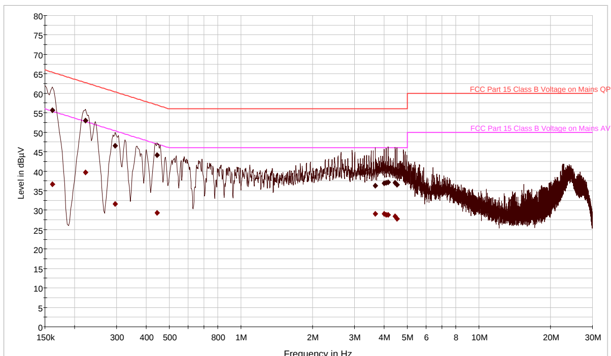
Plot 6-23. Line Conducted Plot with Bluetooth ON (N)
