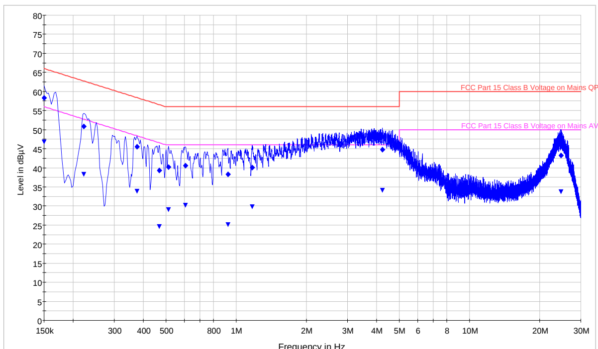
Plot 6-22. Line Conducted Plot with Bluetooth ON (L1)
