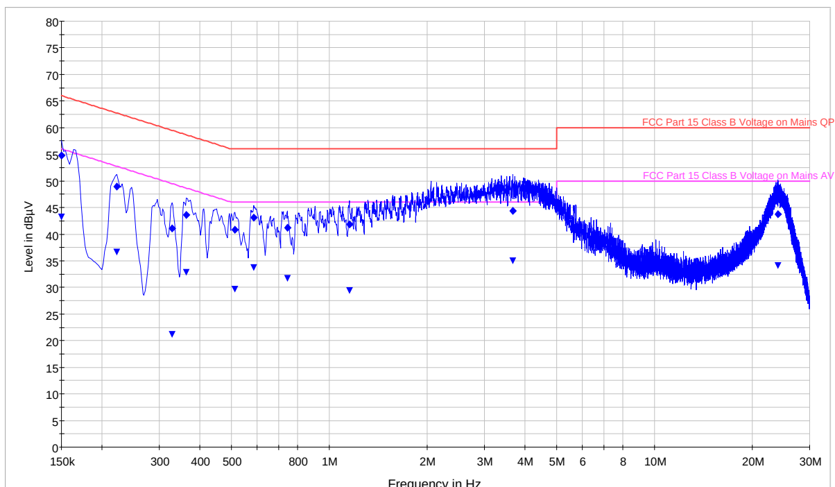
Plot 6-56. Line Conducted Plot with 802.11b (L1)
