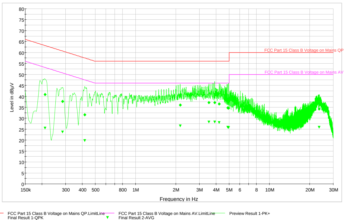
Plot 6-61. Line Conducted Plot with 802.11n (2.4GHz) (N)
