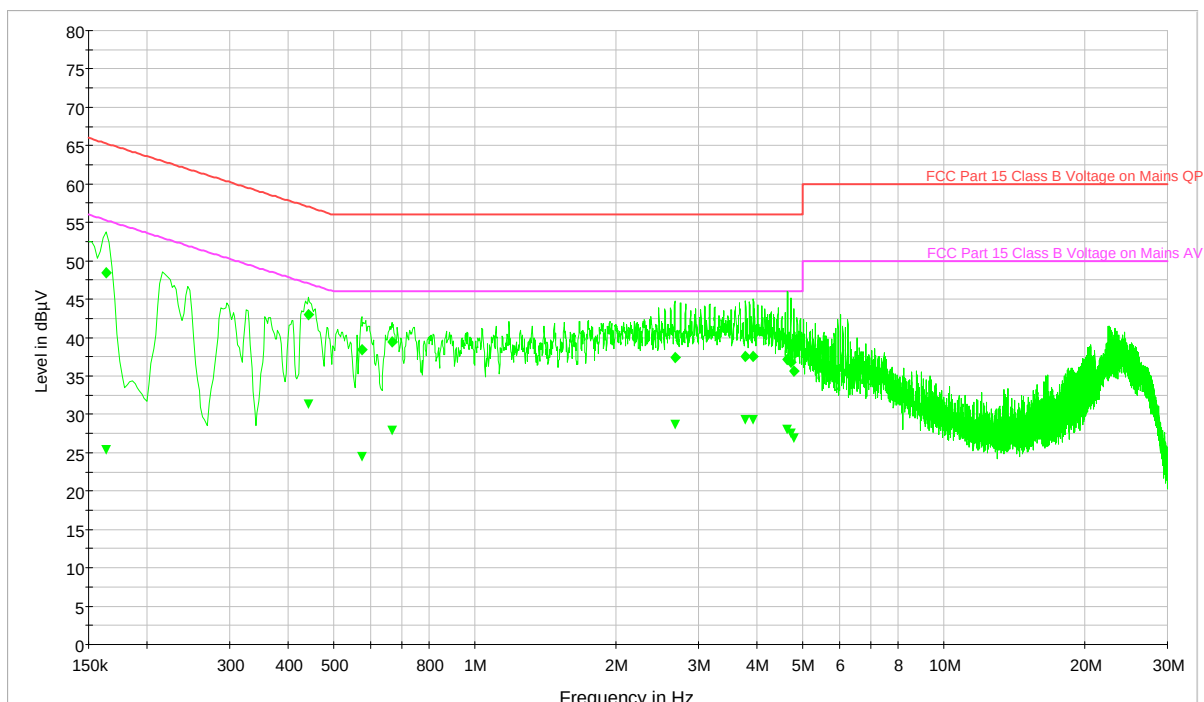
Plot 6-57. Line Conducted Plot with 802.11b (N)
