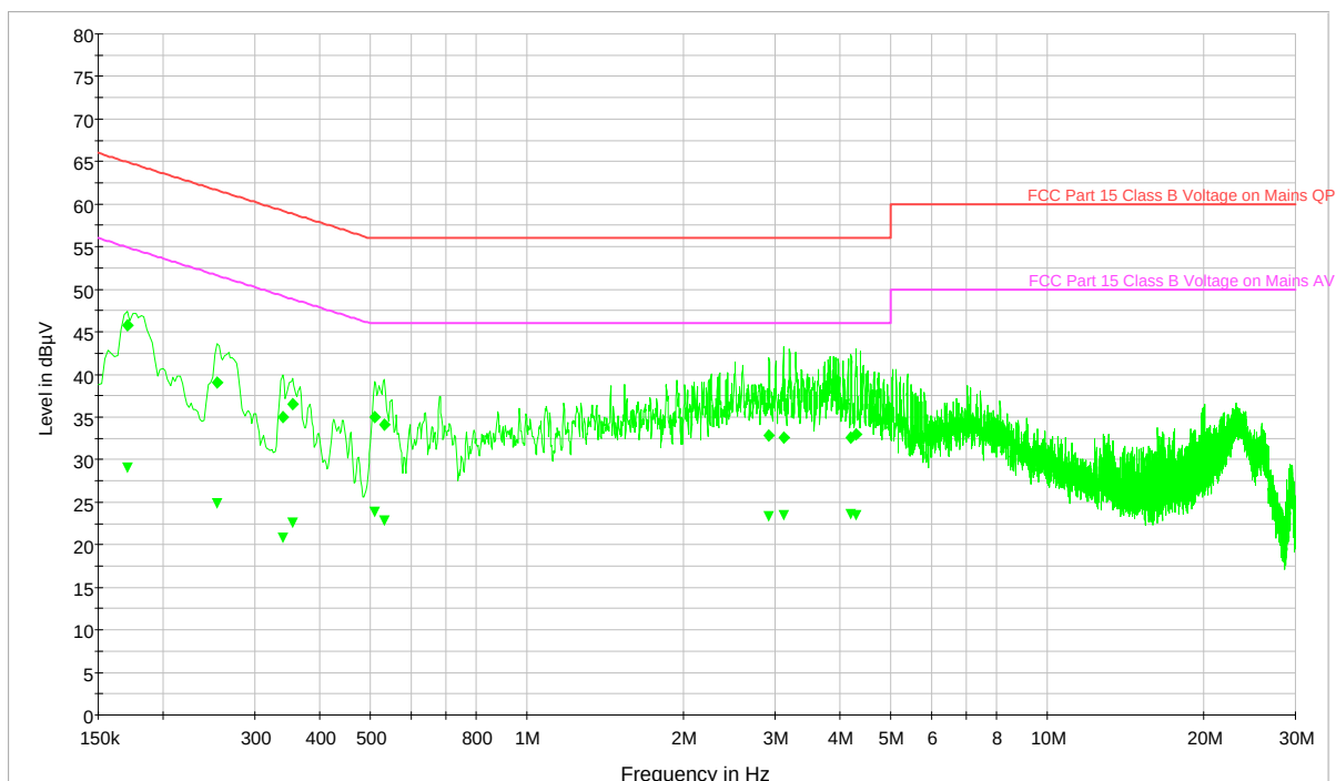
Plot 6-65. Line Conducted Plot with 802.11n (5.8GHz) (N)
