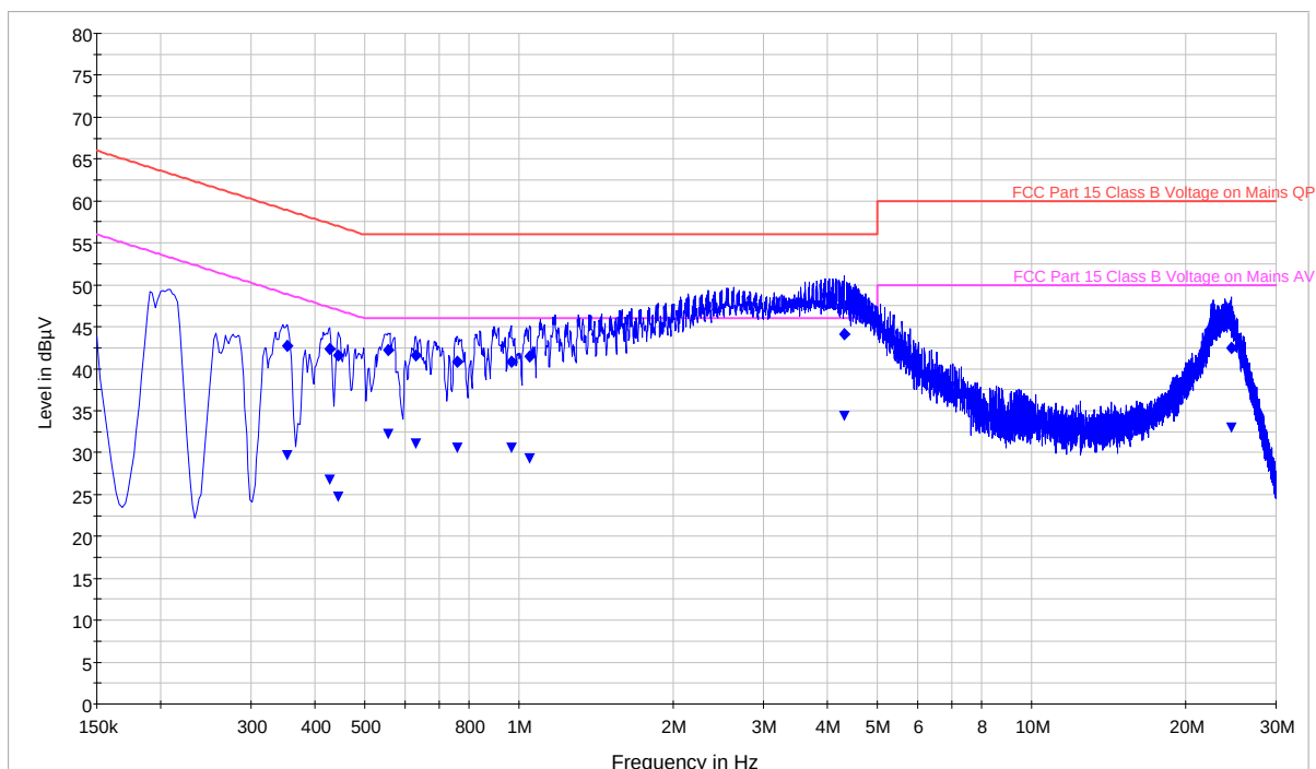
Plot 6-58. Line Conducted Plot with 802.11g (L1)
