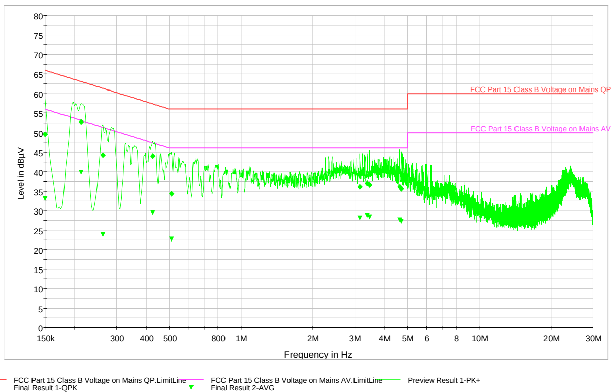
Plot 6-59. Line Conducted Plot with 802.11g (N)
