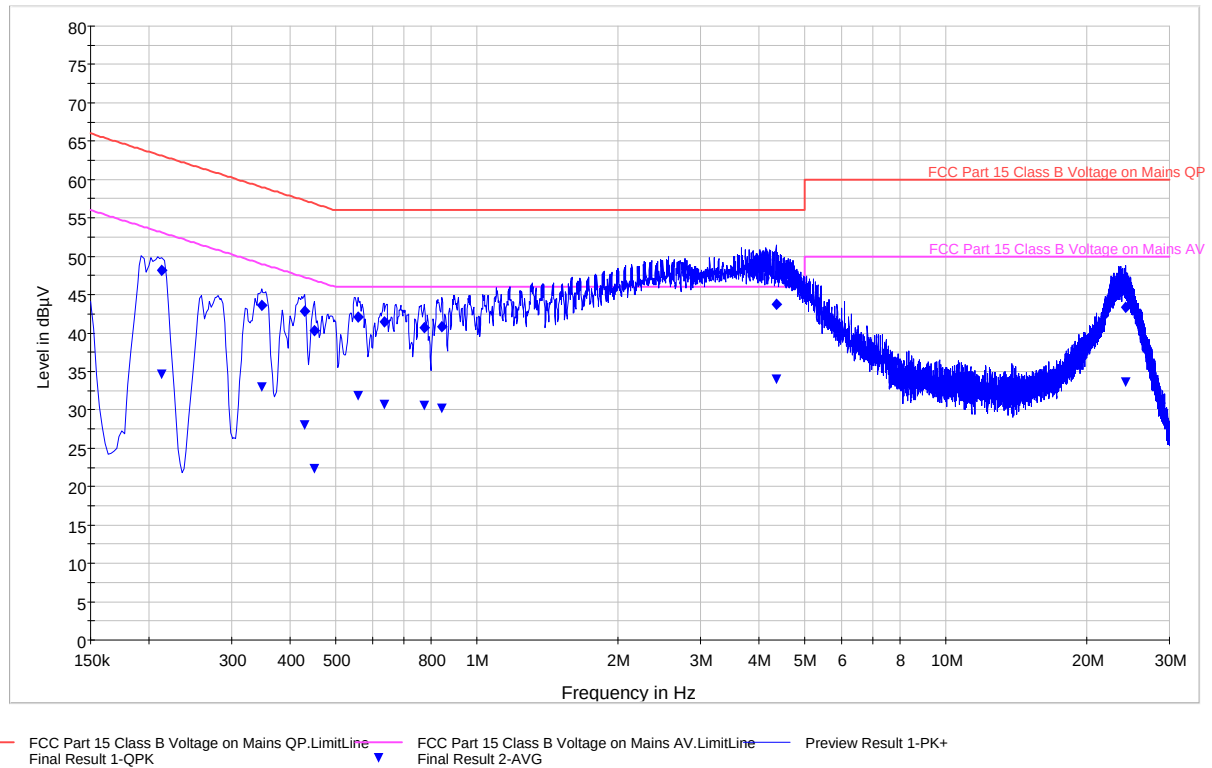
Plot 6-60. Line Conducted Plot with 802.11n (2.4GHz) (L1)
