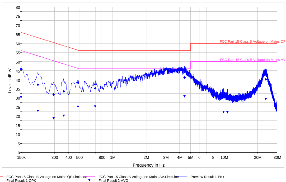
Plot 6-64. Line Conducted Plot with 802.11n (5.8GHz) (L1)
