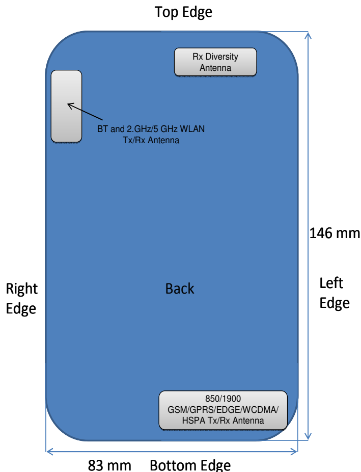
Figure 13-1 Identification of Sides for SAR Testing
