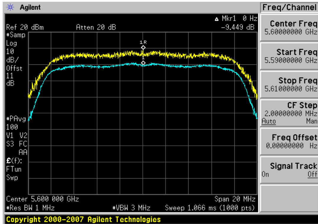
Plot 6-50. Peak Excursion Ratio Plot (802.11a (UNII Band 3) – Ch. 120)
