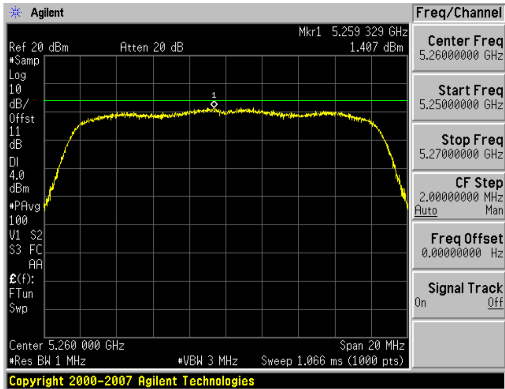
Plot 6-25. Peak Power Spectral Density Plot (802.11a (UNII Band 2) – Ch. 52)
