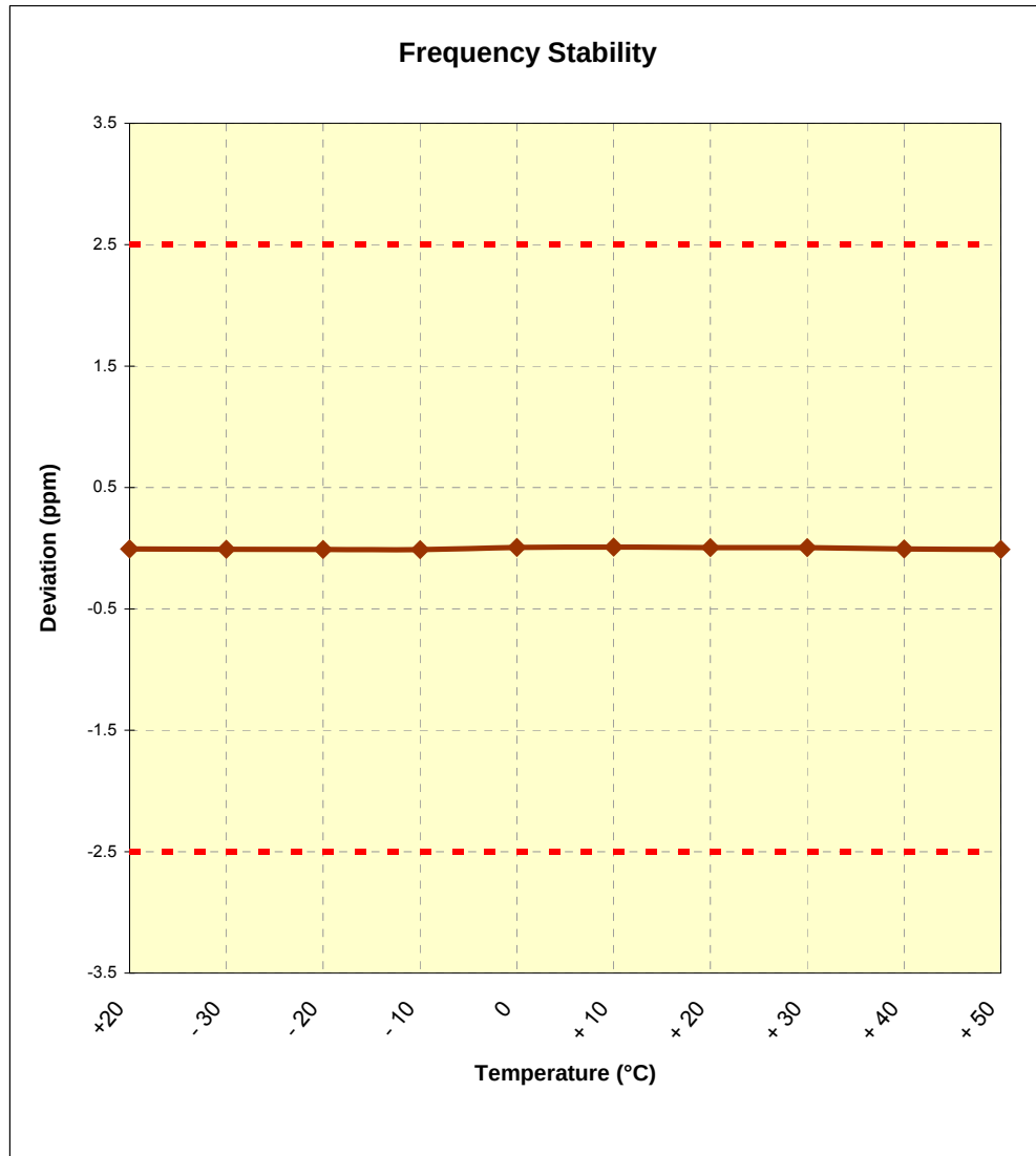
Figure 6-1. Frequency Stability Graph (AWS WCDMA Mode – Ch. 1412)
