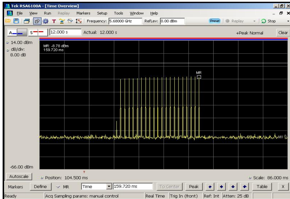
Figure 6-1. Type 1 Radar Pulse
