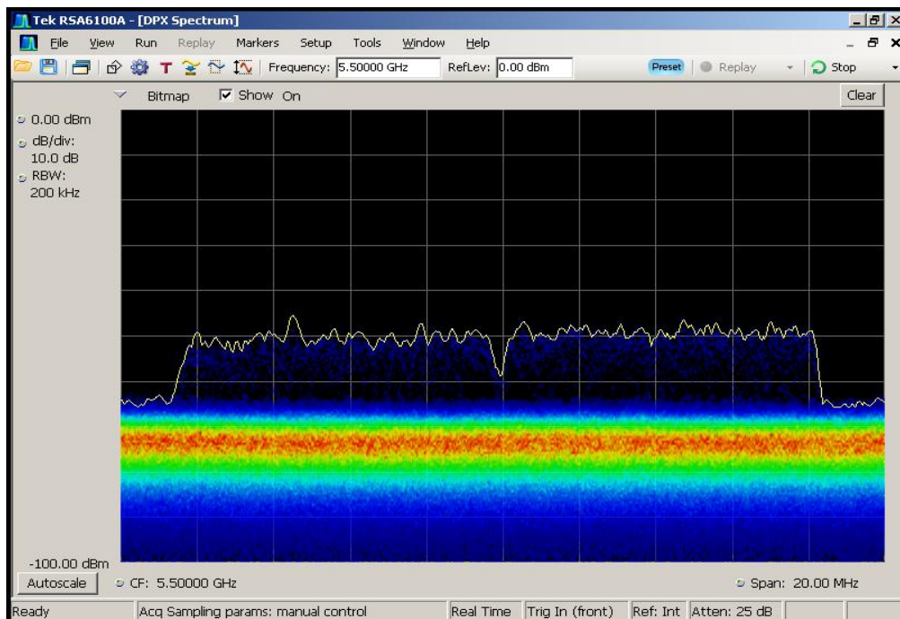
Figure 6-2. Real-Time Spectrum Display, No WLAN Traffic
