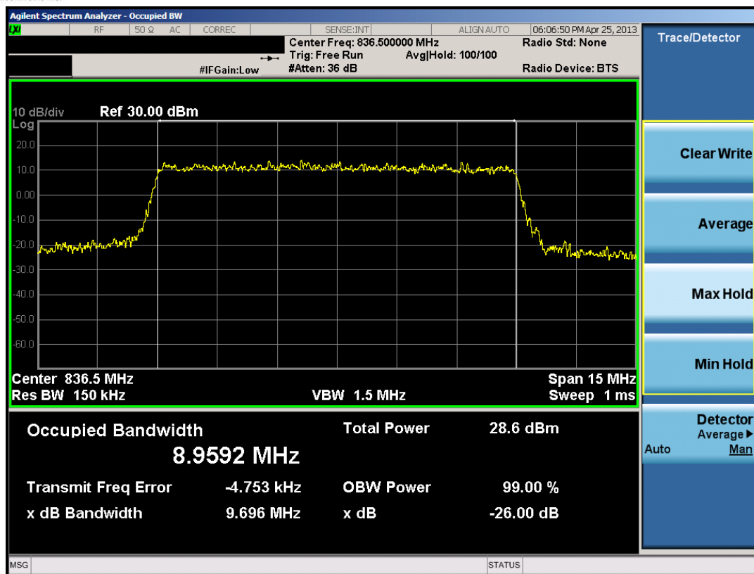
Plot 7-40. Occupied Bandwidth Plot (10.0MHz 16-QAM – RB Size 50)
