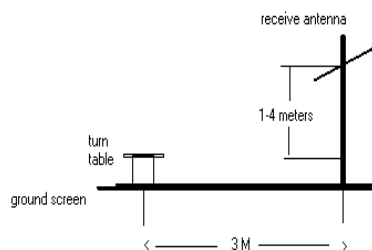
Figure 3-1. Diagram of 3-meter Test Range
