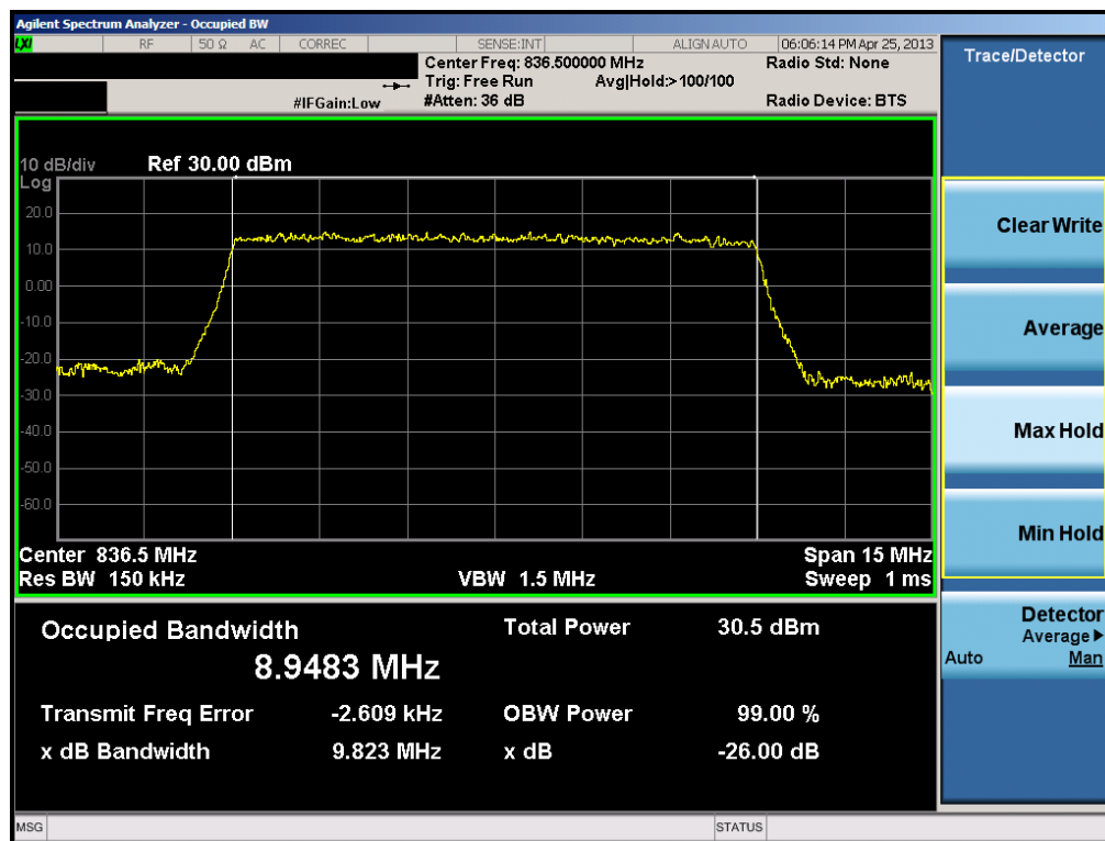
Plot 7-39. Occupied Bandwidth Plot (10.0MHz QPSK – RB Size 50)
