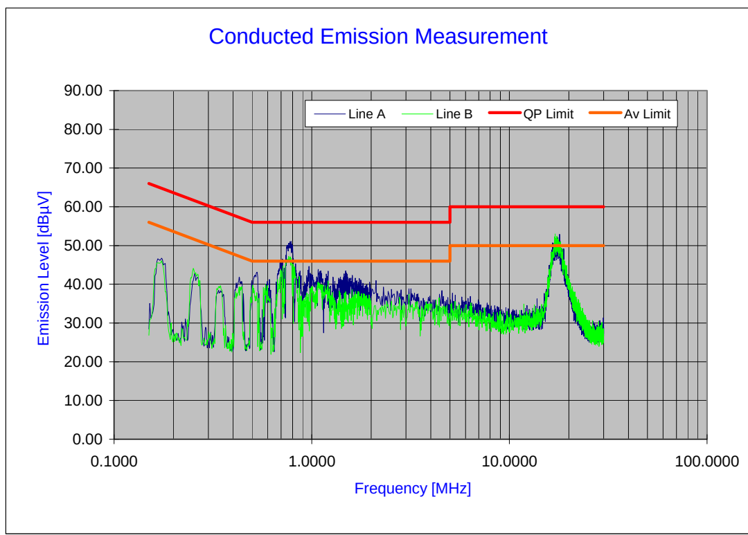
Plot 6-63. Line Conducted Plot with 802.11a UNII Band 3 (L1)
