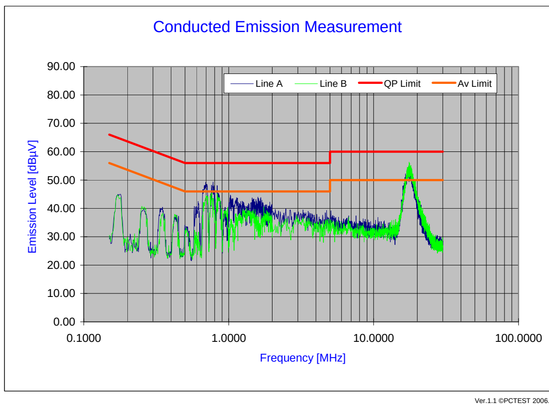
Plot 6-61. Line Conducted Plot with 802.11a UNII Band 1
