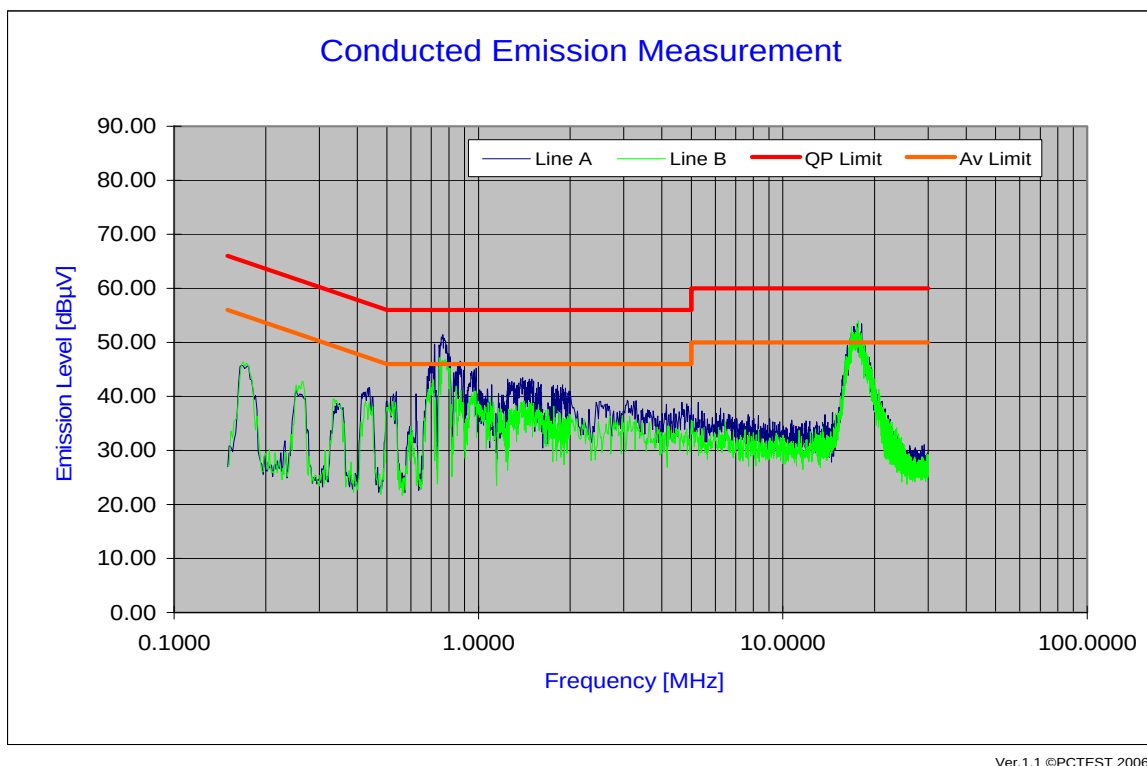
Plot 6-62. Line Conducted Plot with 802.11a UNII Band 2 (L1)
