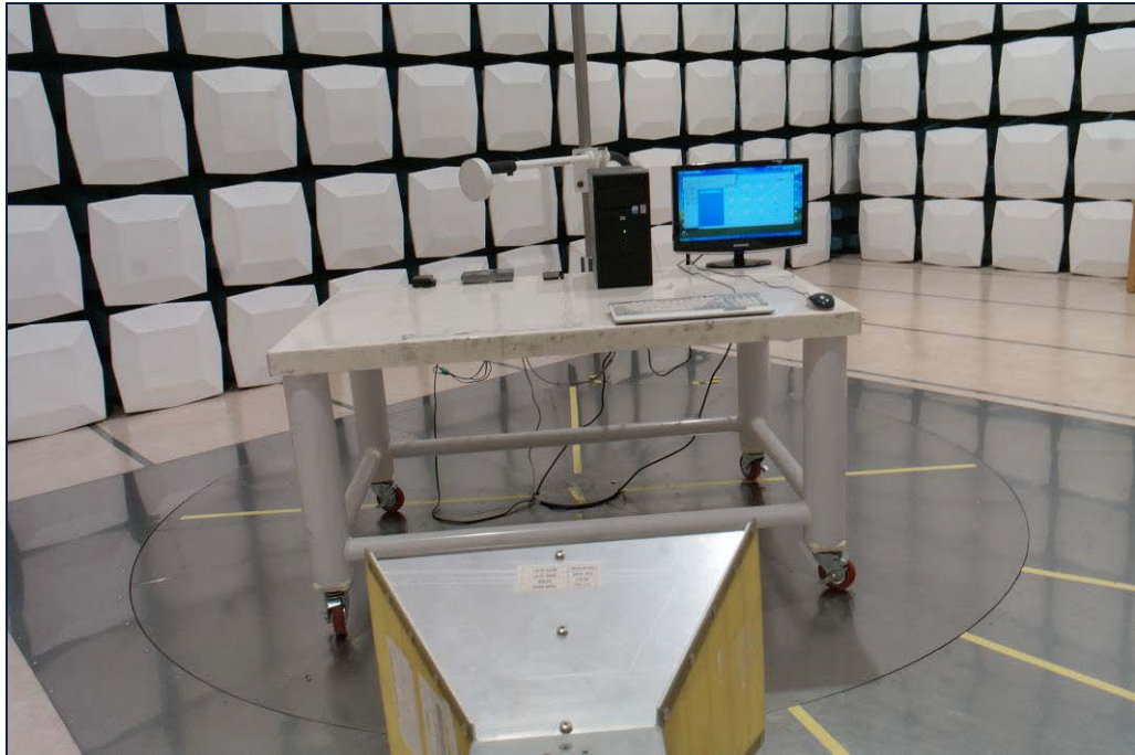
[ Radiated Disturbance for Above 1 GHz – Front ]
