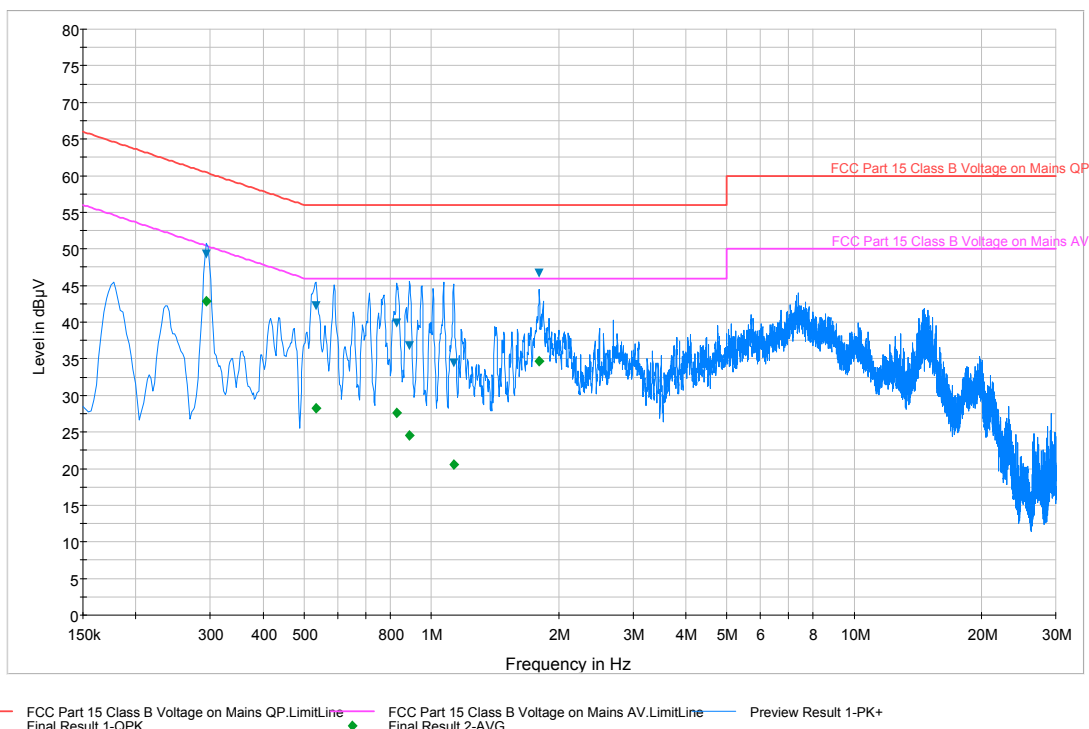
Plot 6-21. Line Conducted Plot with Bluetooth LE (N)
