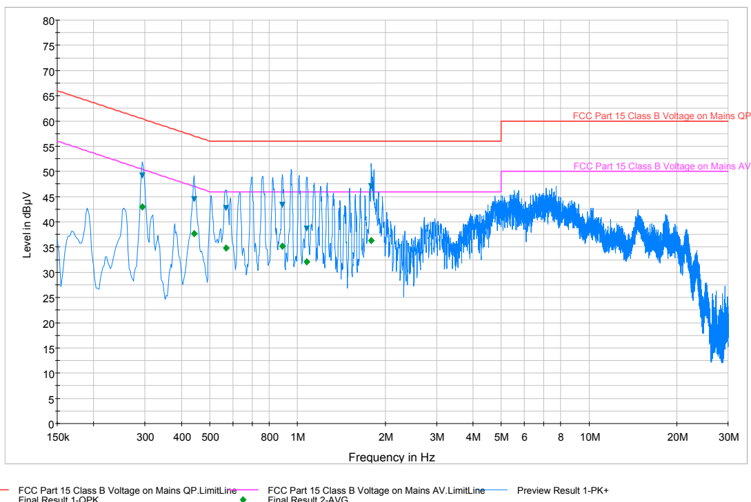
Plot 6-20. Line Conducted Plot with Bluetooth LE (L1)
