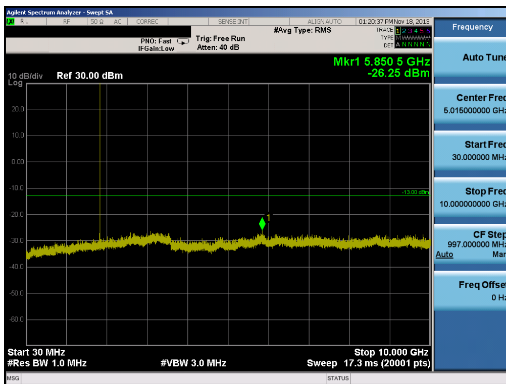
Plot 6-16. Conducted Spurious Plot (PCS GSM Mode – Ch. 512)
