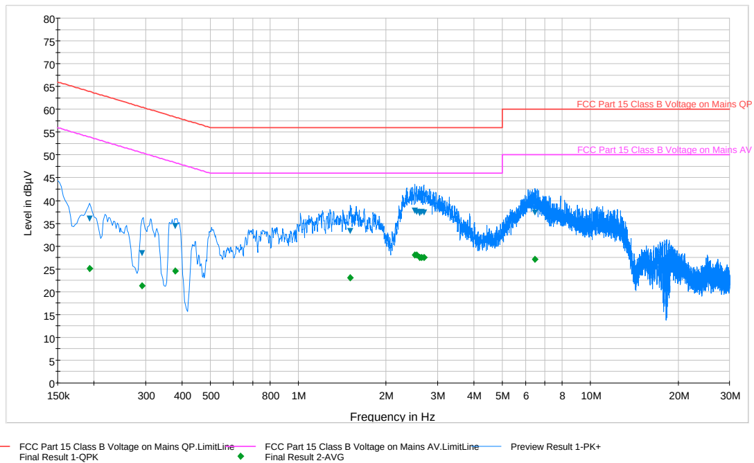
Plot 6-24. Line-Conducted Test Plot (L1)
