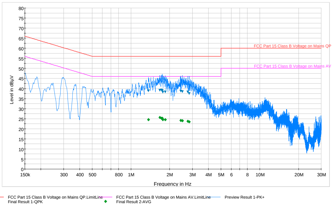
Plot 6-25. Line-Conducted Test Plot (N)
