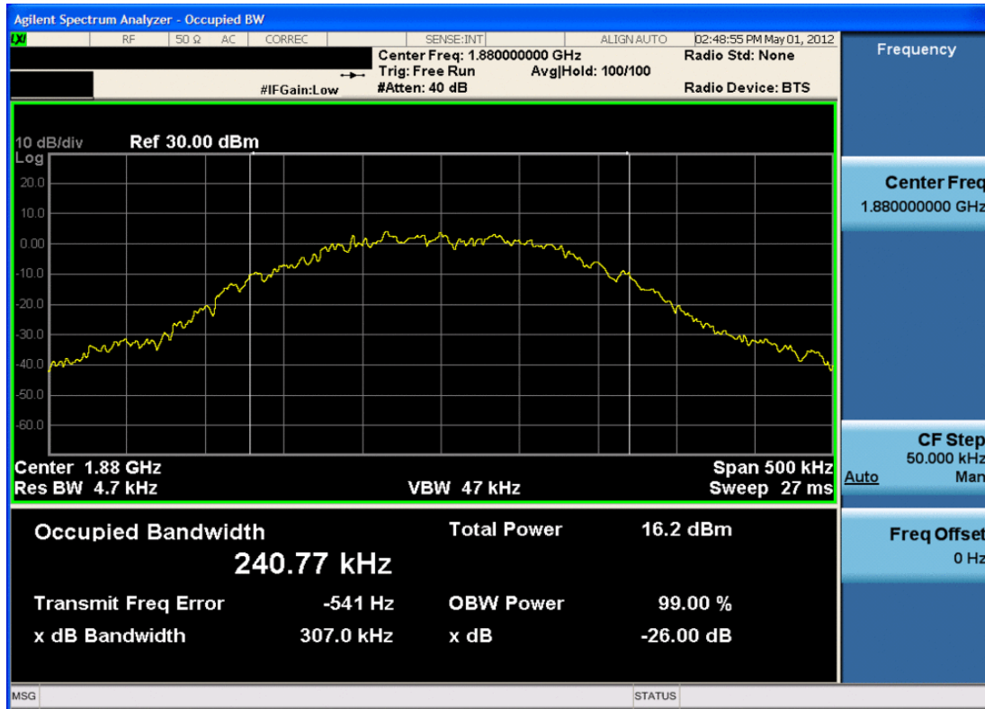
Plot 7-11. Occupied Bandwidth Plot (EDGE1900 Mode – Ch. 661)
