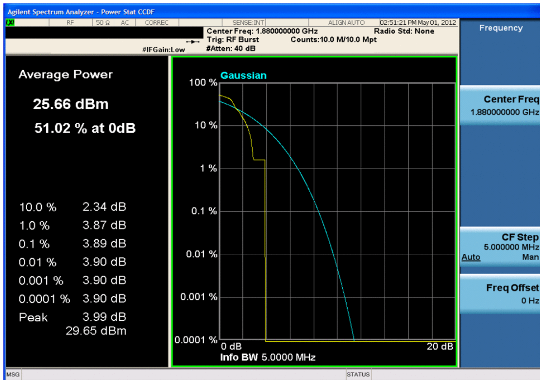
Plot 7-12. Peak-Average Ratio Plot (EDGE1900 Mode – Ch. 661)
